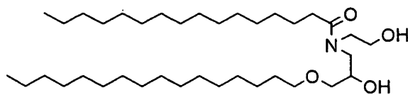
Amphipathic amide lipid B
