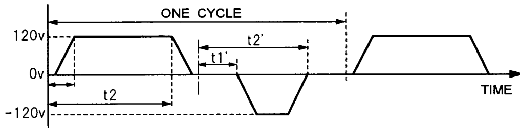
FIG. 7A VOLTAGE WAVEFORM OF SUSTAIN PULSE SIGNAL FOR X ELECTRODE
