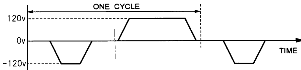
FIG. 7B VOLTAGE WAVEFORM OF SUSTAIN PULSE SIGNAL FOR Y ELECTRODE
