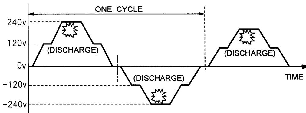
FIG. 7C VOLTAGE WAVEFORM OF (X - Y)
