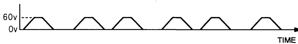
FIG. 7D VOLTAGE WAVEFORM OF (X + Y) / 2
