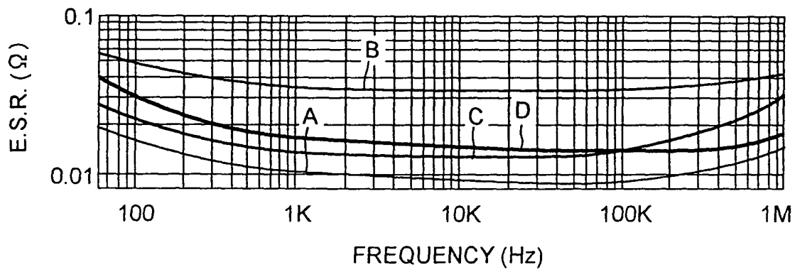
FREQUENCY VS. E.S.R. CHARACTERISTIC OF ELECTROLYTIC CAPACITORS OF 63V /2200 \mu F
