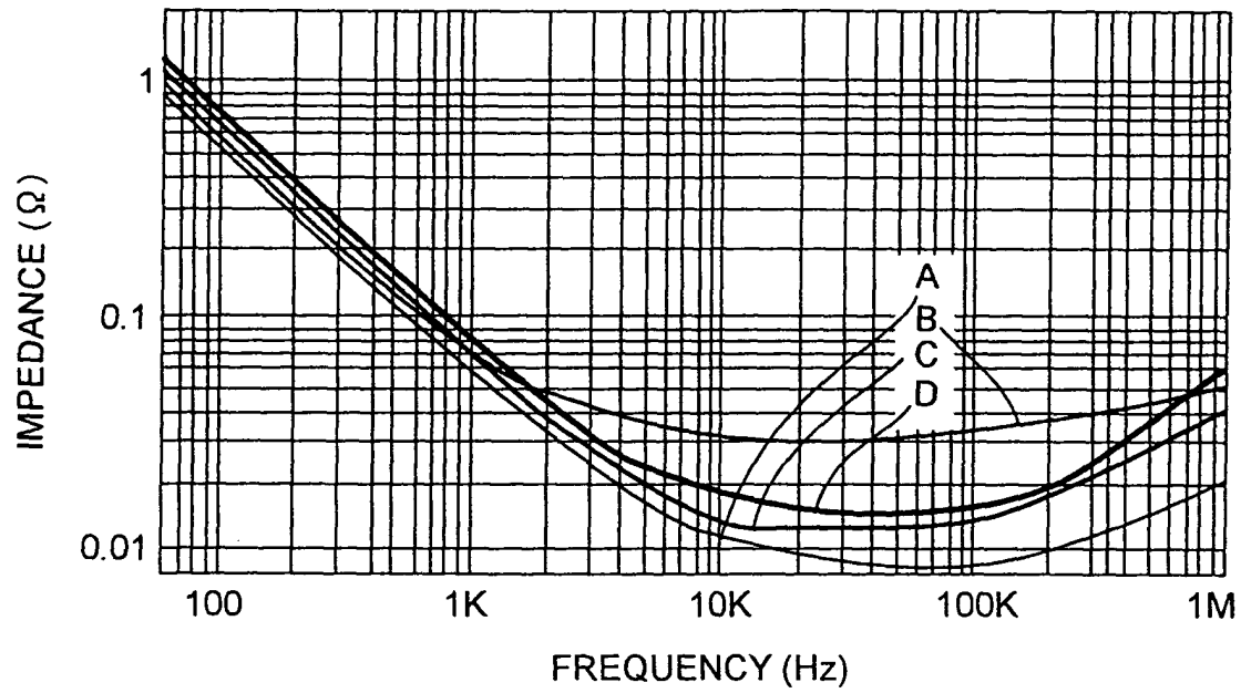
FREQUENCY VS. IMPEDANCE CHARACTERISTIC OF ELECTROLYTIC CAPACITORS OF 63V /2200 \mu F
