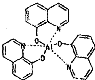
Chemical Formula 2
