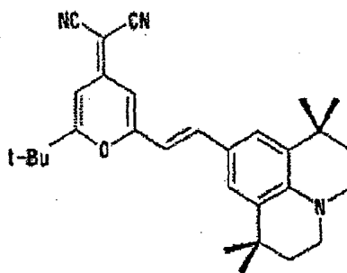
Chemical Formula 3
