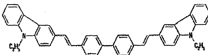
Chemical Formula 5
