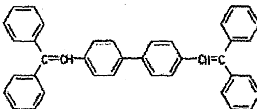
Chemical Formula 4
