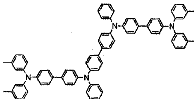
Chemical Formula 1
