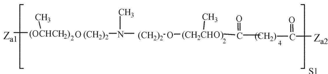
Backbone oligoester 1
