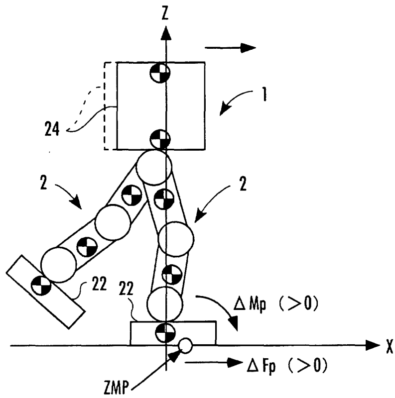
FIG.8 ( BODY TRANSLATION MODE )
