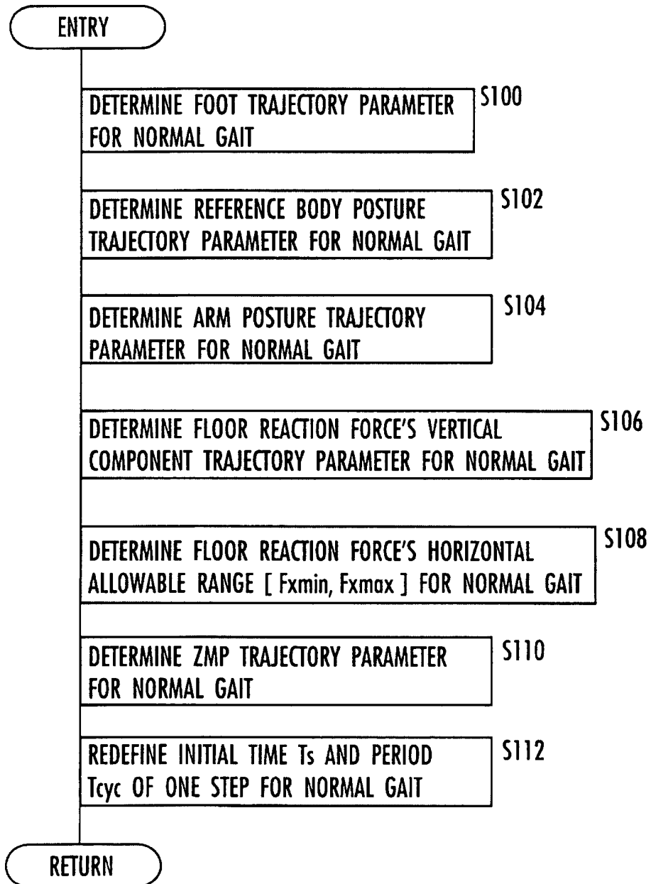
FIG.14 ( PROCESS OF DETERMINING NORMAL GAIT PARAMETER )
