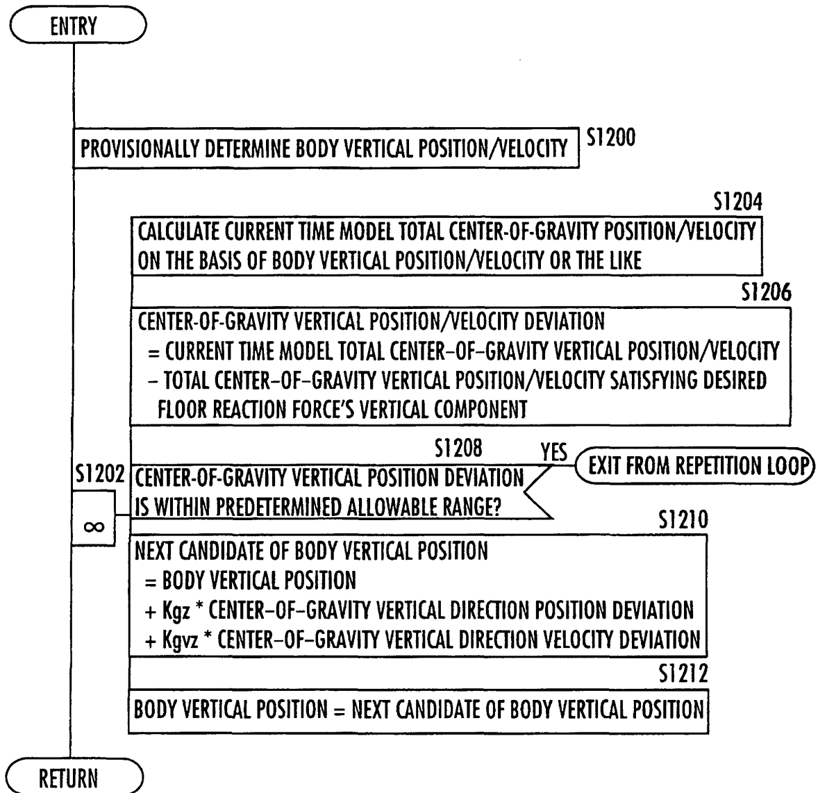
FIG.47 ( BODY VERTICAL POSITION DETERMINATION PROCESS: METHOD 2 )
