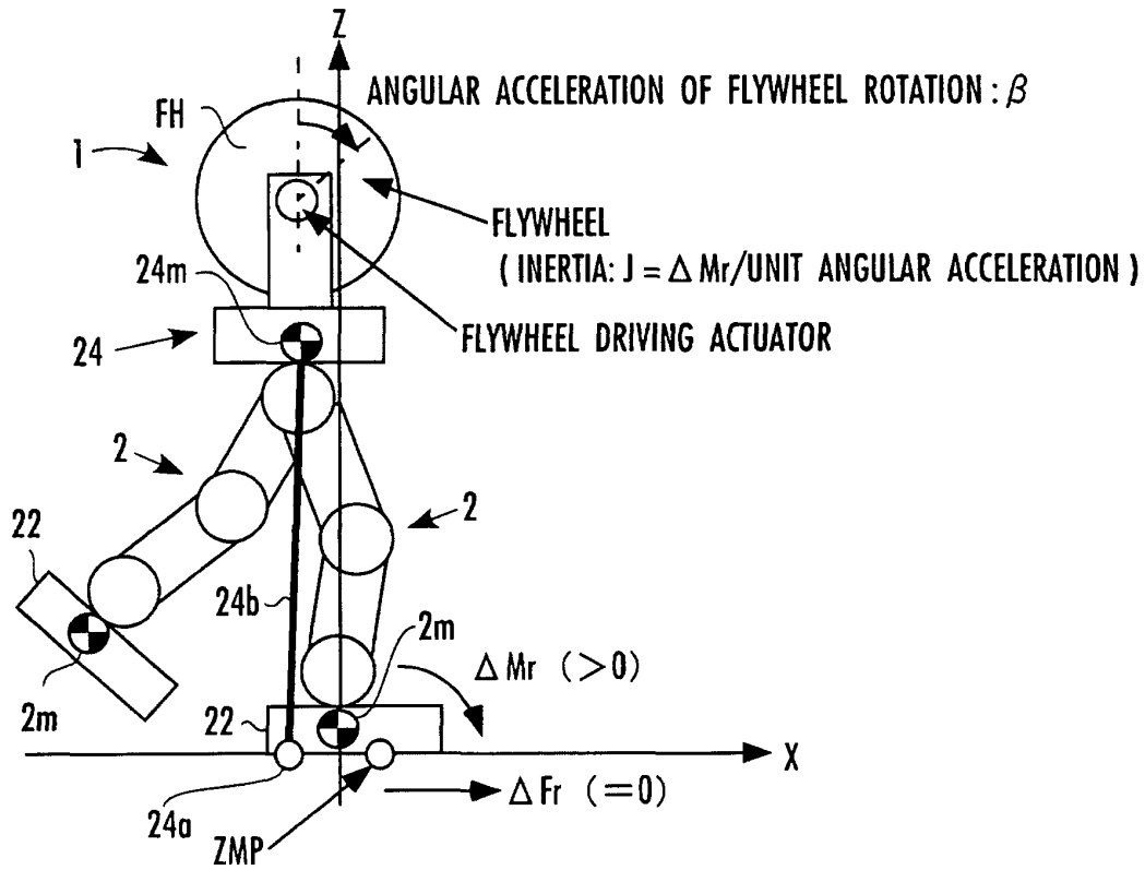
FIG.10 ( MODEL WITH FLYWHEEL )
