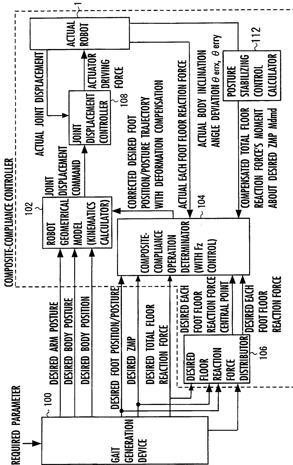
FIG.4 ( FUNCTIONAL BLOCK DIAGRAM OF LEGGED MOBILE ROBOT )
