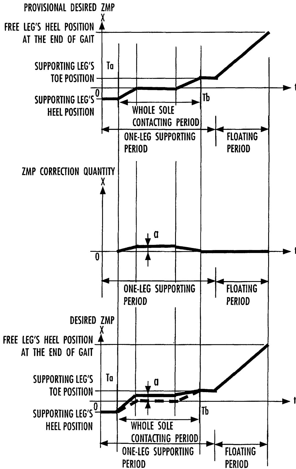
FIG.38 ( CORRECTION OF DESIRED ZMP )
