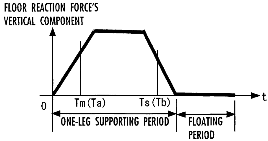
FIG.6 ( DESIRED FLOOR REACTION FORCE'S VERTICAL COMPONENT )
