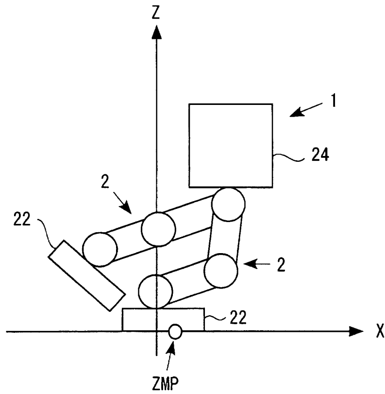
FIG.13 ( DIVERGENCE STATE OF BODY POSITION )
