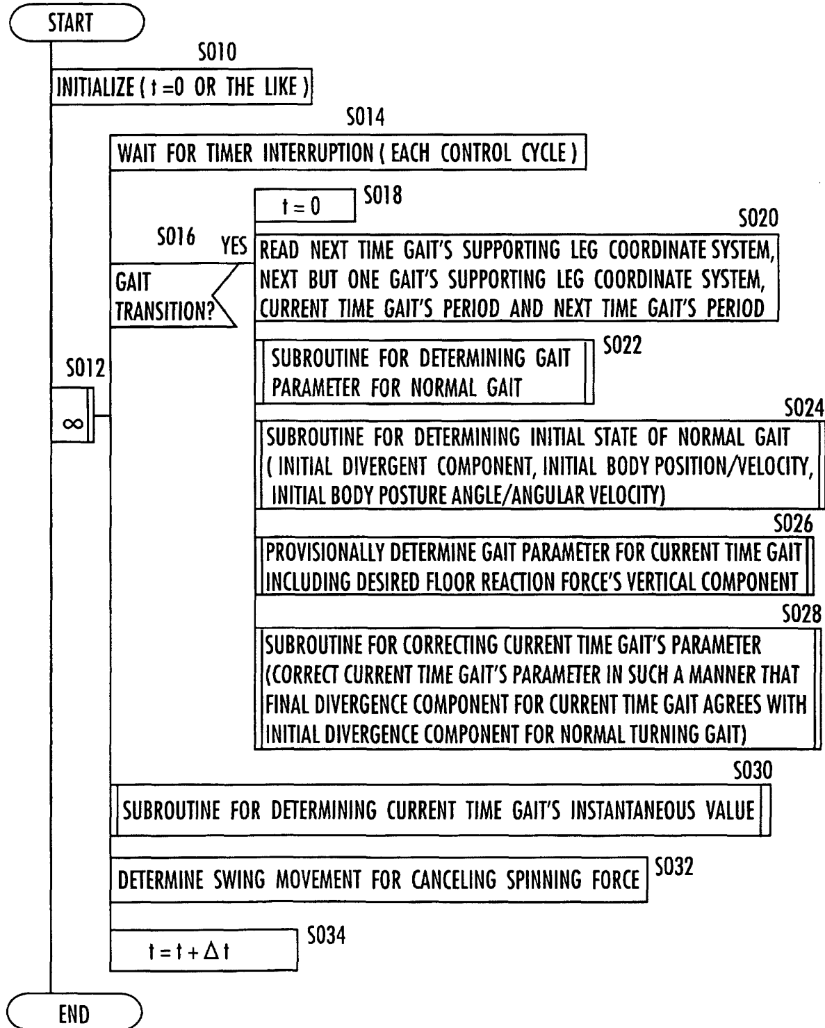
FIG.12 (FLOWCHART OF GAIT GENERATION PROCESS)
