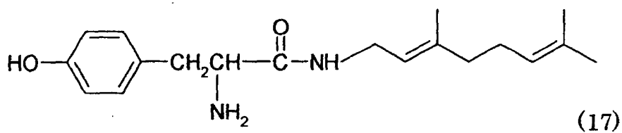
N-acetyltyrosine geranylamide
