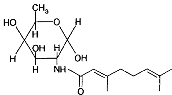
and N-fucosegeranamide
