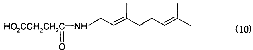
N,N'-digeranylsuccinic diamide
