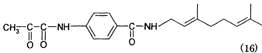
tyrosine geranylamide
