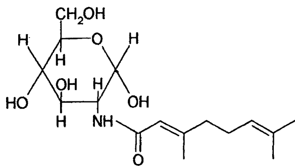
N-glucosylgeranamide
