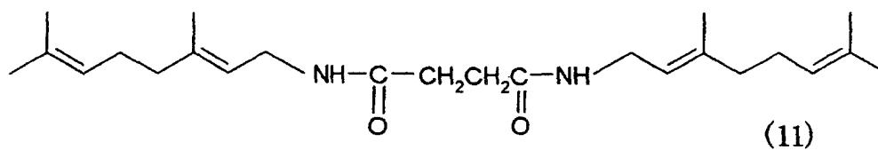
N,N'-digeranylfumaric diamide
