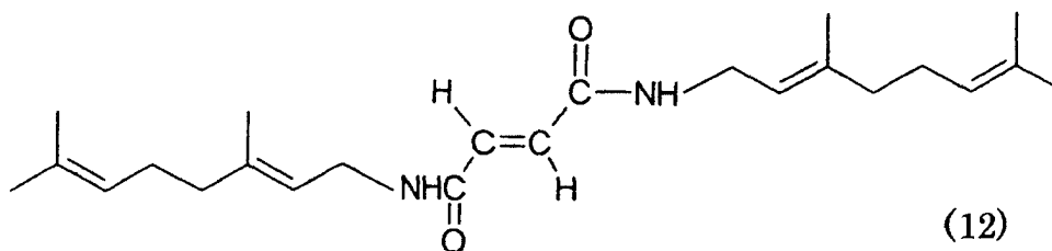
N-geranylfumaric monoamide
