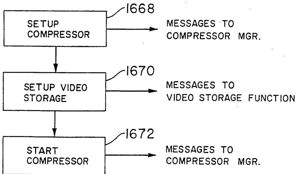
FIG. 72 VIDEO RECORD FUNCTION
