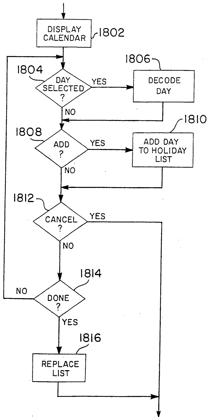
FIG. 80 SCHEDULING: HOLIDAY SETUP
