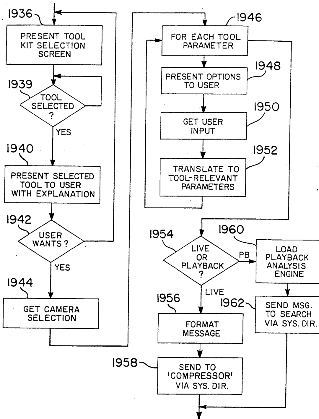
FIG. 89 SELECT & SETUP ANALYSIS TOOL
