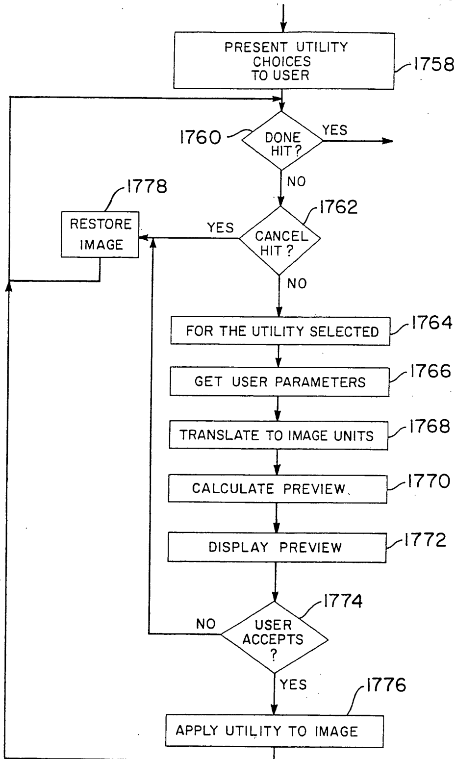
FIG. 77 IMAGE PROCESSING UTILITIES MGR.
