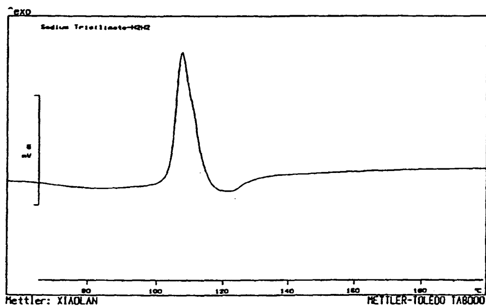
DSC of sodium trisilicate peroxide complex (\text{Na}_2\text{Si}_3\text{O}_7 \cdot 0.68\text{H}_2\text{O}_2) under the atmosphere condition
