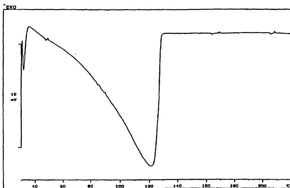
DSC of calcium pyrophosphate peroxide complex ( \text{Ca}_2\text{P}_2\text{O}_7 \cdot 3.42\text{H}_2\text{O}_2 ) under the atmosphere condition
