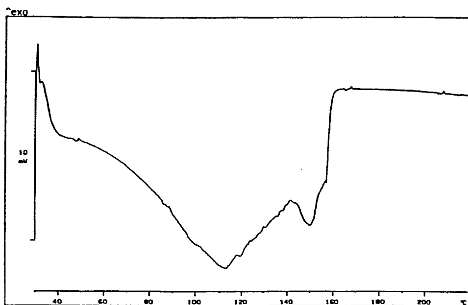
DSC of potassium sulfate peroxide complex ( \text{K}_2\text{SO}_4 \cdot 0.62\text{H}_2\text{O}_2 ) under the atmosphere condition
