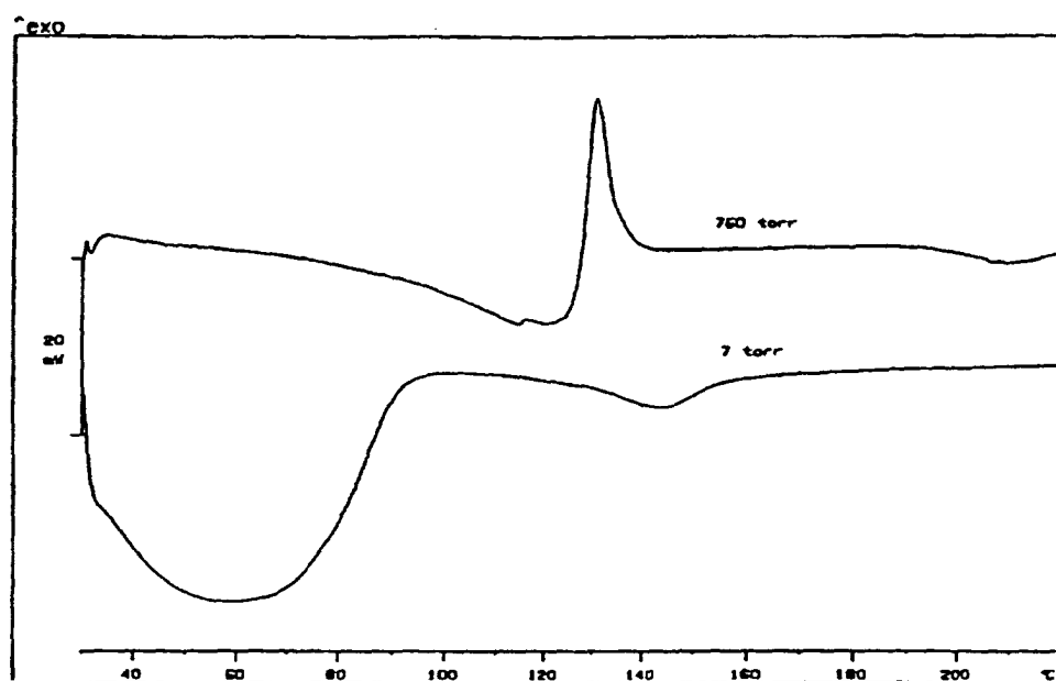
DSC of magnesium pyrophosphate peroxide complex ( \text{Mg}_2\text{P}_2\text{O}_7 \cdot 4.60\text{H}_2\text{O}_2 ) at 760 torr and 7 torr.
