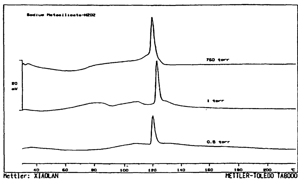
DSC of Sodium metasilicate peroxide complex (Na 2 SiO 3 ·2.15H 2 O 2 ) under the atmosphere (760 torr) and vacuum (1 torr and 0.5 torr) conditions
