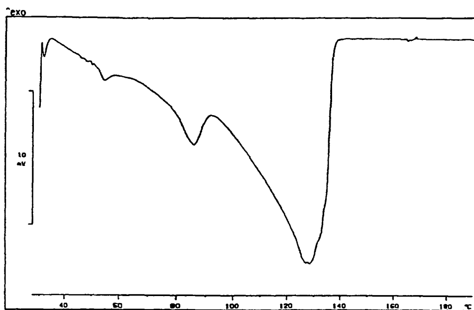
DSC of sodium sulfate peroxide complex ( \text{Na}_2\text{SO}_4 \cdot 1.28\text{H}_2\text{O}_2 ) under the atmosphere condition
