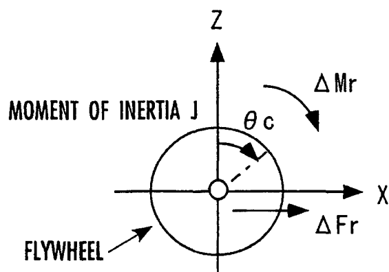
FIG.44 ( PERTURBATION MODEL FOR CORRECTING BODY POSTURE ANGLES )
