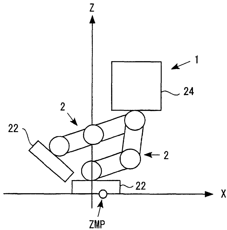
FIG.14 ( DIVERGENCE STATE OF BODY POSITION )
