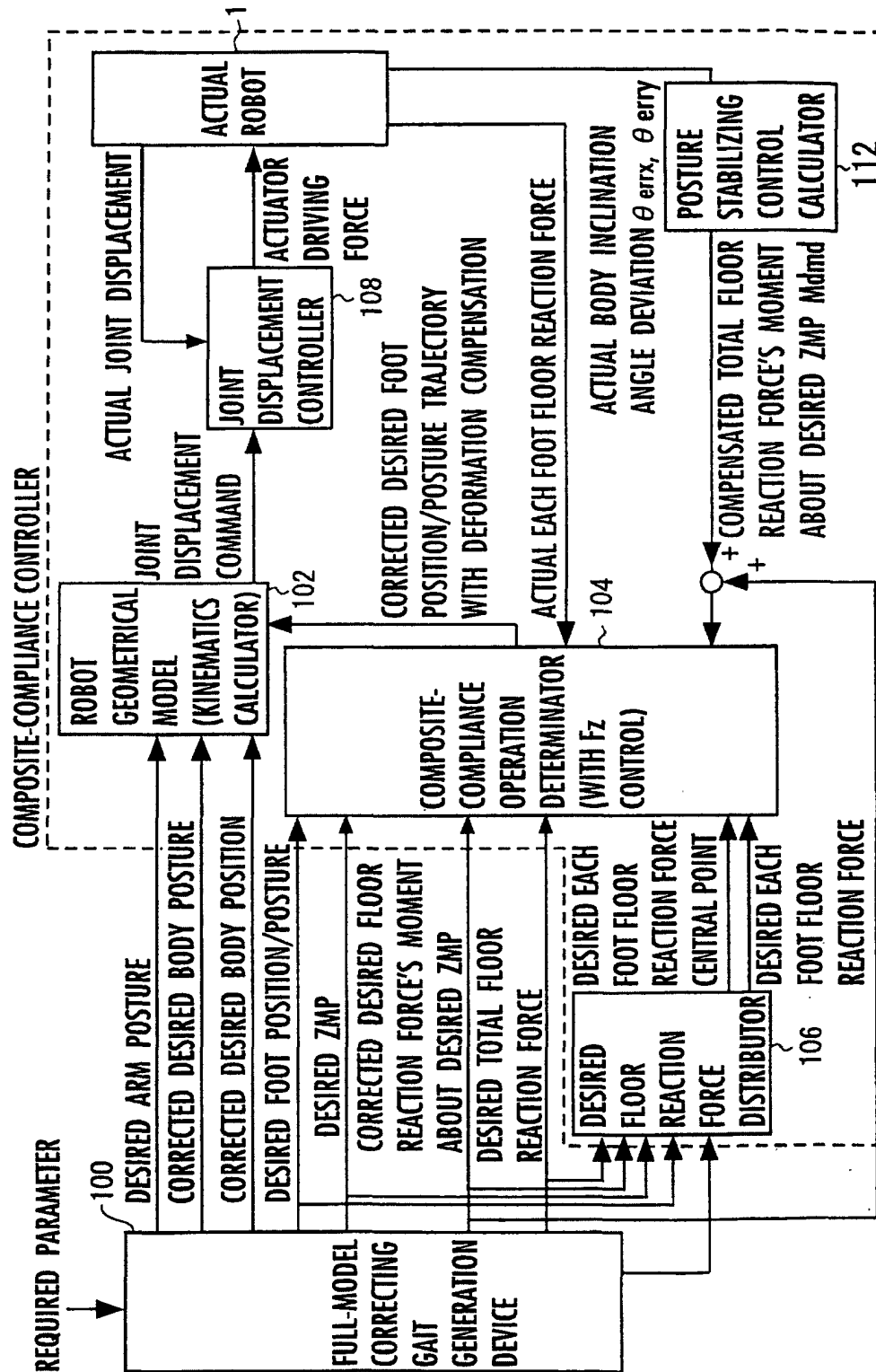
FIG.4 ( FUNCTIONAL BLOCK DIAGRAM OF CONTROL UNIT )
