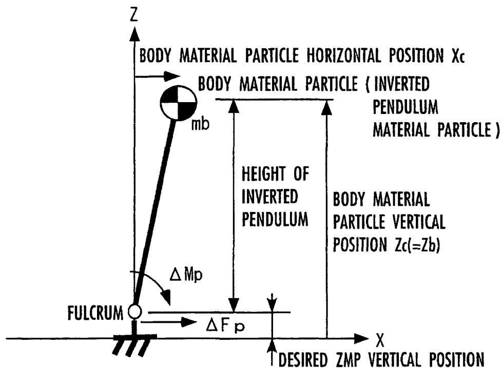
FIG.43 ( PERTURBATION MODEL FOR CORRECTING BODY HORIZONTAL POSITIONS )
