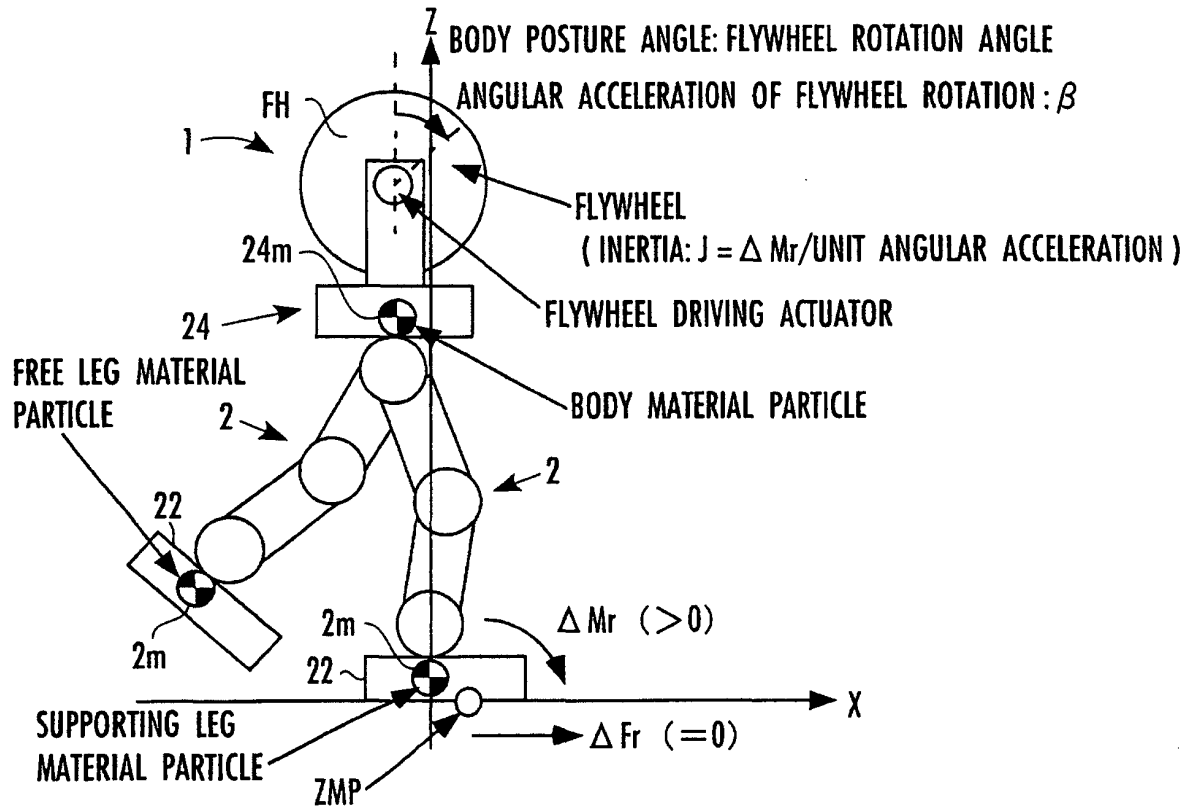
FIG.11 (SIMPLIFIED MODEL WITH FLYWHEEL)
