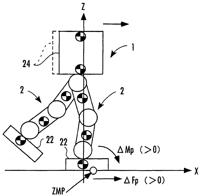
FIG.9 ( BODY TRANSLATION MODE )
