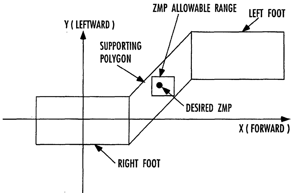
FIG.45 ( SUPPORTING POLYGON AND ZMP ALLOWABLE RANGE )
