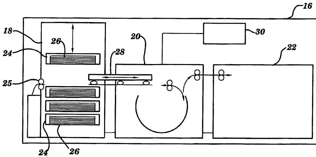
FIG. 3 (PRIOR ART)
