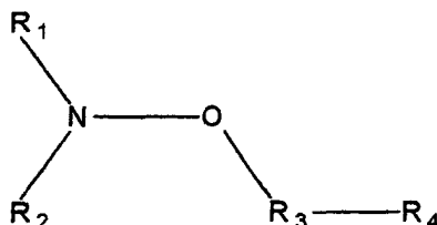
Generic Nitroxyl Ether Structure
