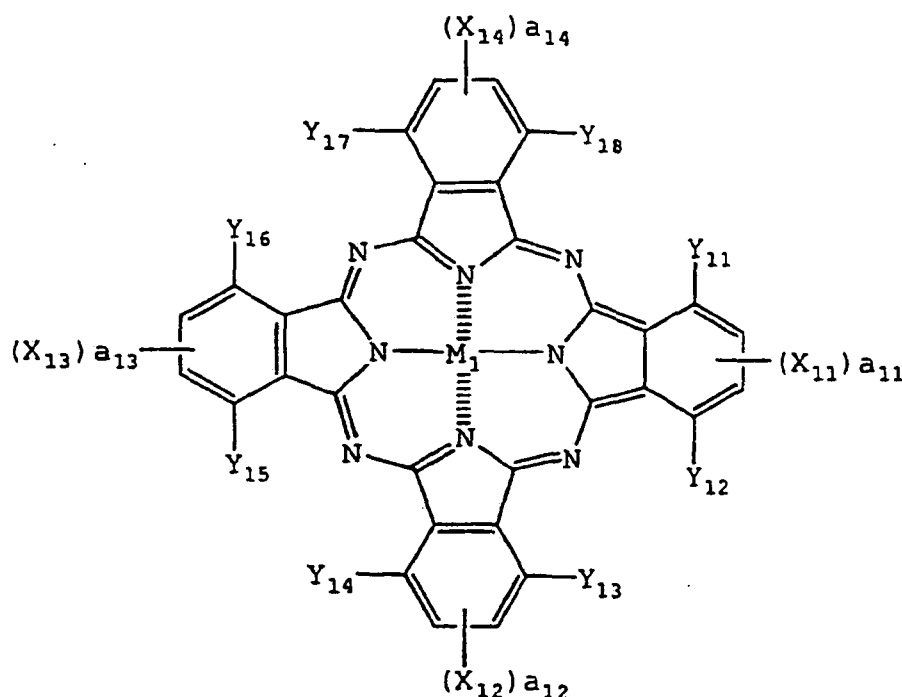
Formel (II)
