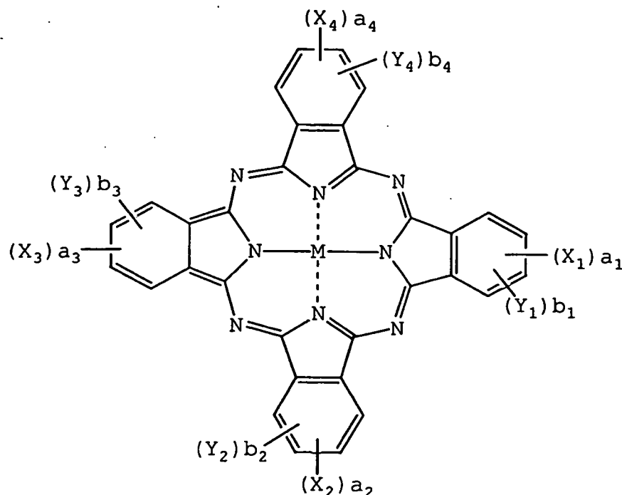
Formula (I):
