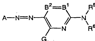
General formula (1)
