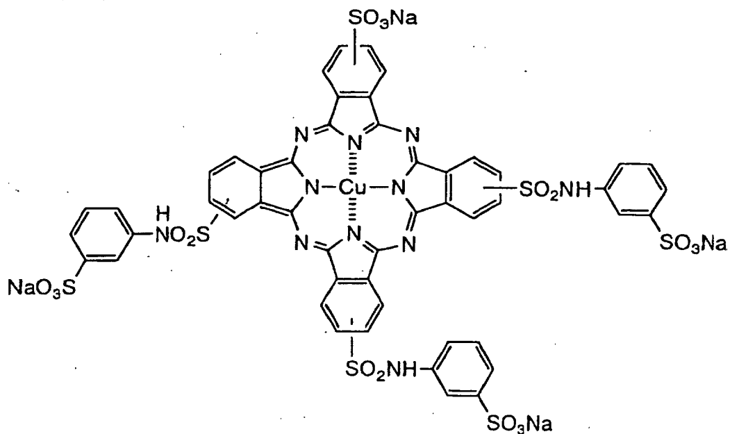
(I-2)
