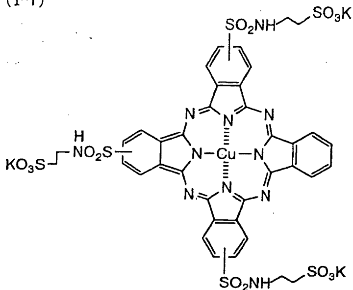
(I-1)
