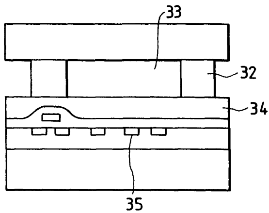
FIG. 3 PRIOR ART
