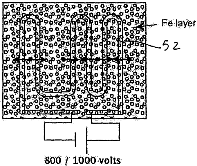
Fig 18: Simple coil configuration to direct a vehicle:
