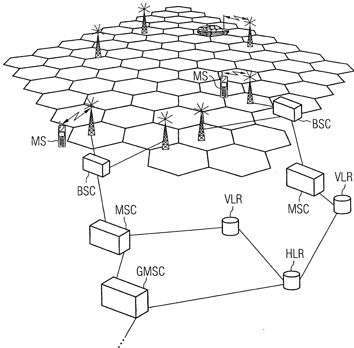
FIG. 11 Prior Art
