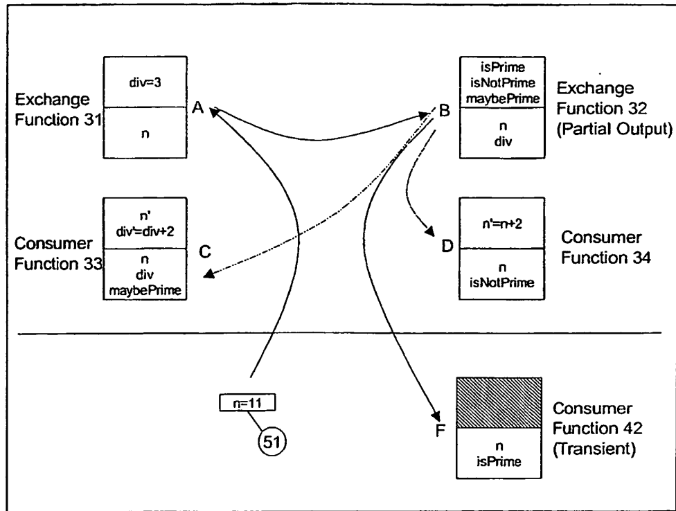
Figure 7 - Prime Numbers Example Application - Stage 3
