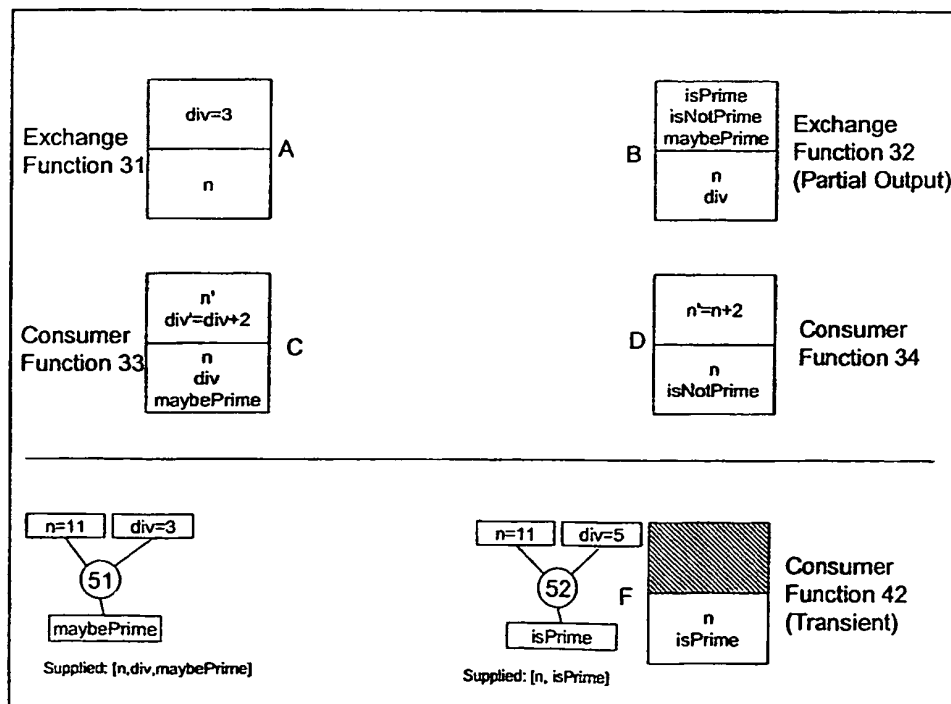
Figure 12 - Prime Numbers Example Application - Stage 8
