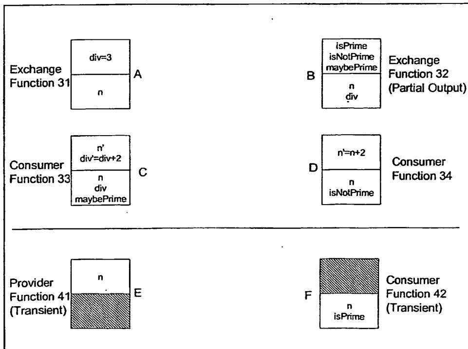
Figure 6 - Prime Numbers Example Application - Stage 2
