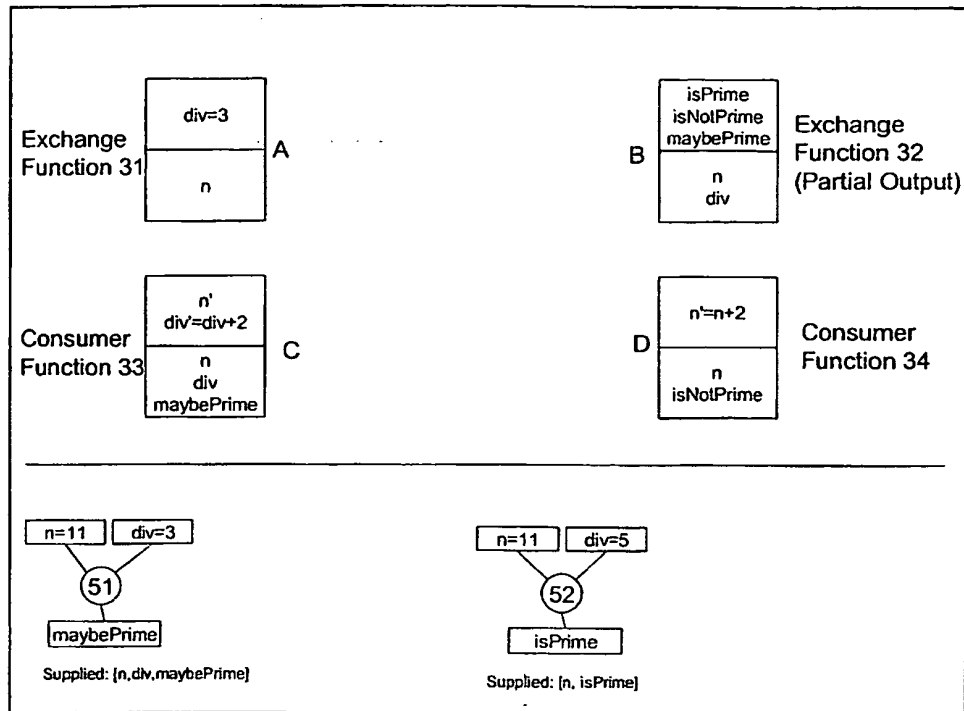
Figure 13 - Prime Numbers Example Application - Stage 9
