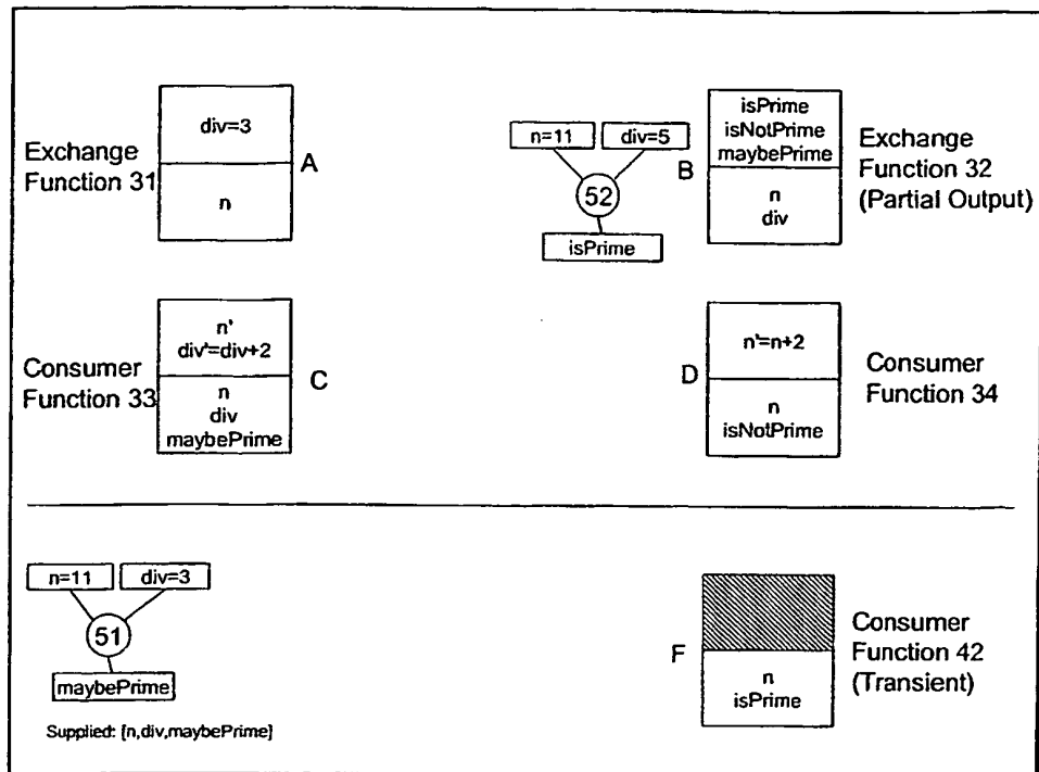
Figure 11 - Prime Numbers Example Application - Stage 7
