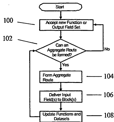
Figure 3 - Example Information Router Main Loop
