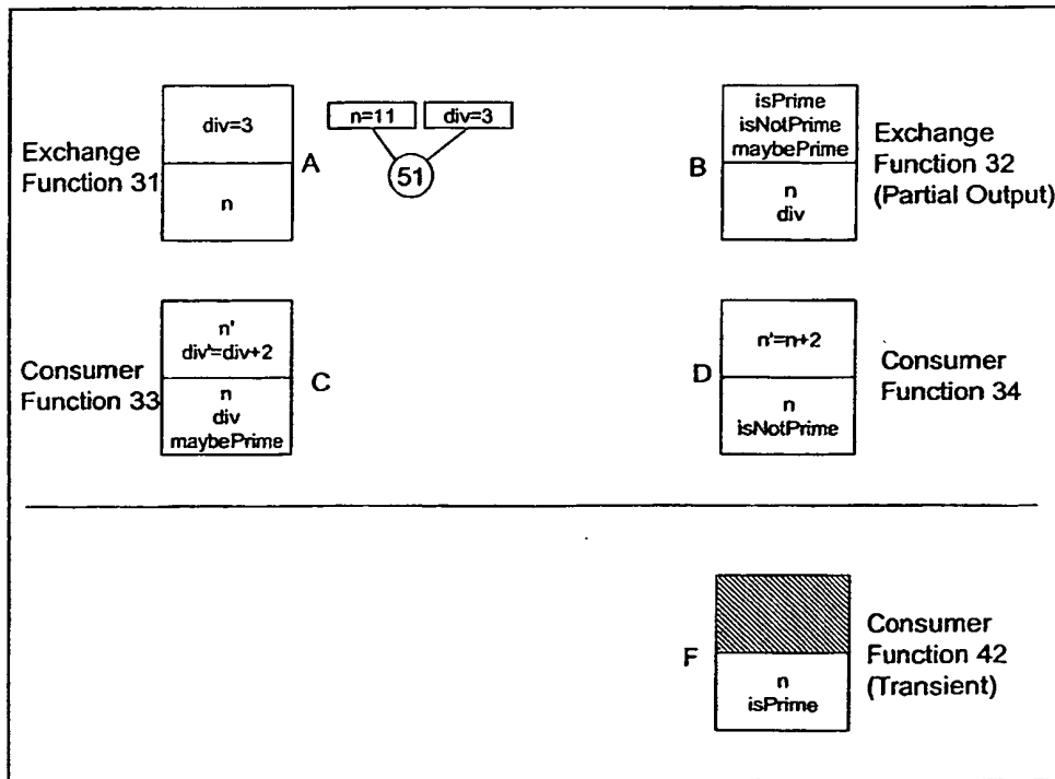
Figure 8 - Prime Numbers Example Application - Stage 4
