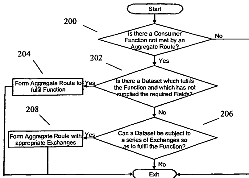
Figure 4 - Process Steps for Forming an Aggregate Route
