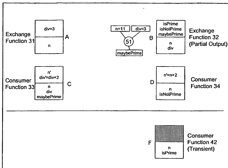
Figure 9 - Prime Numbers Example Application - Stage 5
