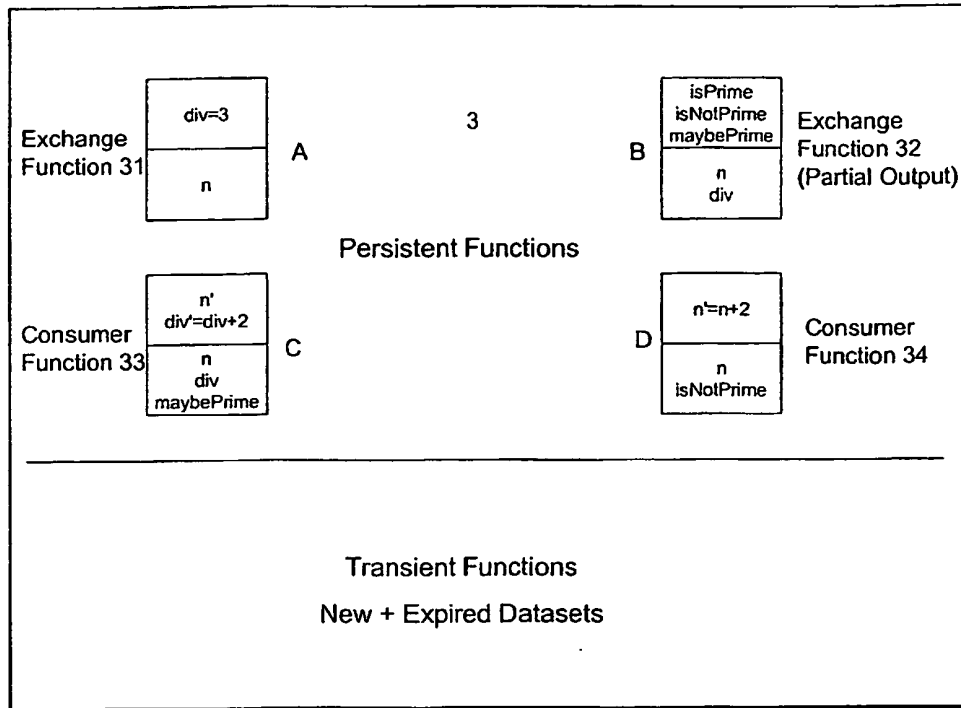
Figure 5 - Prime Numbers Example Application - Stage 1
