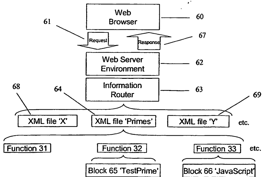
Figure 14 – Web based implementation
