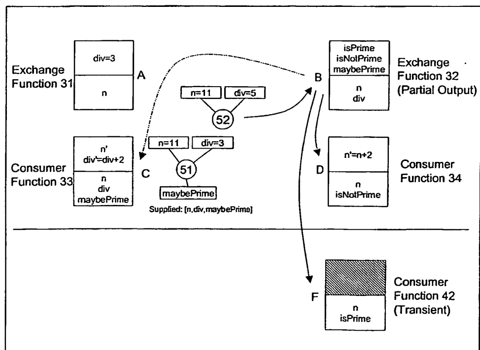
Figure 10 - Prime Numbers Example Application - Stage 6
