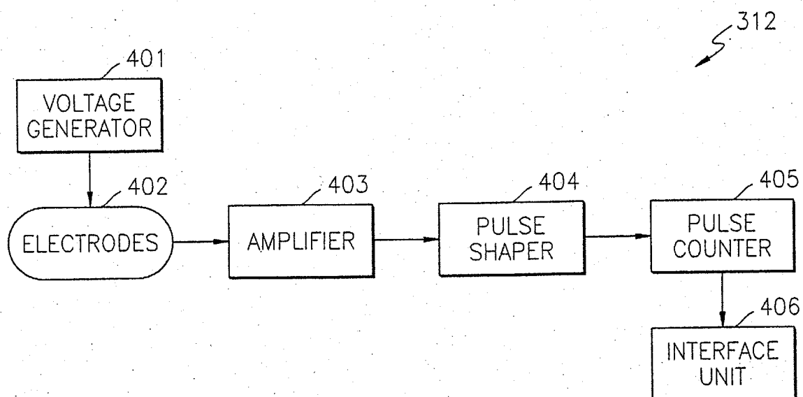
FIG. 4 (PRIOR ART)
