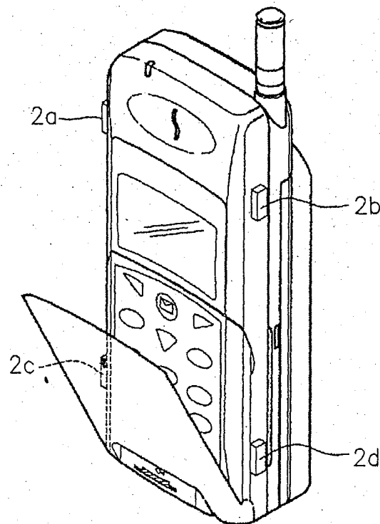
FIG. 2 (PRIOR ART)
