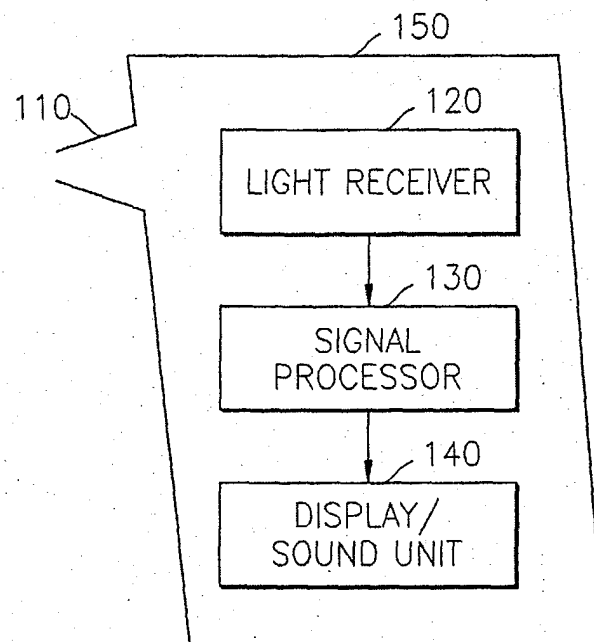
FIG. 1 (PRIOR ART)
