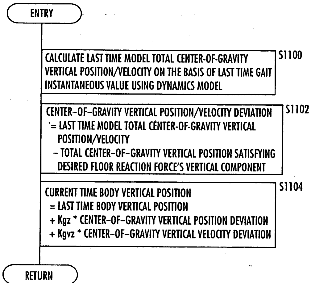
FIG.46 ( BODY VERTICAL POSITION DETERMINATION PROCESS: METHOD 1 )
