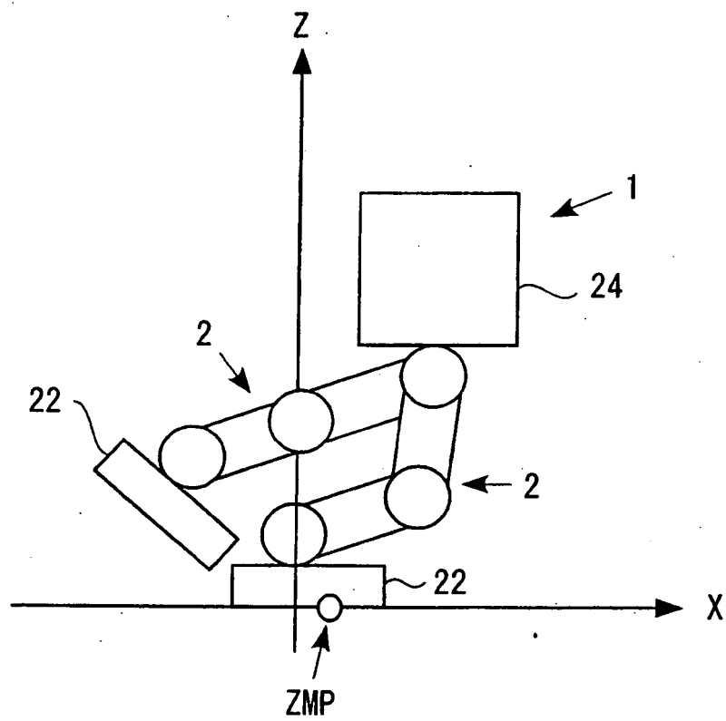
FIG.13 ( DIVERGENCE STATE OF BODY POSITION )
