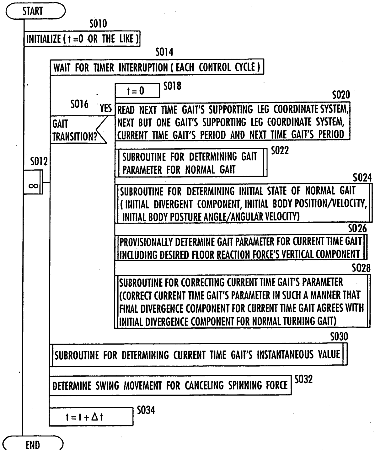
FIG.12 (FLOWCHART OF GAIT GENERATION PROCESS)
