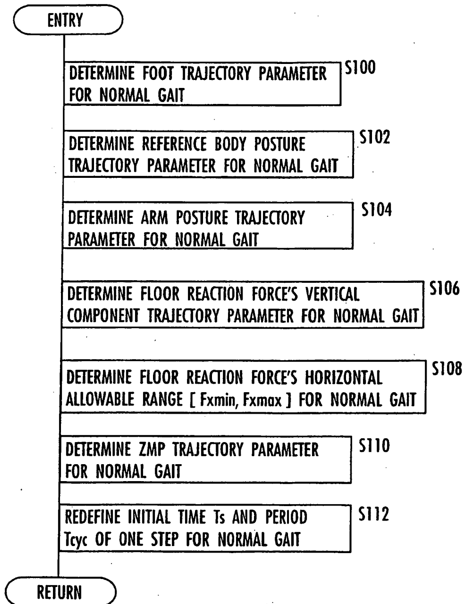
FIG.14 ( PROCESS OF DETERMINING NORMAL GAIT PARAMETER )
