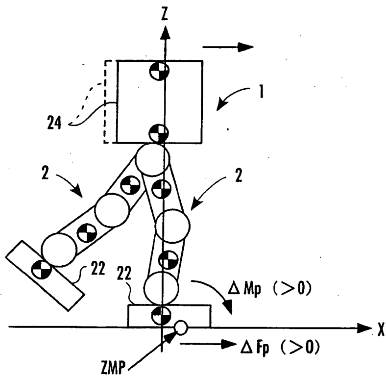
FIG.8 ( BODY TRANSLATION MODE )
