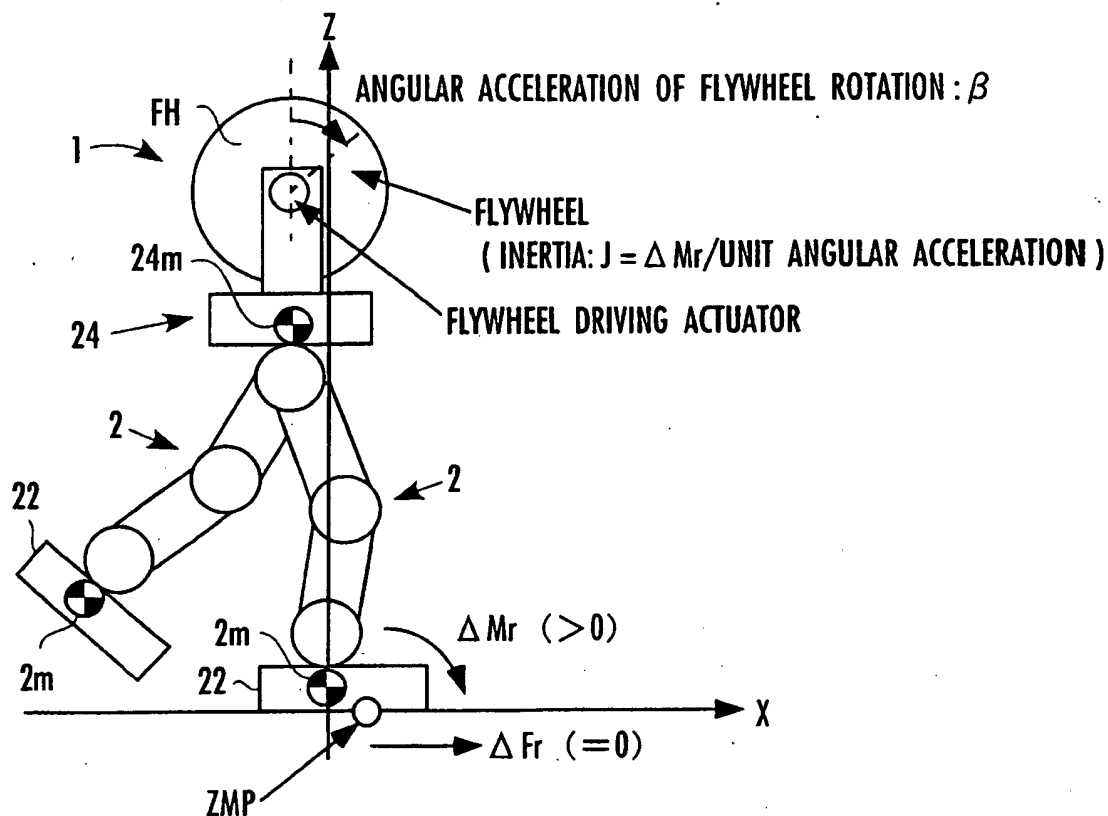
FIG.10 ( MODEL WITH FLYWHEEL )
