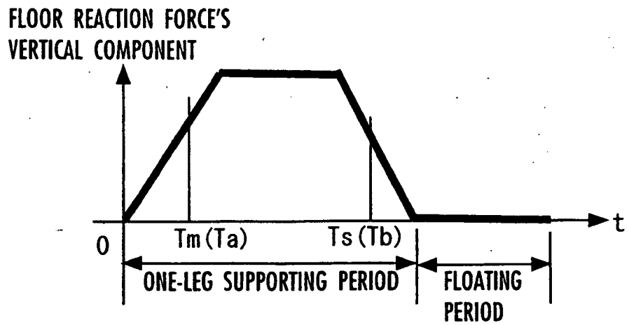
FIG.6 ( DESIRED FLOOR REACTION FORCE'S VERTICAL COMPONENT )
