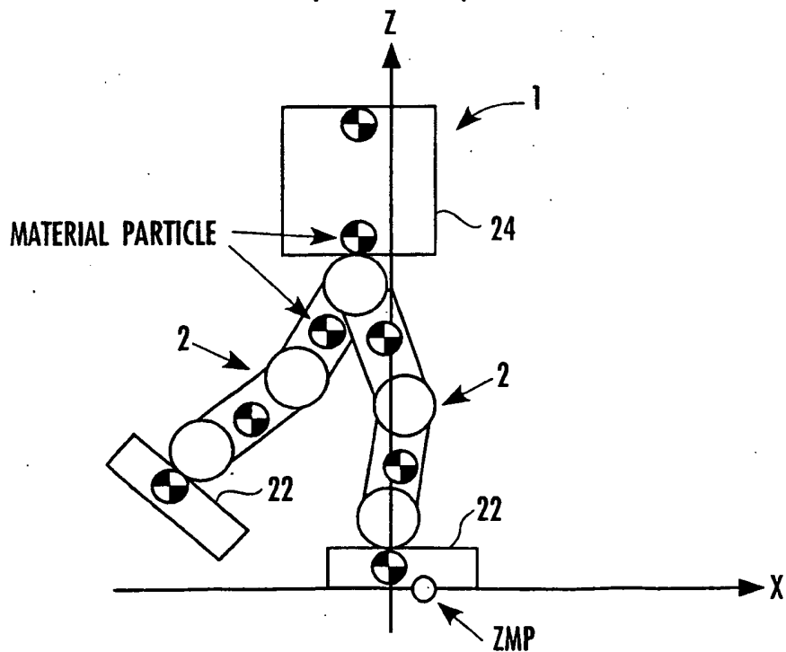
FIG.11 ( FULL MODEL )
