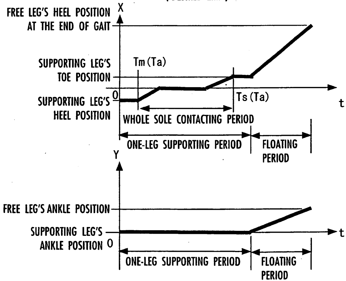
FIG.7 ( DESIRED ZMP )
