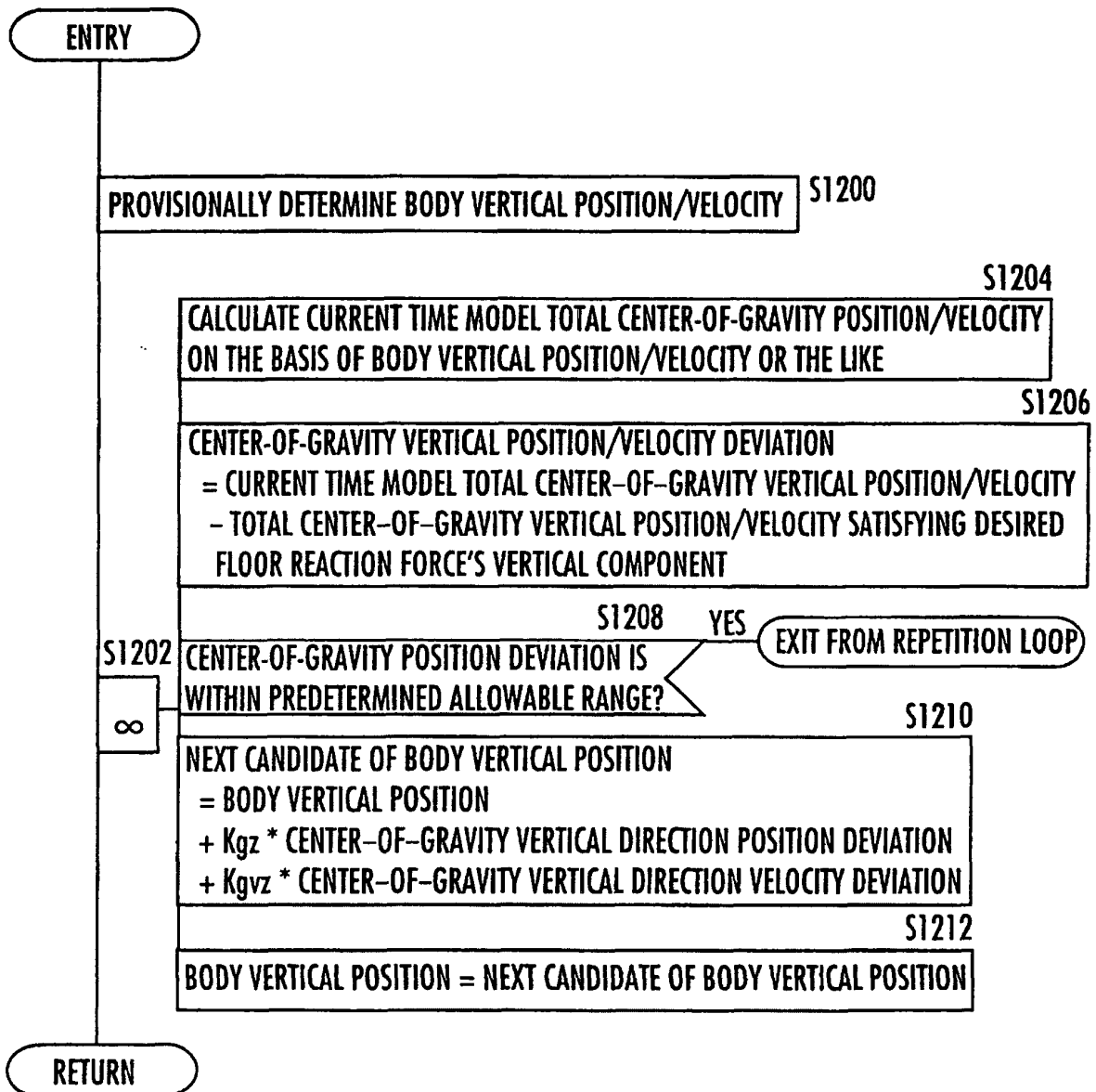
FIG.45 ( BODY VERTICAL POSITION DETERMINATION PROCESS: METHOD 2 )
