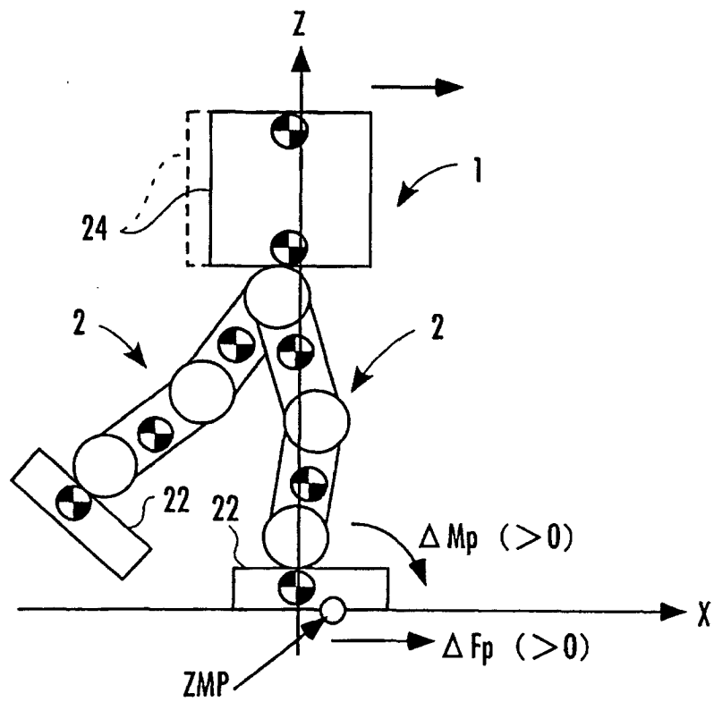
FIG.8 ( BODY TRANSLATION MODE )
