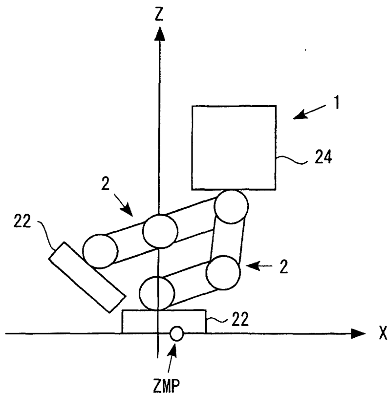
FIG.13 ( DIVERGENCE STATE OF BODY POSITION )
