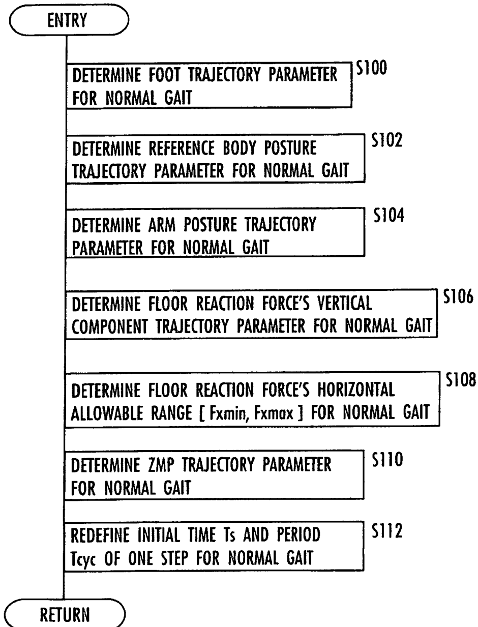
FIG.14 ( PROCESS OF DETERMINING NORMAL GAIT PARAMETER )
