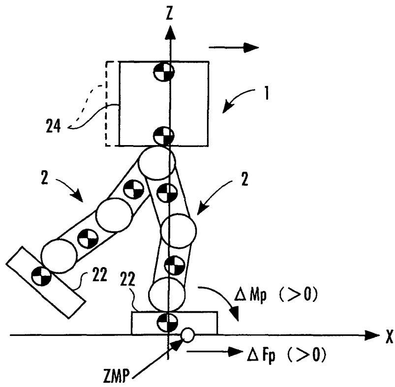
FIG.8 ( BODY TRANSLATION MODE )
