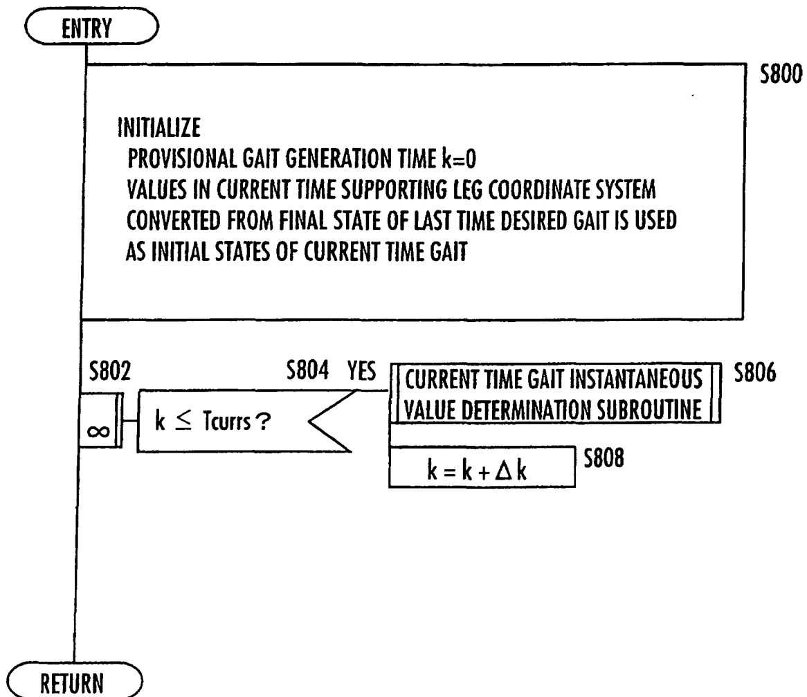
FIG.35 ( PROCESS OF GENERATING PROVISIONAL CURRENT TIME GAIT )
