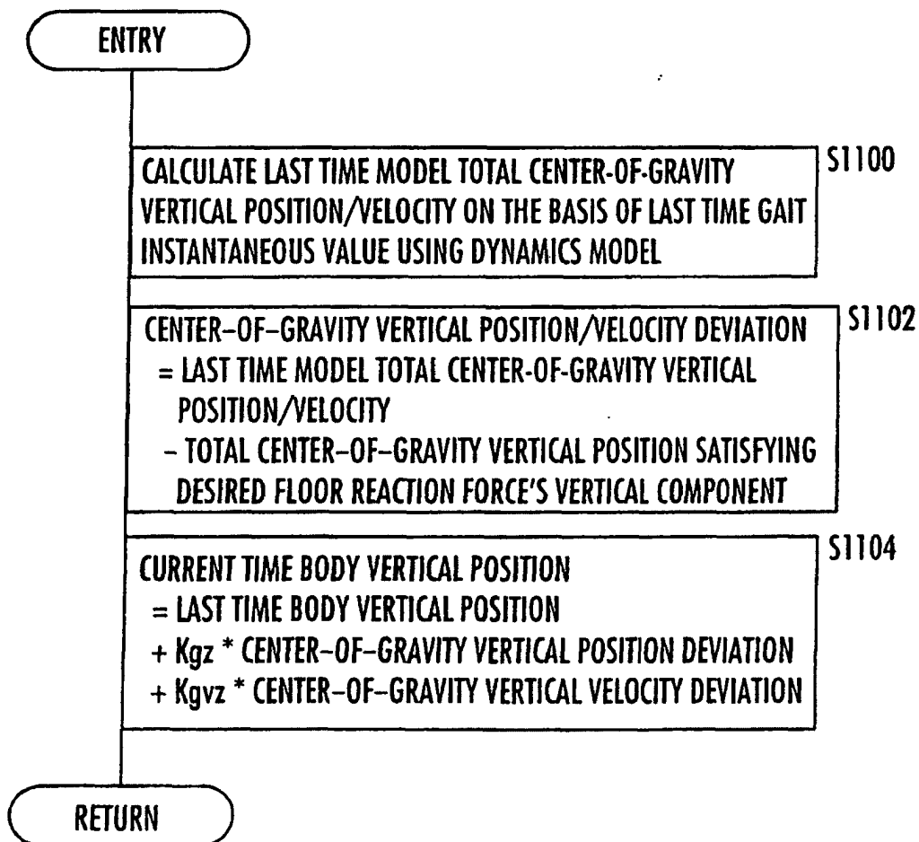
FIG.46 ( BODY VERTICAL POSITION DETERMINATION PROCESS: METHOD 1 )
