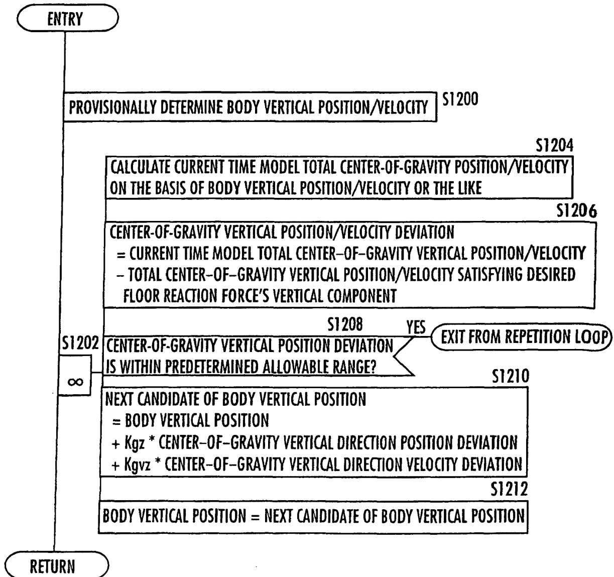
FIG.47 ( BODY VERTICAL POSITION DETERMINATION PROCESS: METHOD 2 )
