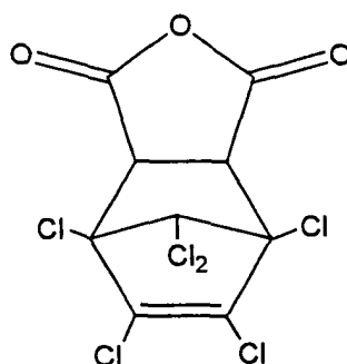
[Chlorendic anhydride]
