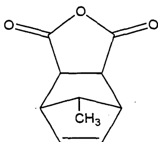
[Methylenendomethylenetetrahydrophthalate anhydride]
