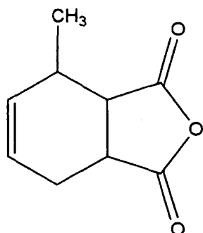
[Methyltetrahydrophthalic anhydride]
