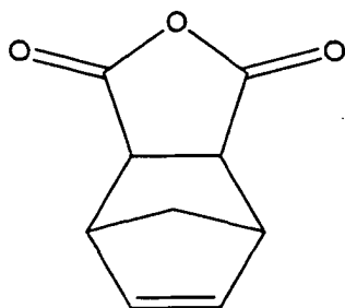
[Endomethylenetetrahydrophthalic anhydride]
