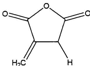
[Itaconic anhydride]
