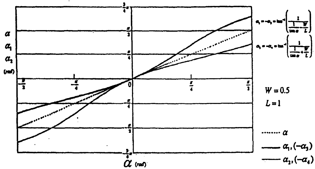
Steering Angles \alpha_1 Through \alpha_4 When \alpha_0 is Used as the Steering Command Value (Steering Mode M1)
