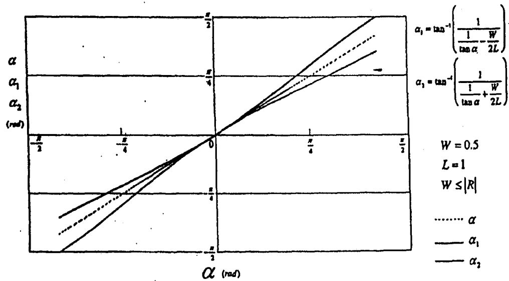
Steering Angles \alpha_1 and \alpha_2 When \alpha_0 is Used as the Steering Command Value (Steering Mode M3)
