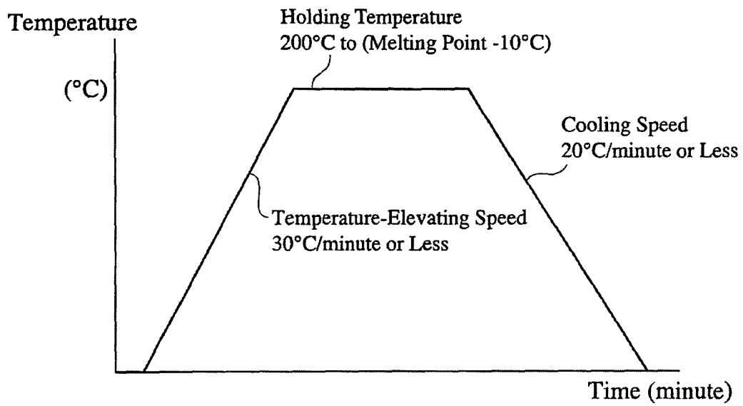
Heat Treatment Pattern
