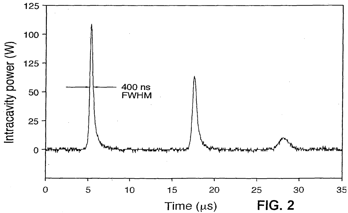
Typical relaxation-oscillation pulse-train near threshold
