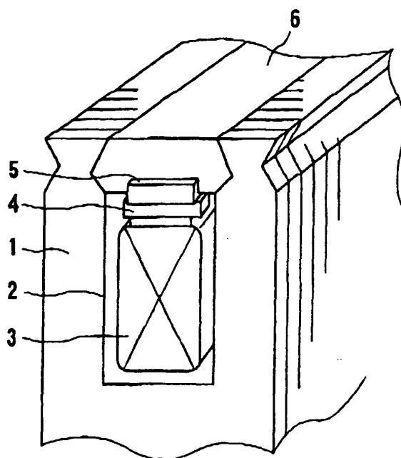
FIG. 19 PRIOR ART
