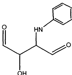
2-Benzylamino-3-hydroxy-succindialdehyde
