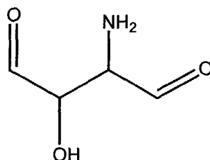
2-Amino-3-hydroxy-succindialdehyde
