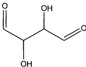
2,3-dihydroxy-succindialdehyde
