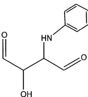
2-Benzylamino-3-hydroxy-succindialdehyde
