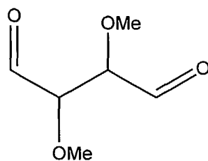
2,3-Dimethoxysuccindialdehyde
