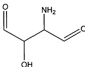
2-Amino-3-hydroxy-succindialdehyde
