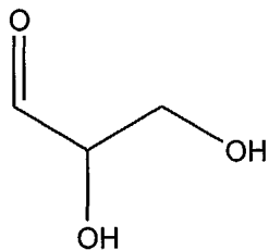
Glyceraldehyde
