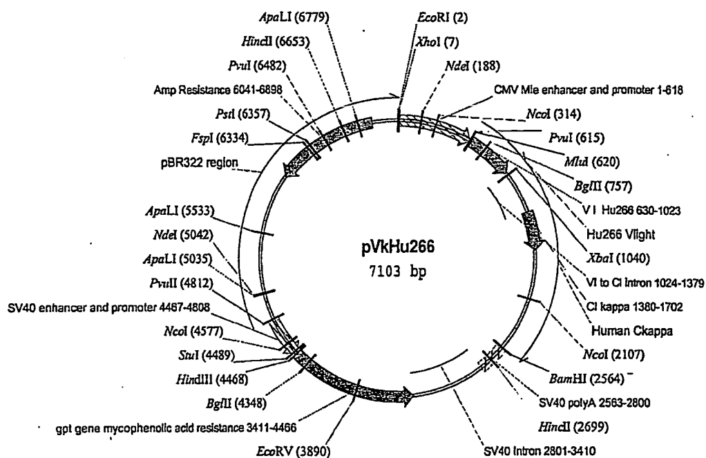
Figure 6. Plasmid pVkJHu266
