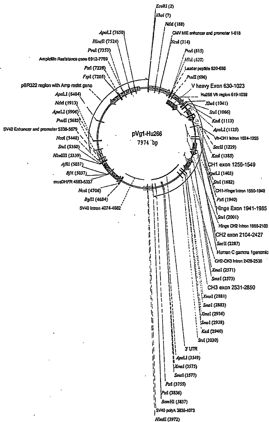
Figure 7 Plasmid pVg1-Hu266
