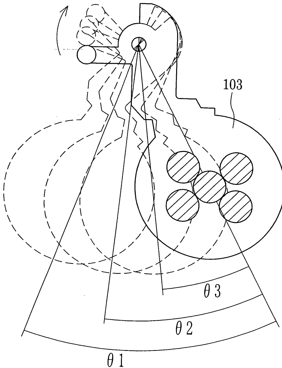
FIG.17 (PRIOR ART)
