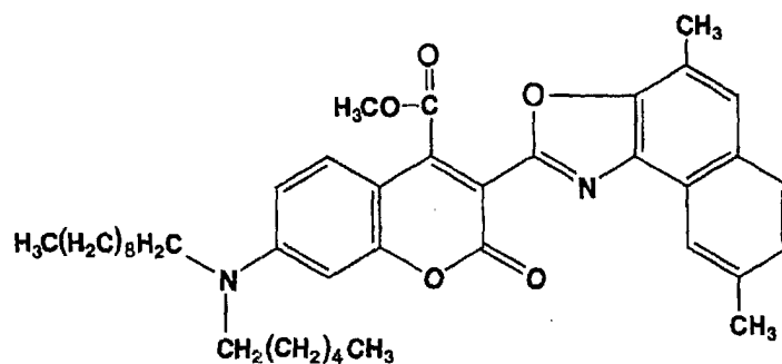
Chemical Formula 10:
