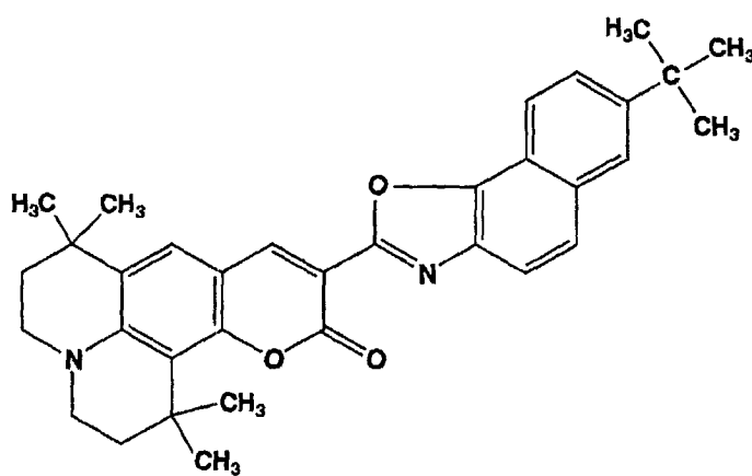
Chemical Formula 18:
