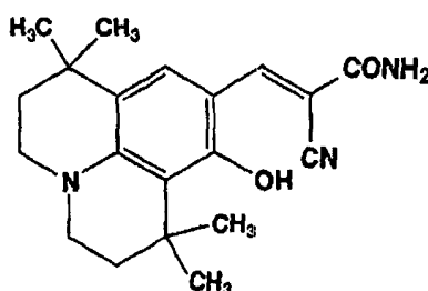
Chemical Formula 60:
