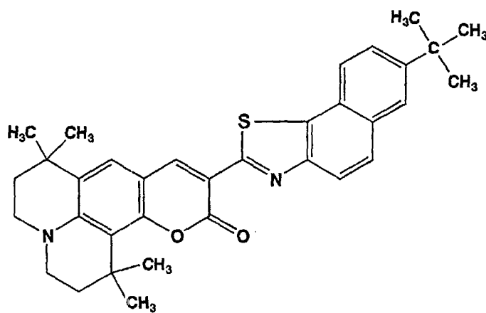
Chemical Formula 18:
