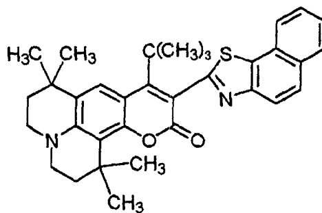
Chemical Formula 51:
