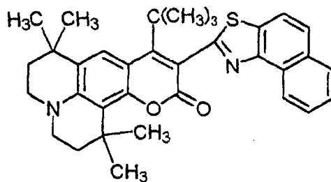
Chemical Formula 53:
