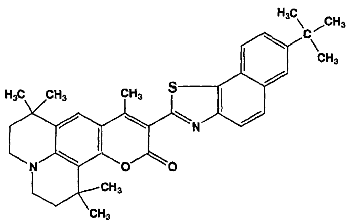
Chemical Formula 20:
