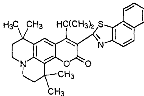
Chemical Formula 49:
