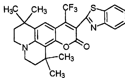
Chemical Formula 39:
