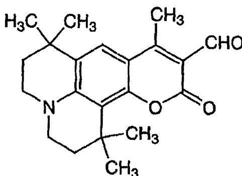
Chemical Formula 68:
