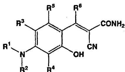
General Formula 7:
