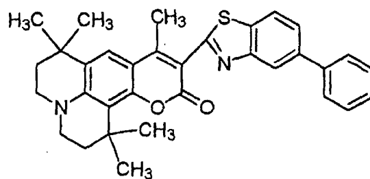
Chemical Formula 37:
