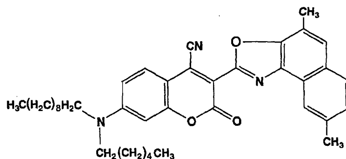
Chemical Formula 10:
