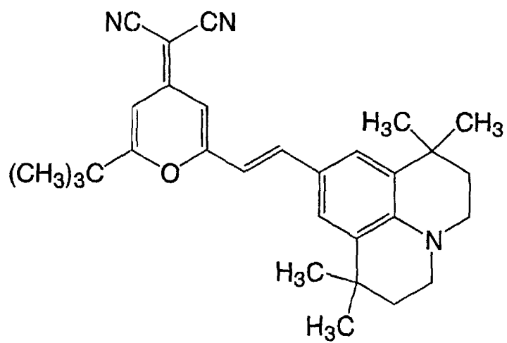
Chemical Formula 29:
