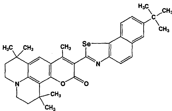
Chemical Formula 23:
