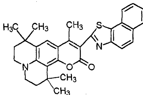
Chemical Formula 34:
