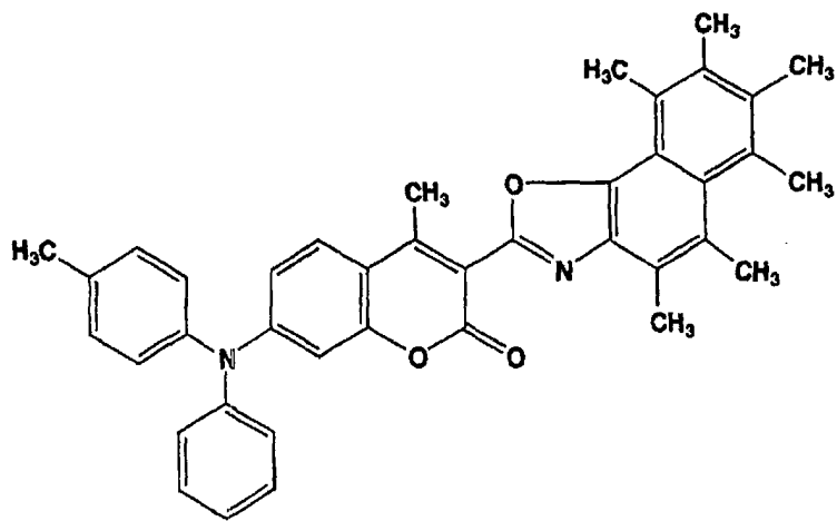
Chemical Formula 27:
