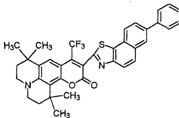
Chemical Formula 43:
