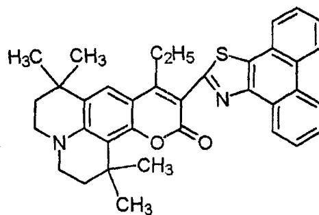
Chemical Formula 48:
