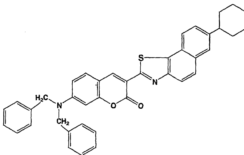
Chemical Formula 15:
