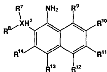
General Formula 9:
