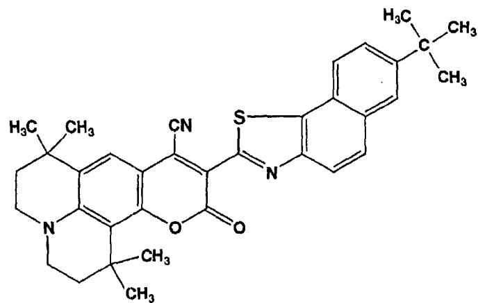
Chemical Formula 21:
