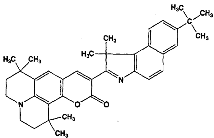
Chemical Formula 19:
