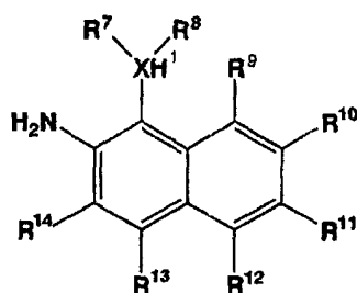
General Formula 8:
