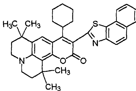
Chemical Formula 56:
