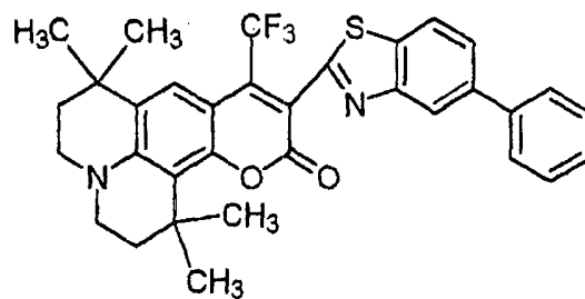
Chemical Formula 43:
