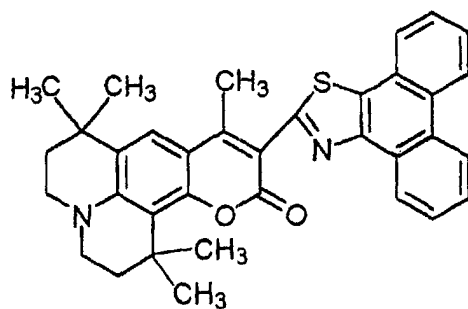
Chemical Formula 37:
