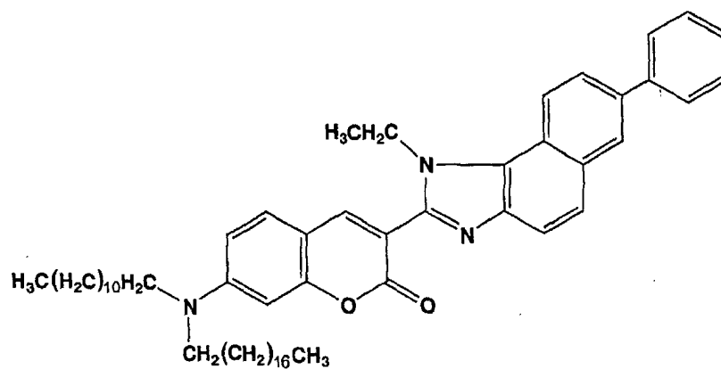
Chemical Formula 12:
