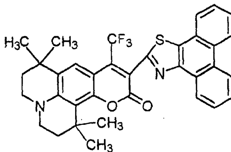
Chemical Formula 45:
