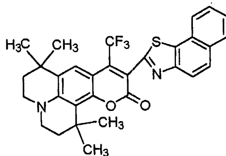
Chemical Formula 39:
