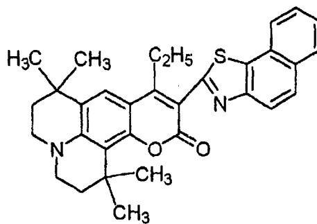
Chemical Formula 46:
