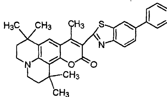
Chemical Formula 35:
