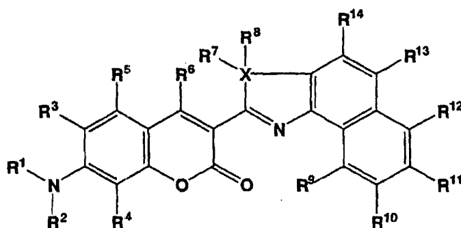
General Formula 2:
