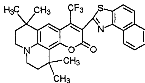
Chemical Formula 41:
