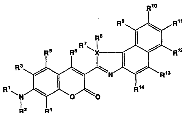
General Formula 1:
