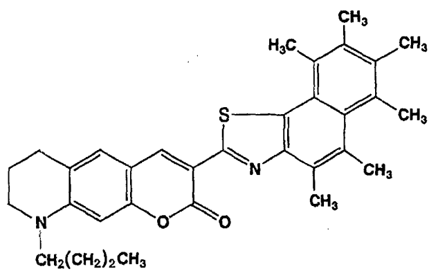
Chemical Formula 26:
