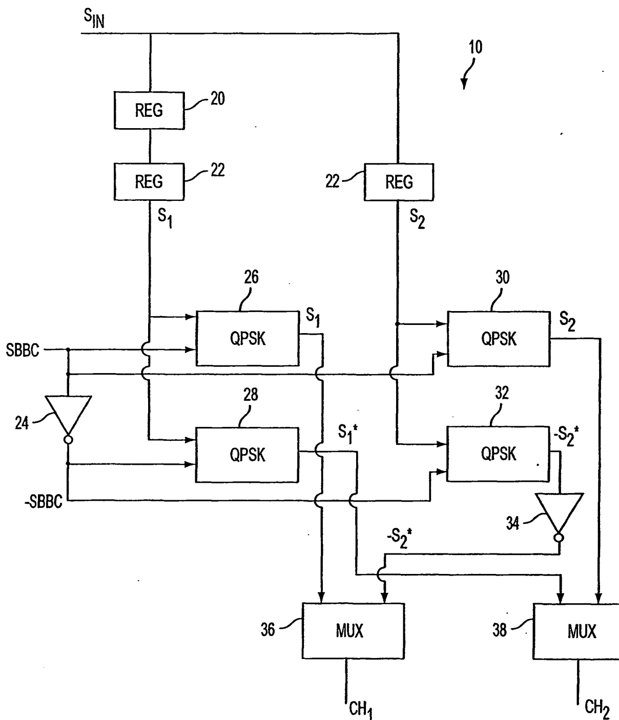
FIG. 3 (PRIOR ART)
