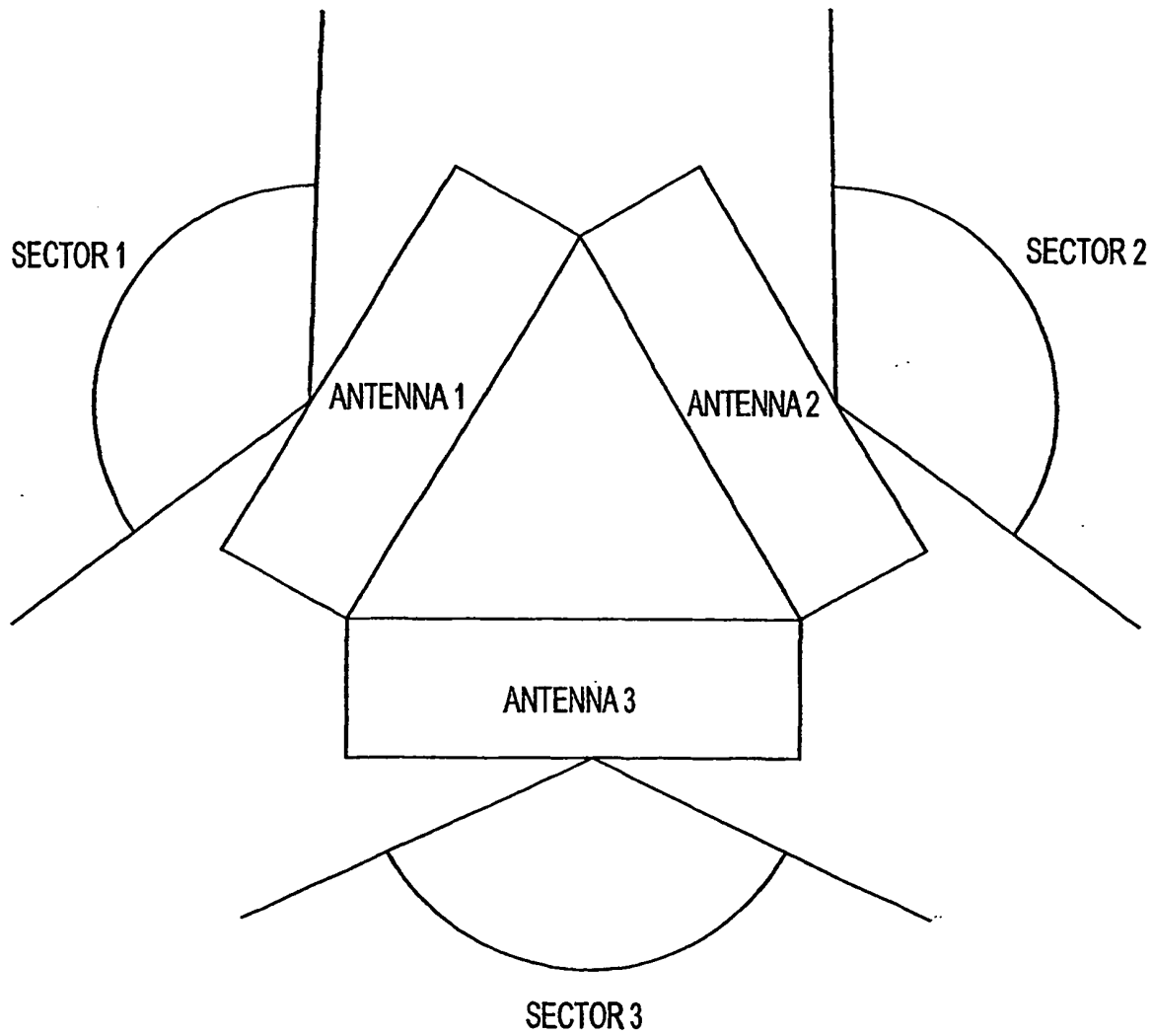
FIG. 8 (PRIOR ART)
