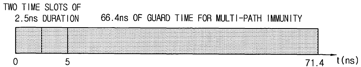
BINARY PPM-APPLIED TIME FRAME STRUCTURE
