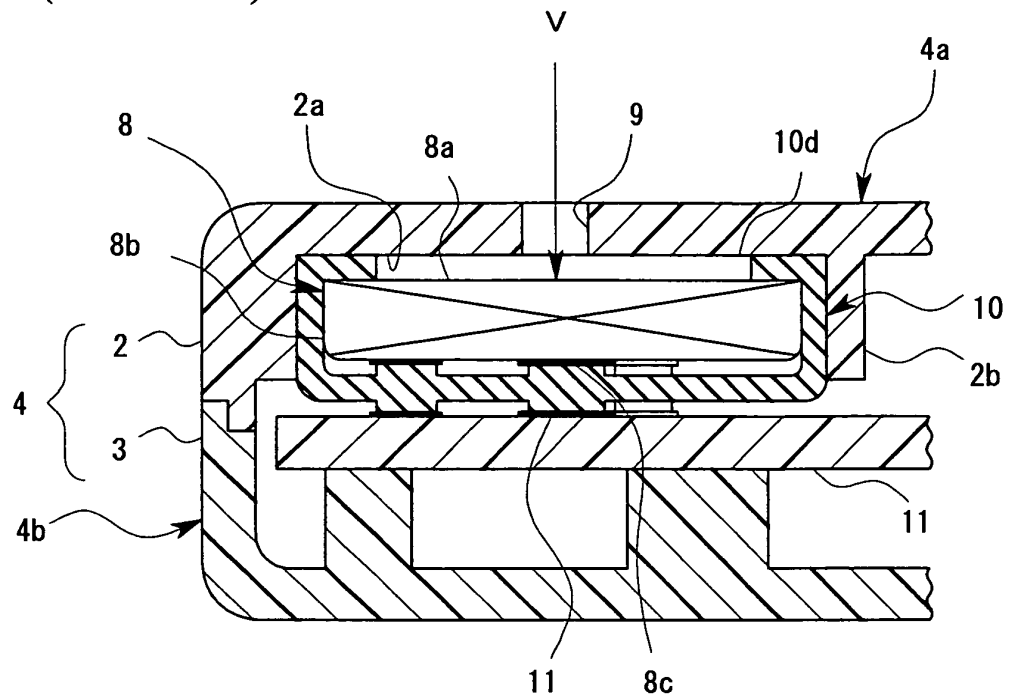
Fig.7 (Prior Art)
