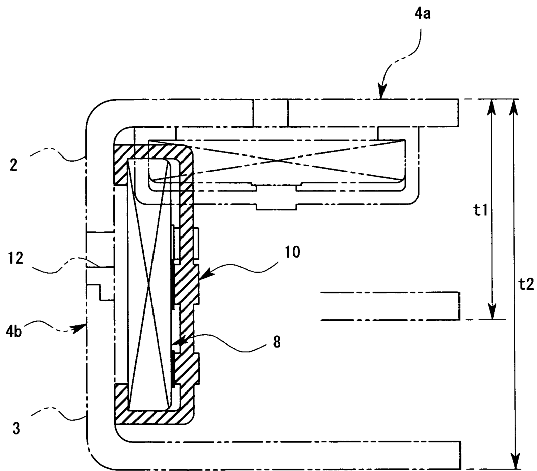
Fig.9 (Prior Art)
