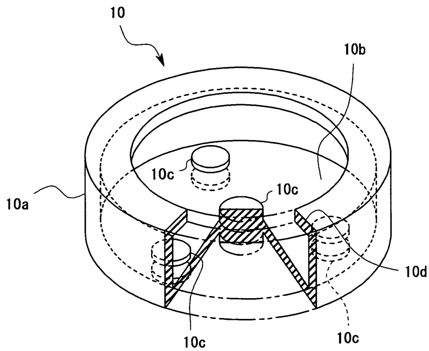
Fig.8 (Prior Art)
