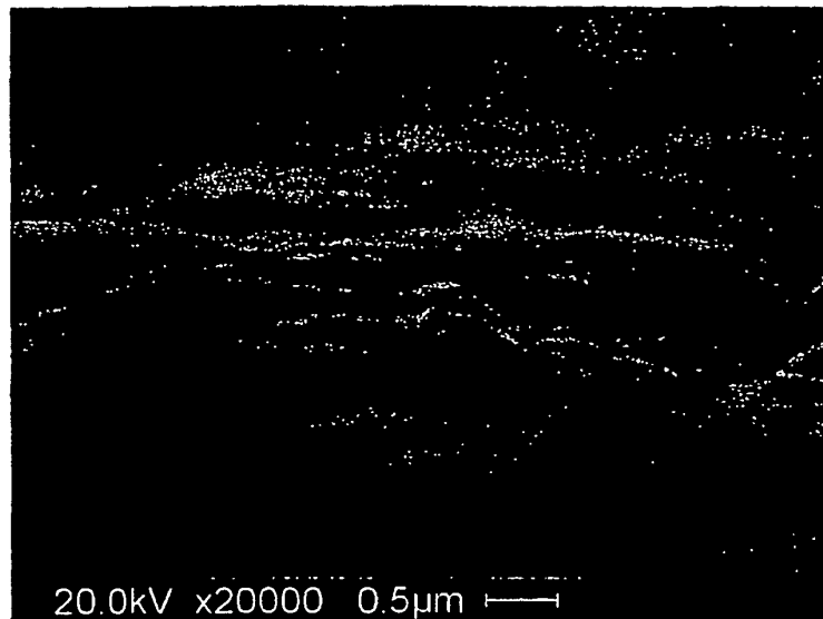
SCANNING ELECTRON MICROGRAPH OF COMPARATIVE SAMPLE (SAMPLE NO. 5) TAKEN IN HORIZONTAL DIRECTION
