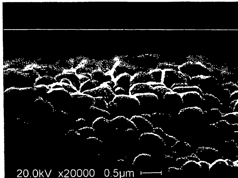
SCANNING ELECTRON MICROGRAPH OF ROUGHENED SAMPLE SURFACE TAKEN IN HORIZONTAL DIRECTION
