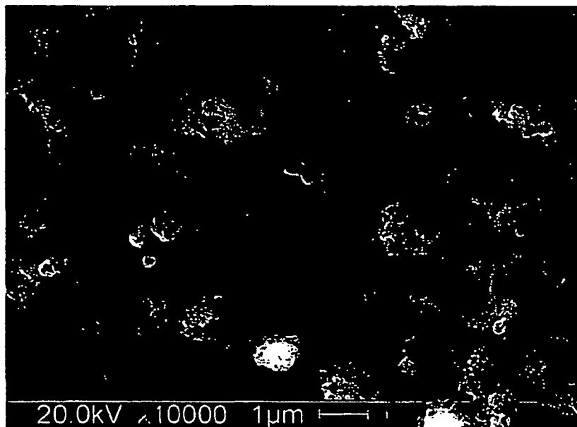
SCANNING ELECTRON MICROGRAPH AFTER FORMATION OF THE CALCIUM PHOSPHATE COMPOUND COATING
