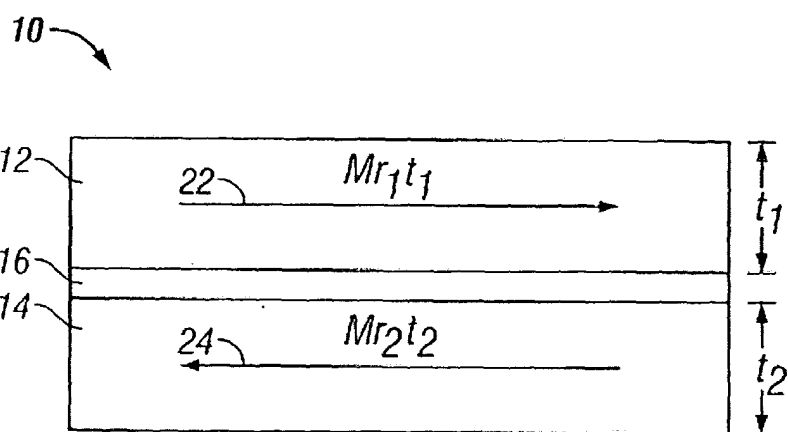
FIG. 1 (Prior Art)
