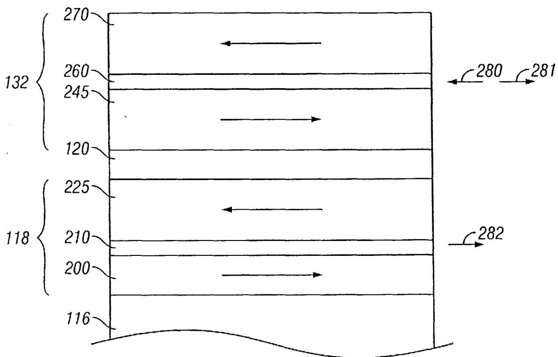
FIG. 4 (Prior Art)
