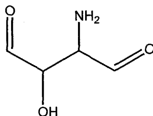
2-Amino-3-hydroxy-succindialdehyde
