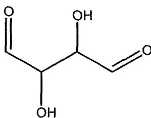
2,3-dihydroxy-succindialdehyde
