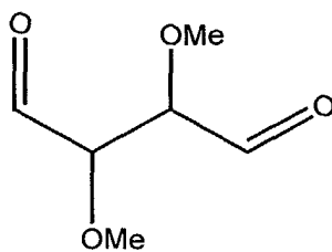
2,3-Dimethoxysuccindialdehyde
