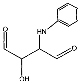
2-Benzylamino-3-hydroxy-succindialdehyde
