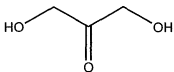
Dihydroxyacetone
