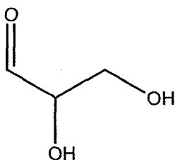
Glyceraldehyde
