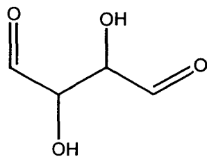
2,3-dihydroxy-succindialdehyde
