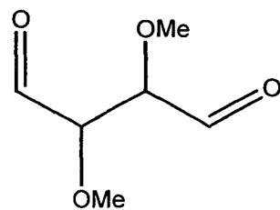
2,3-Dimethoxysuccindialdehyde
