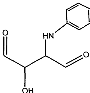
2-Benzylamino-3-hydroxy-succindialdehyde
