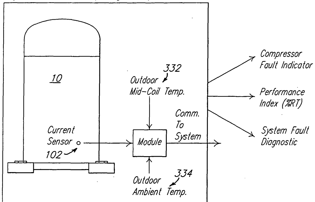
Integrated Protection/Diagnostic/Defrost Control
