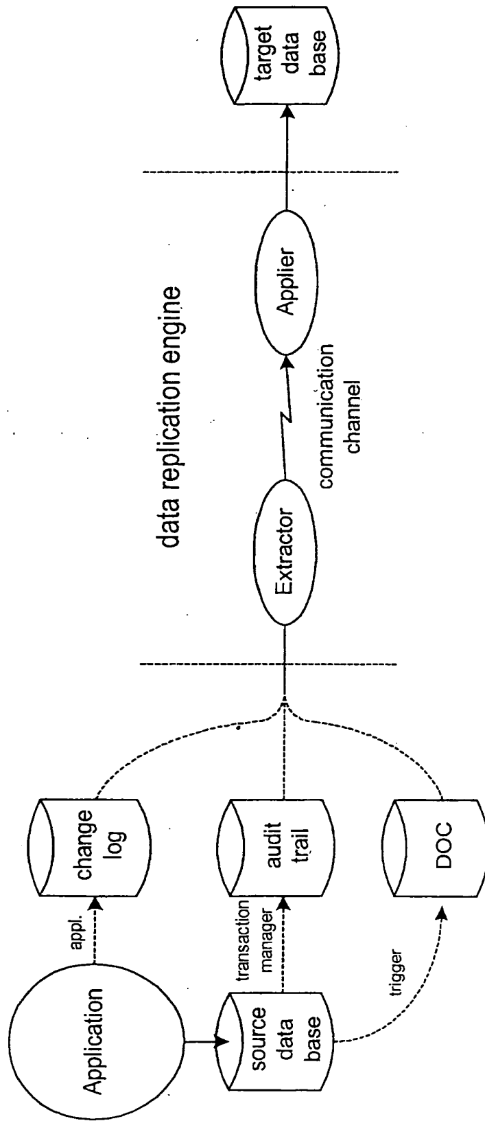
Simple Data Replication Engine
