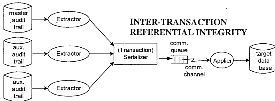
Use of a Transaction Serializer
