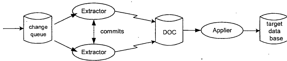
Transaction Serializing with Extractor Coordination
