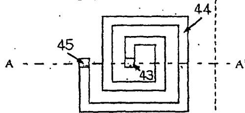
Fig. 4 (b) Top view of the second layer
