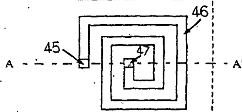
Fig. 4 (c) Top view of the third layer
