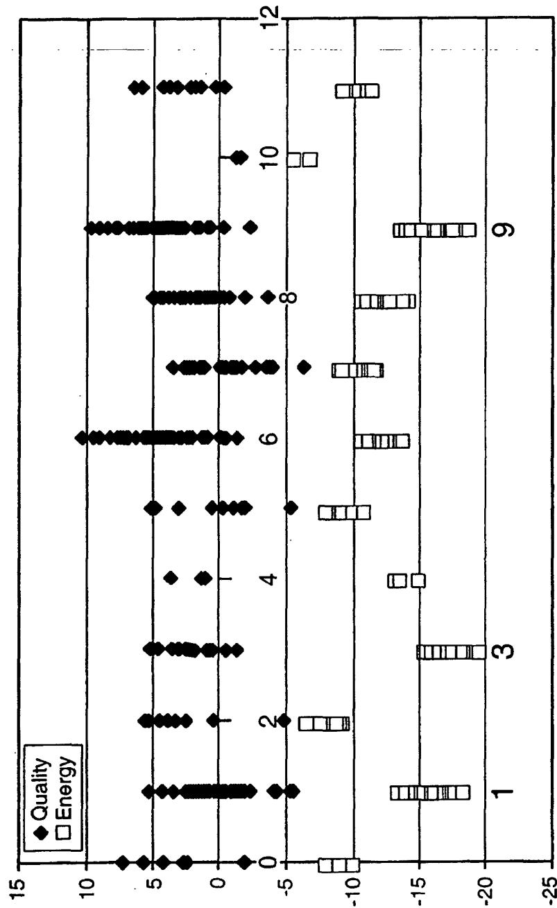
Cluster Number
