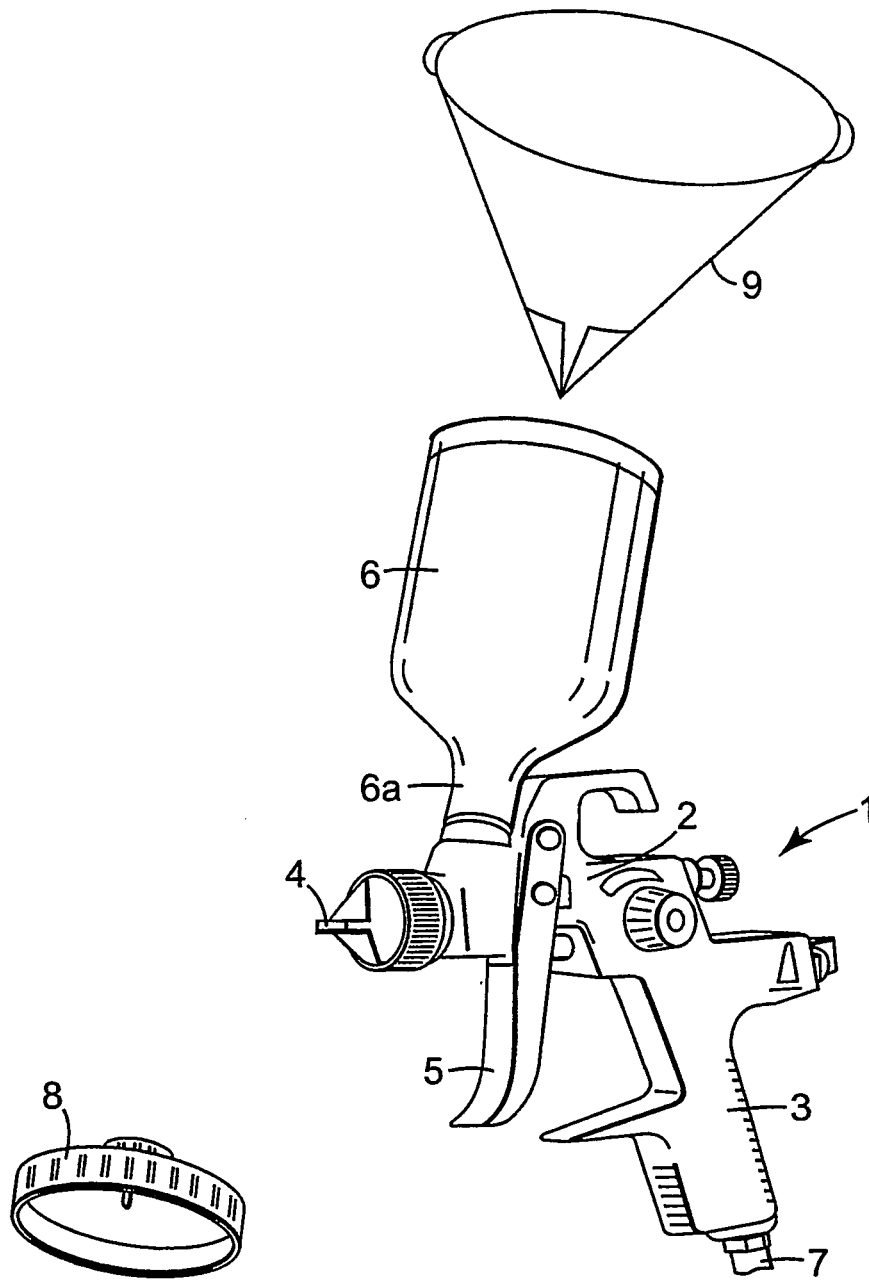
FIG. 1 PRIOR ART
