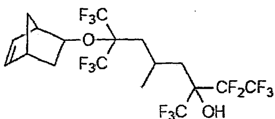
7-bicyclo[2.2.1]hept-5-en-2-yloxy-3,7-bis(trifluoromethyl)-1,1,1,2,2,8,8,8-octafluoro-5-methyloctan-3-ol
