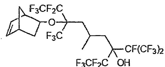
7-bicyclo[2.2.1]hept-5-en-2-yloxy-1,1,1,2,2,8,8,9,9-decafluoro-5-methyl-3-[1,2,2,2-tetrafluoro-1-(trifluoromethyl)ethyl]-7-(trifluoromethyl)nonan-3-ol
