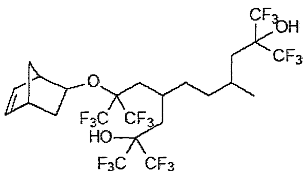
4-[2-bicyclo[2.2.1]hept-5-en-2-yloxy-3,3,3-trifluoro-2-(trifluoromethyl)propyl]-2,9-bis(trifluoromethyl)-1,1,1,10,10,10-hexafluoro-7-methyldecane-2,9-diol
