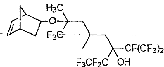
7-bicyclo[2.2.1]hept-5-en-2-yloxy-1,1,1,2,2,8,8,8-octafluoro-5,7-dimethyl-3-[1,2,2,2-tetrafluoro-1-(trifluoromethyl)ethyl]octan-3-ol
