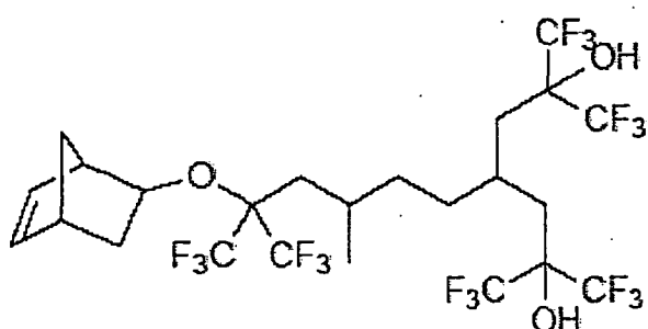
4-[5-bicyclo[2.2.1]hept-5-en-2-yloxy-6,6,6-trifluoro-3-methyl-5-(trifluoromethyl)hexyl]-2,6-bis(trifluoromethyl)-1,1,1,7,7,7-hexafluoroheptane-2,6-diol
