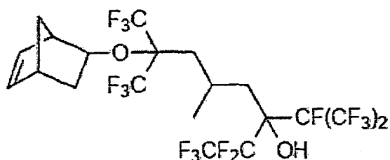
7-bicyclo[2.2.1]hept-5-en-2-yloxy-1,1,1,2,2,8,8,8-octafluoro-5-methyl-3-[1,2,2,2-tetrafluoro-1-(trifluoromethyl)ethyl]-7-(trifluoromethyl)octan-3-ol
