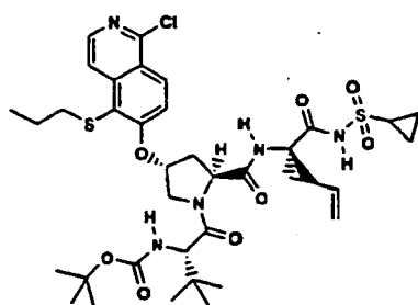
Compound 204
