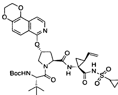
Compound 286
