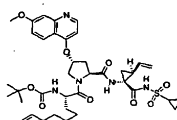
Compound 377
