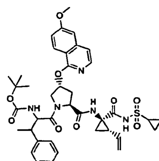
Compound 136
