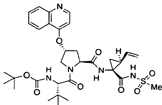
Compound 386
