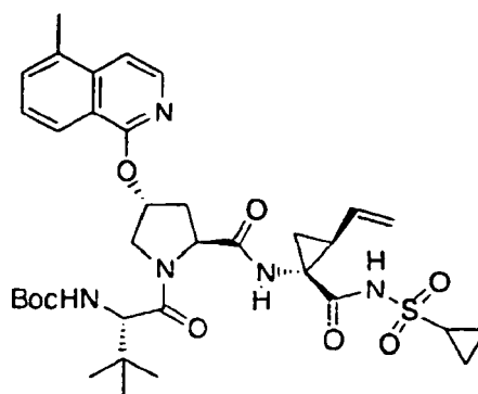
Compound 252
