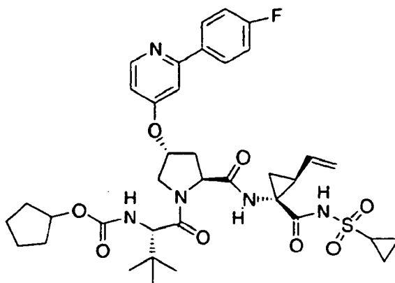
Compound 427
