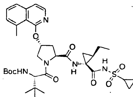
Compound 297
