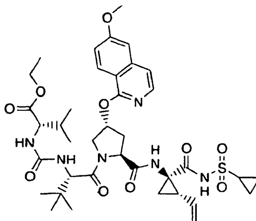
Compound 148
