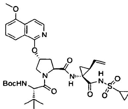
Compound 253
