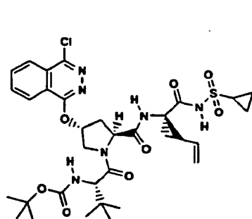
Compound 195
