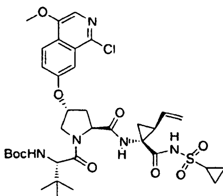
Compound 283
