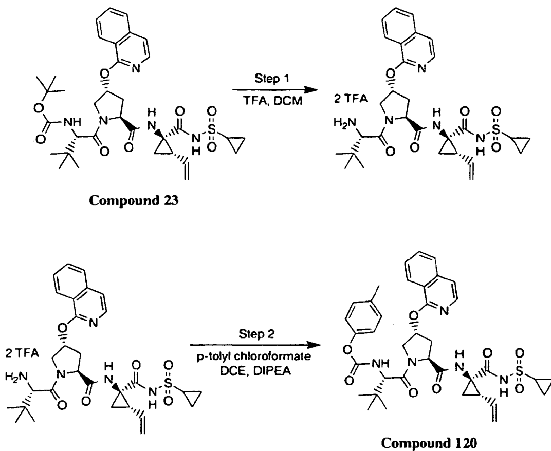
Scheme 1
