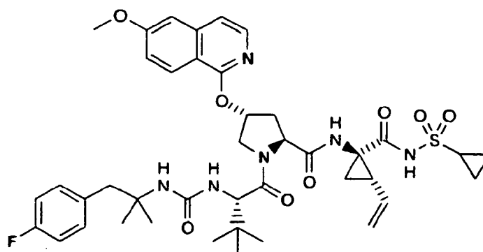
Compound 82
