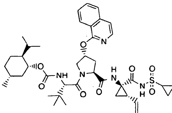
Compound 128
