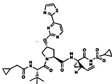
Compound 340
