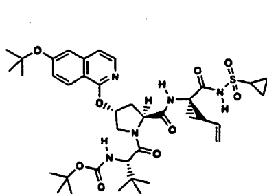
Compound 193
