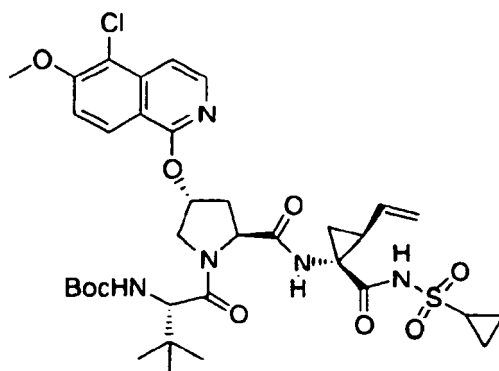
Compound 275
