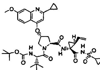
Compound 373
