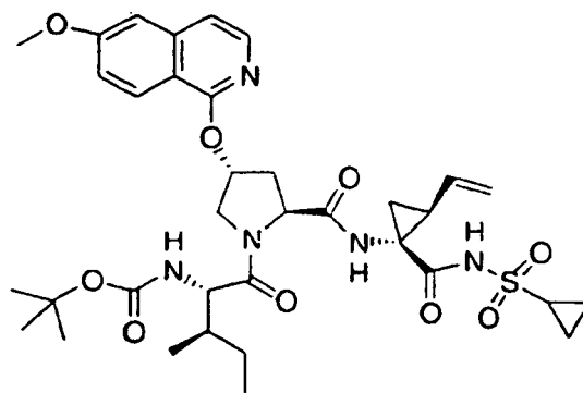
Compound 13
