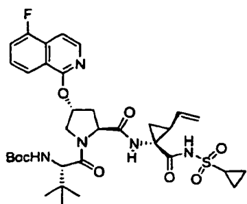
Compound 255
