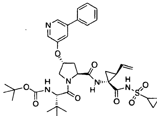
Compound 420
