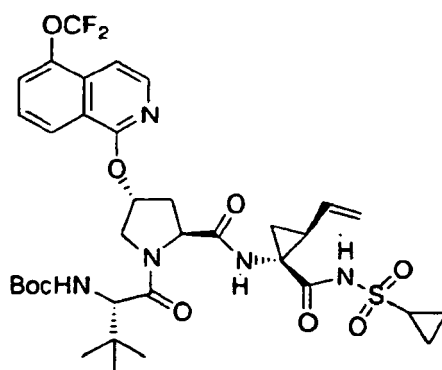
Compound 285
