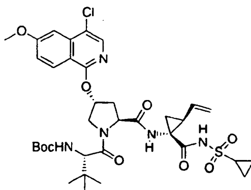
Compound 278
