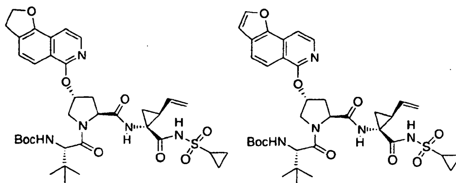
Compound 265
