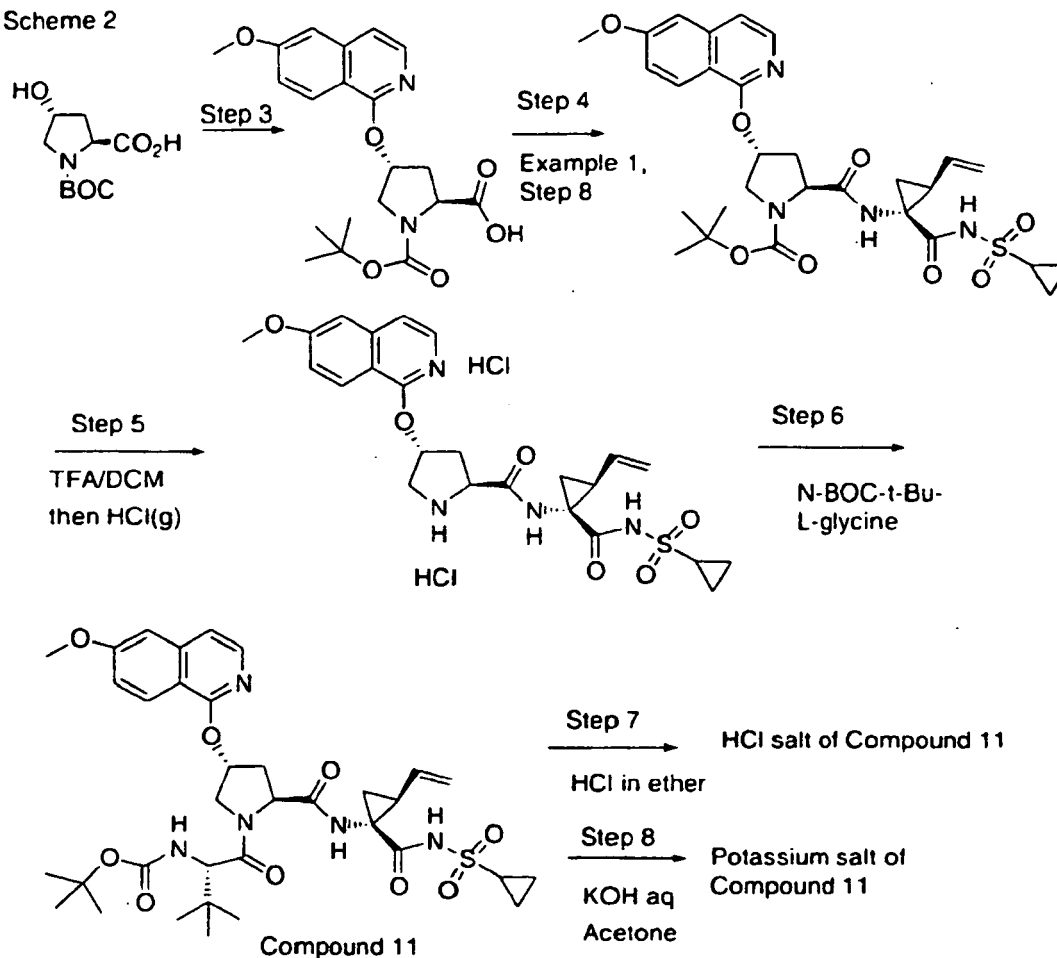
Scheme 2
