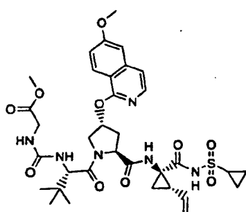
Compound 144
