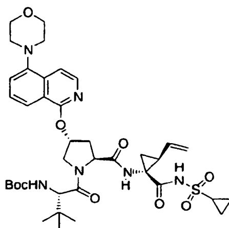
Compound 271
