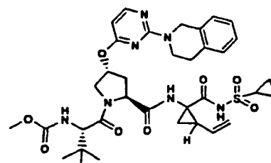
Compound 341
