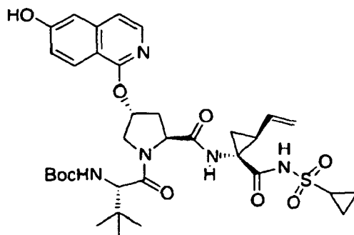
Compound 280
