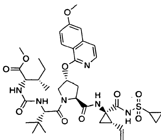
Compound 151
