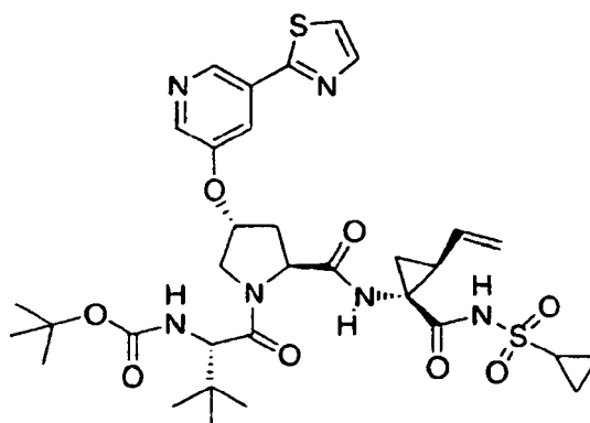
Compound 432
