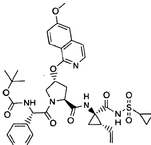
Compound 134
