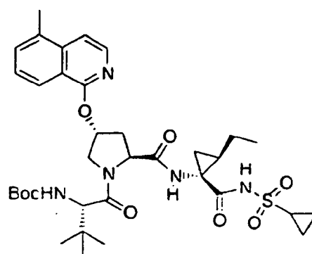
Compound 293
