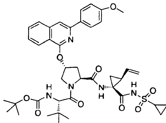
Compound 26
