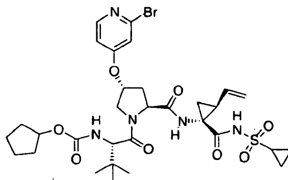
Compound 425
