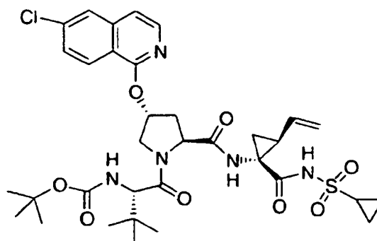
Compound 20
