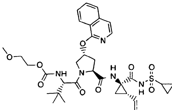
Compound 124
