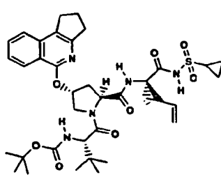
Compound 215
