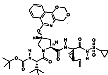
Compound 227
