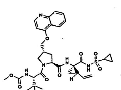
Compound 344
