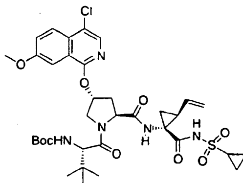
Compound 284
