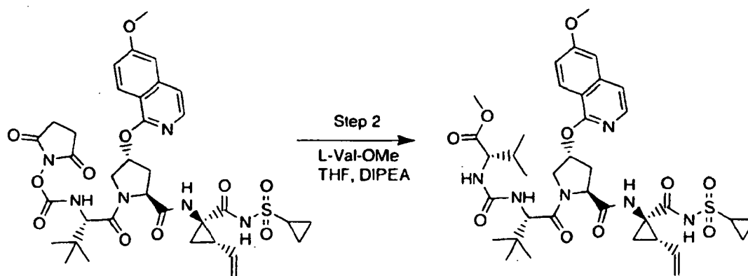
Compound 141
