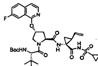
Compound 257
