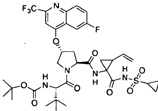
Compound 450
