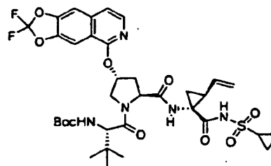
Compound 288
