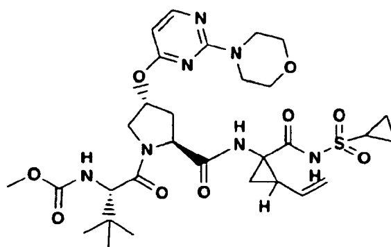
Compound 343
