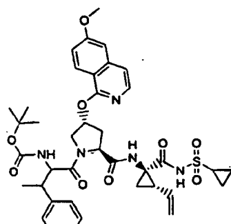
Compound 135
