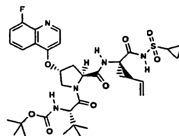
Compound 241
