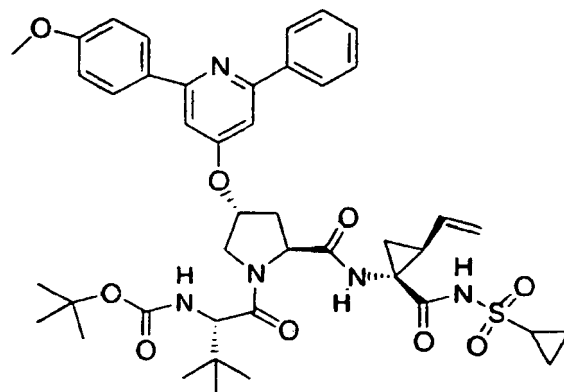
Compound 414
