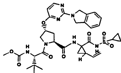
Compound 342
