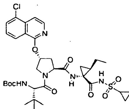
Compound 294
