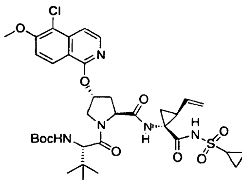
Compound 275
