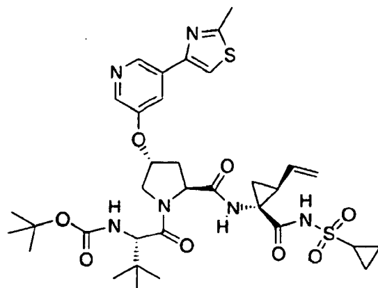
Compound 433
