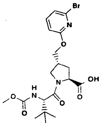
intermediate 9
