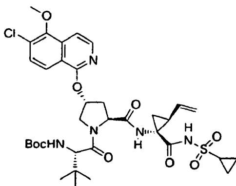
Compound 276
