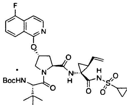
Compound 255
