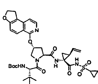
Compound 267
