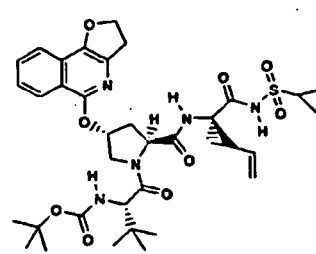
Compound 219
