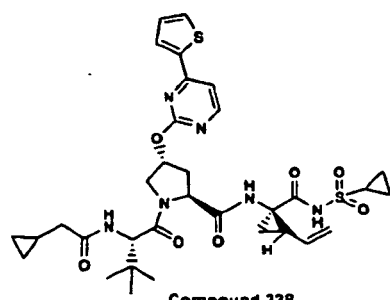
Compound 338
