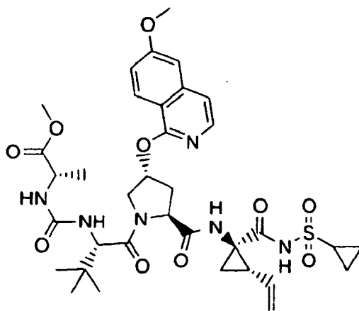
Compound 145
