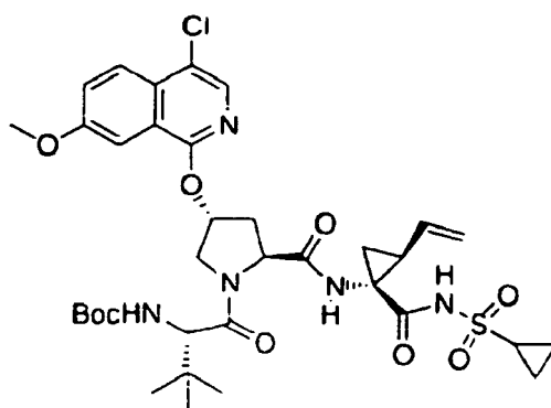
Compound 284
