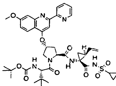
Compound 379
