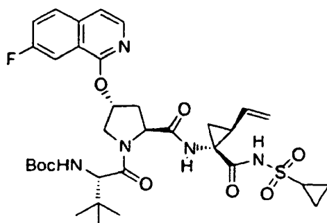
Compound 257
