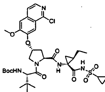
Compound 300
