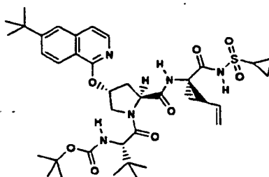
Compound 191
