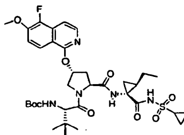
Compound 299
