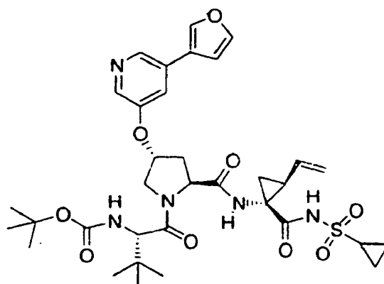
Compound 424
