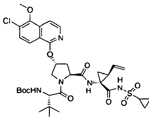
Compound 276
