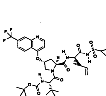
Compound 185
