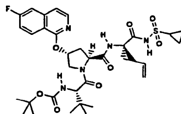
Compound 187
