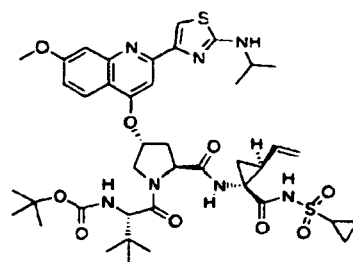
Compound 370
