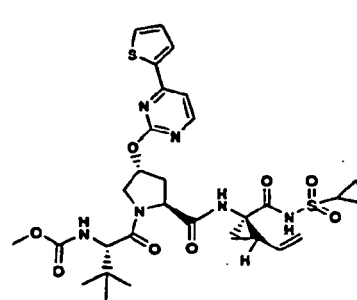
Compound 337
