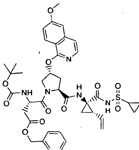
Compound 137
