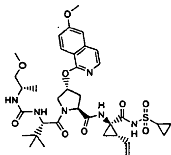
Compound 153
