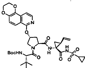
Compound 286
