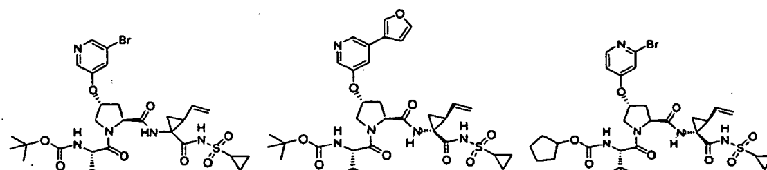
Compound 423
