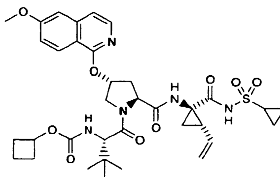
Compound 71
