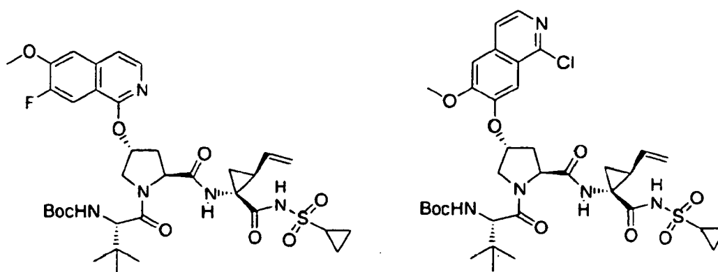
Compound 262
