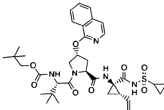
Compound 125
