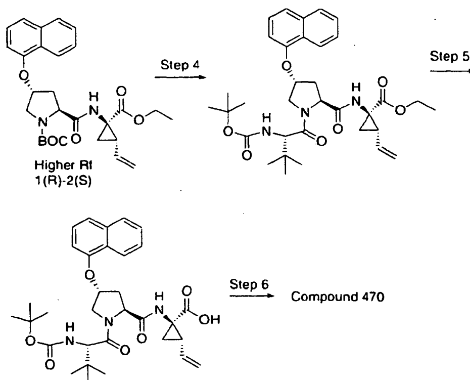
Scheme 2
