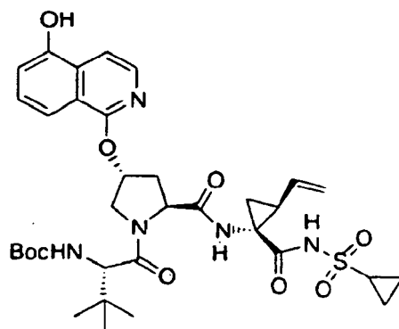
Compound 256
