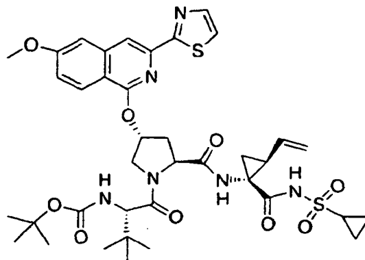
Compound 37
