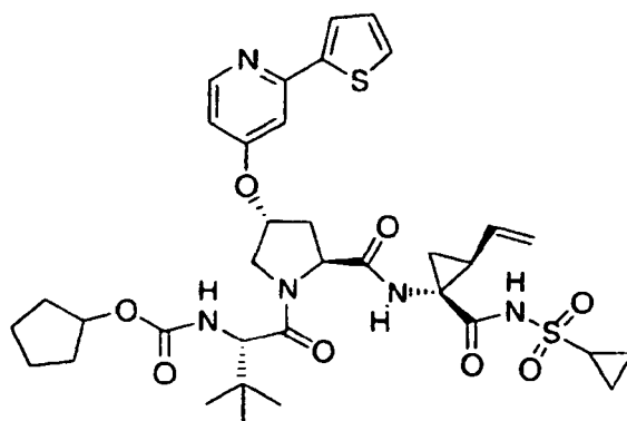
Compound 429
