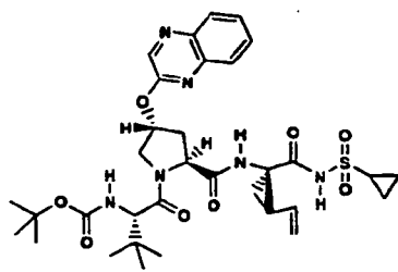
Compound 237
