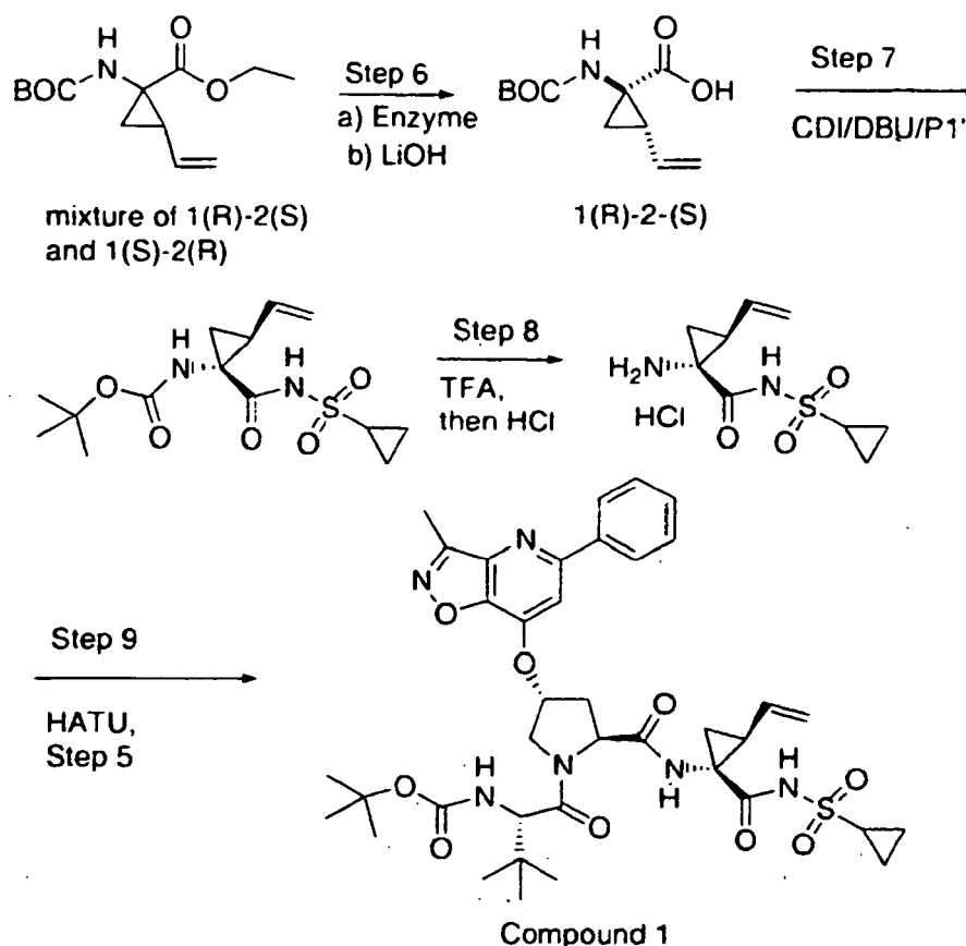
Scheme 3
