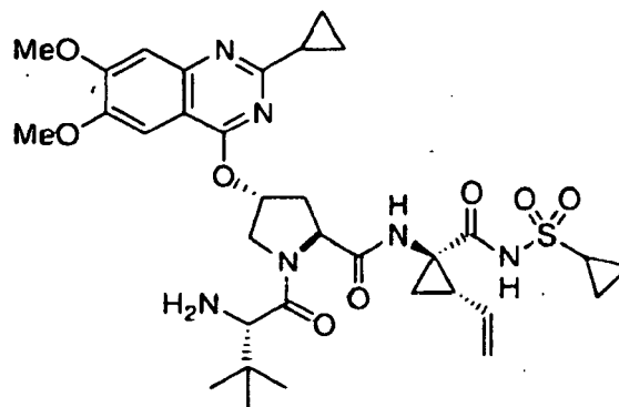
Compound 49
