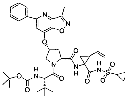
Compound 10
