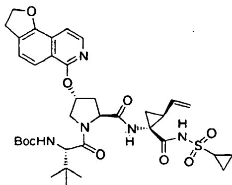
Compound 265
