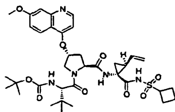
Compound 374
