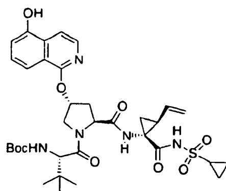
Compound 256
