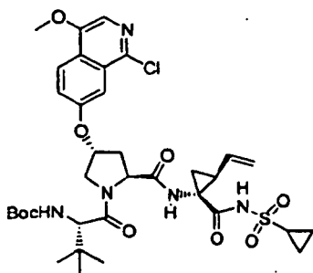
Compound 283
