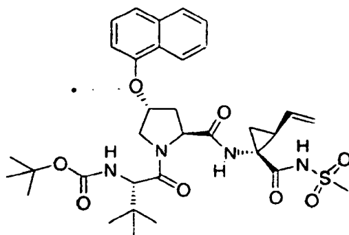
Compound 470
