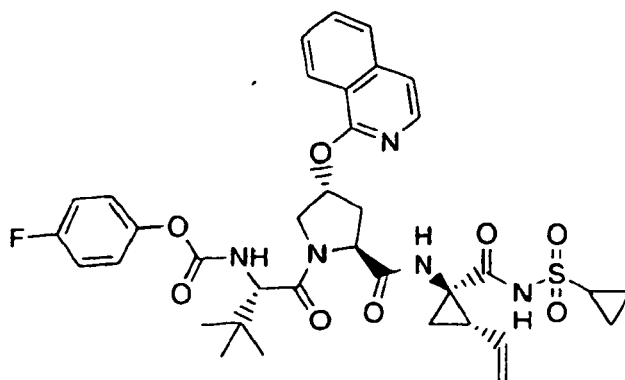
Compound 122
