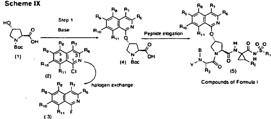
Scheme IX
