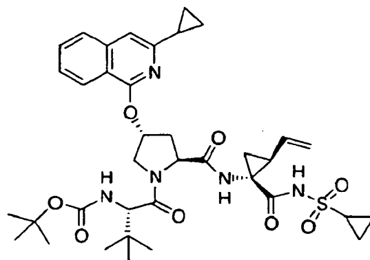
Compound 34
