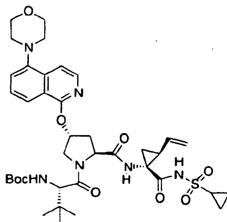
Compound 271
