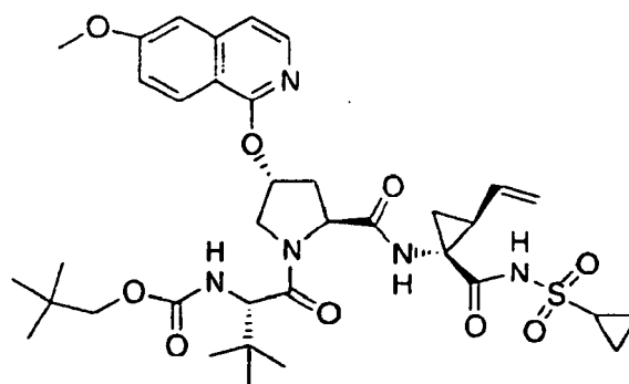
Compound 18
