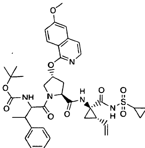
Compound 136
