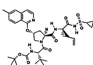
Compound 210
