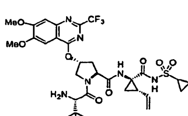
Compound 52
