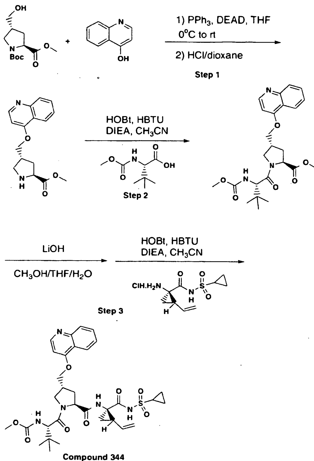
Scheme 2:
