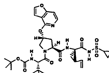
Compound 233
