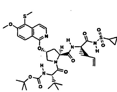
Compound 207
