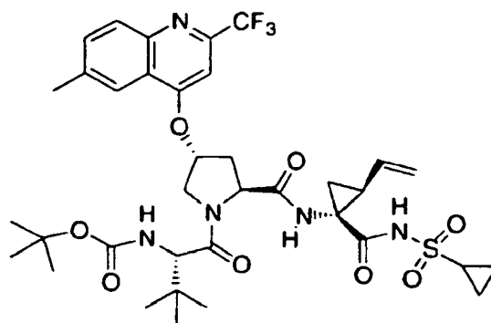
Compound 410
