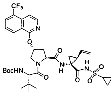
Compound 270
