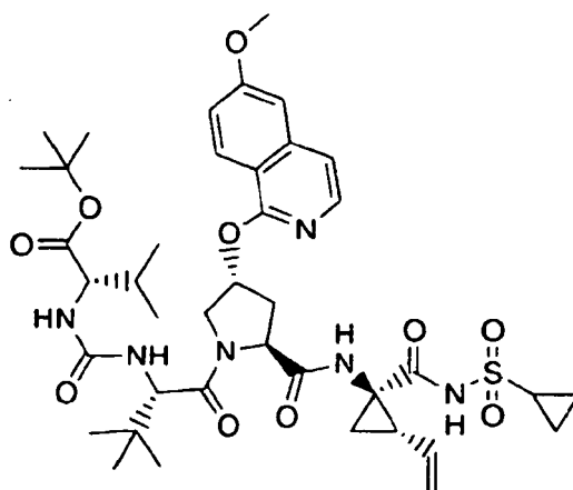
Compound 152
