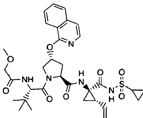
Compound 131
