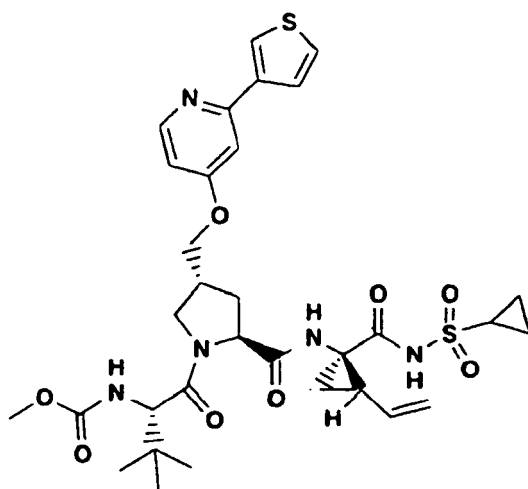
Compound 349
