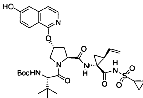
Compound 280
