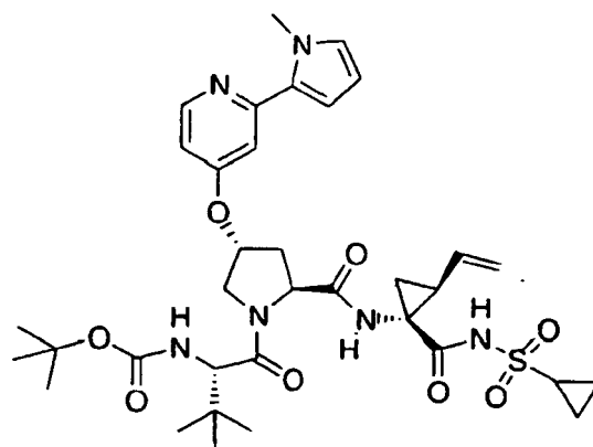
Compound 434
