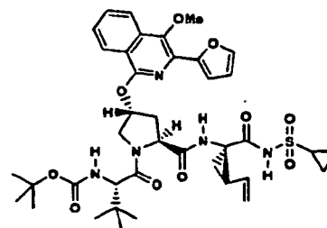
Compound 230
