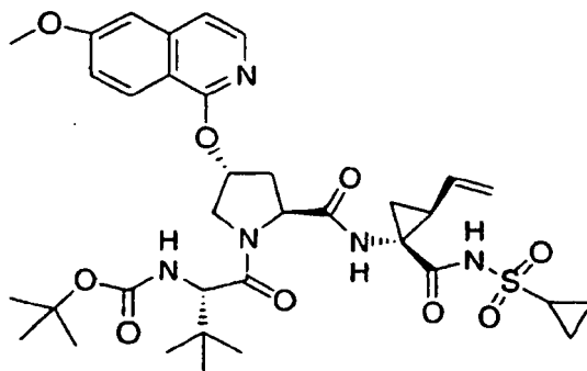
Compound 11
