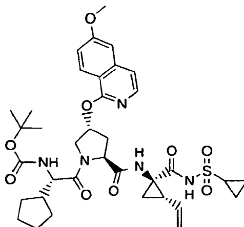
Compound 149
