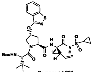
Compound 324
