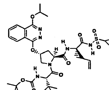
Compound 199
