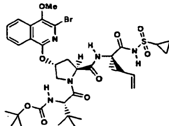
Compound 223
