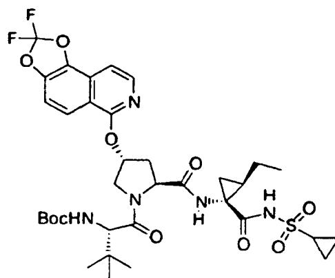
Compound 289
