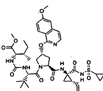
Compound 151
