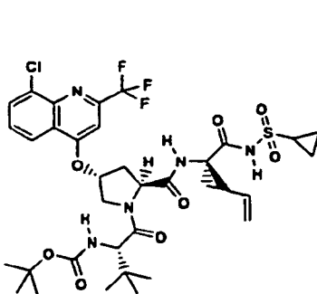
Compound 183
