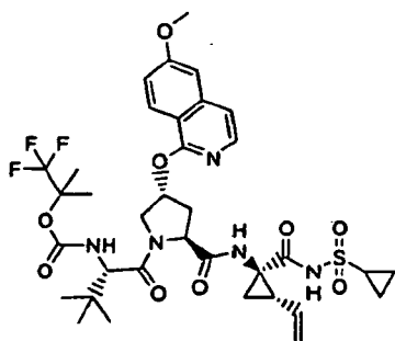
Compound 155
