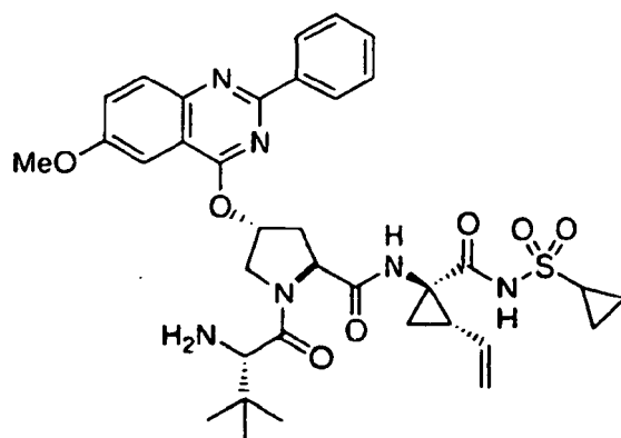
Compound 50
