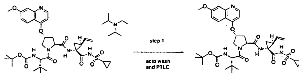
Compound 375
