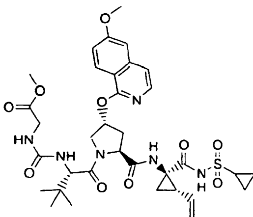
Compound 144
