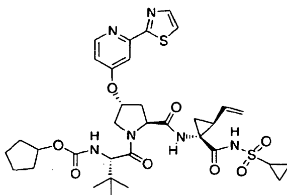
Compound 431
