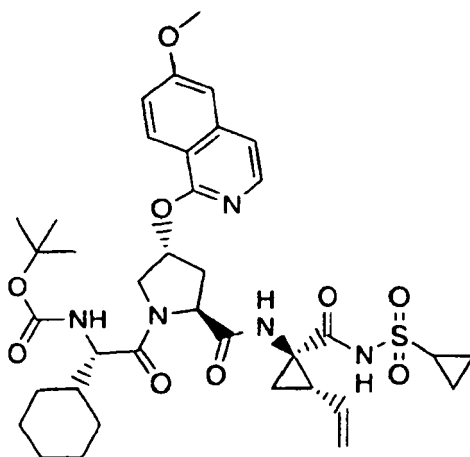
Compound 143
