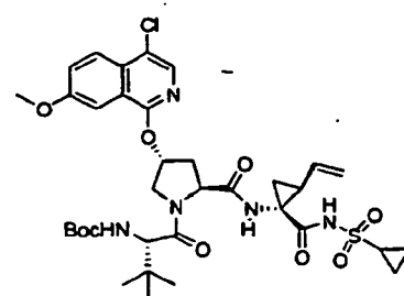
Compound 284
