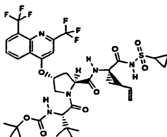
Compound 181
