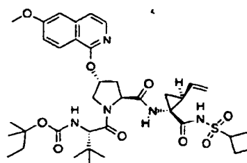
Compound 382
