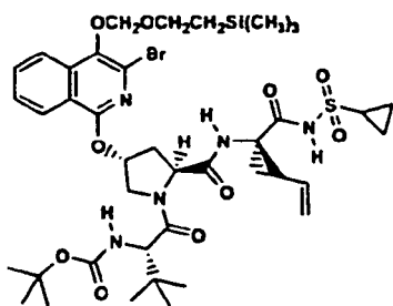
Compound 225
