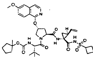
Compound 384
