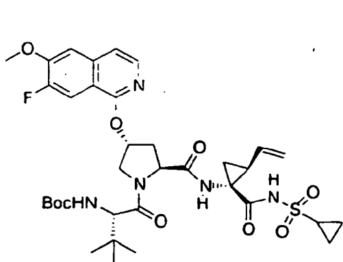
Compound 261
