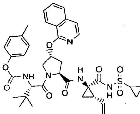
Compound 120
