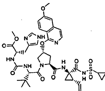
Compound 147
