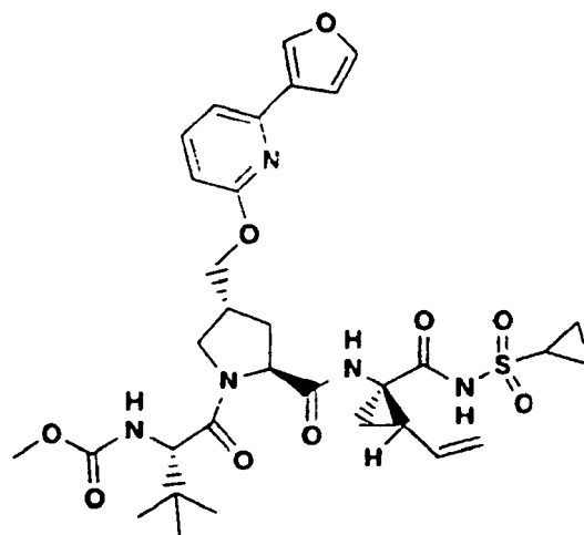
Compound 355
