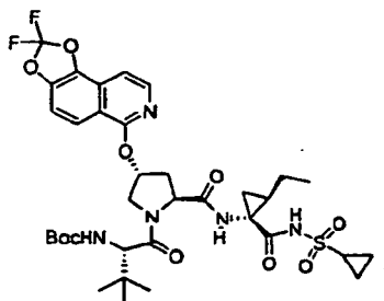
Compound 289
