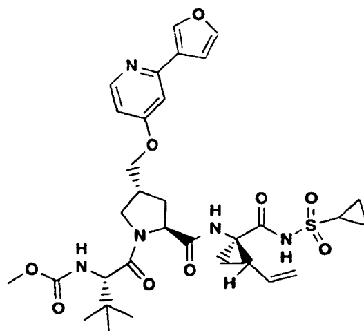
Compound 351
