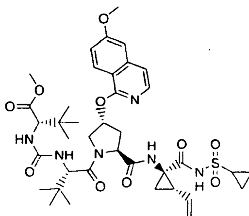
Compound 146
