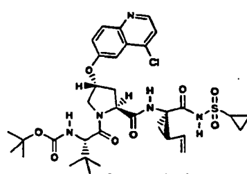
Compound 240
