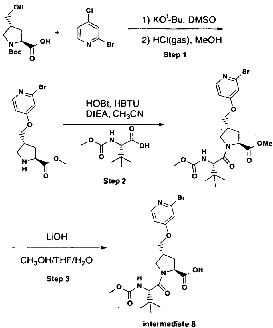
Scheme 2:
