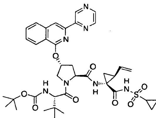
Compound 31
