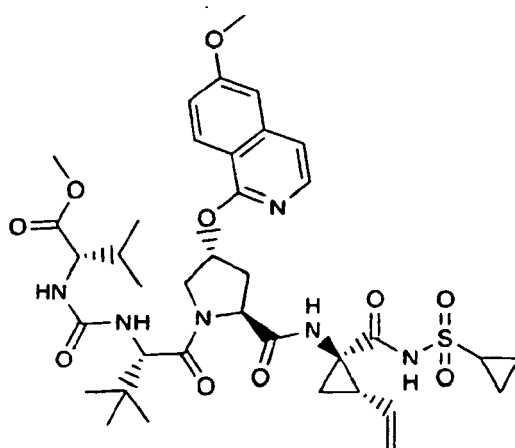
Compound 141
