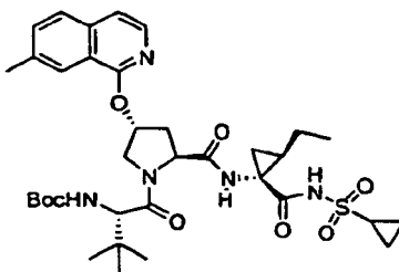
Compound 296
