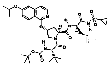
Compound 192
