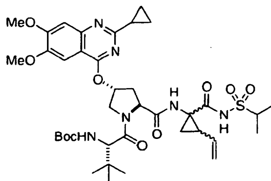
Compound 46
