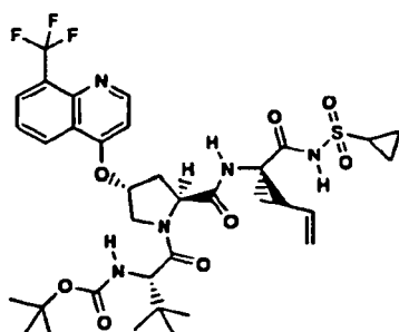
Compound 186
