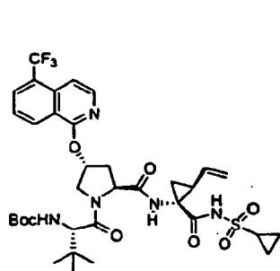
Compound 270
