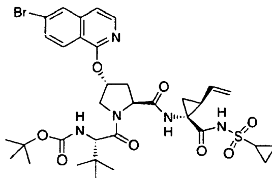
Compound 22
