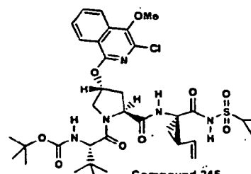
Compound 245
