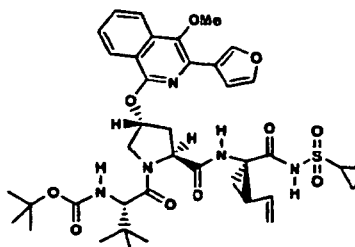
Compound 229
