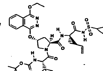
Compound 200
