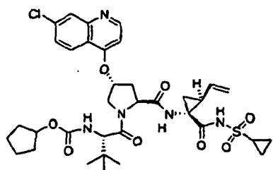
Compound 372
