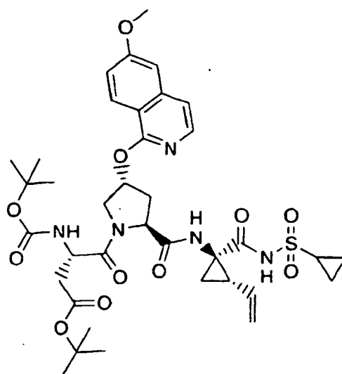
Compound 139
