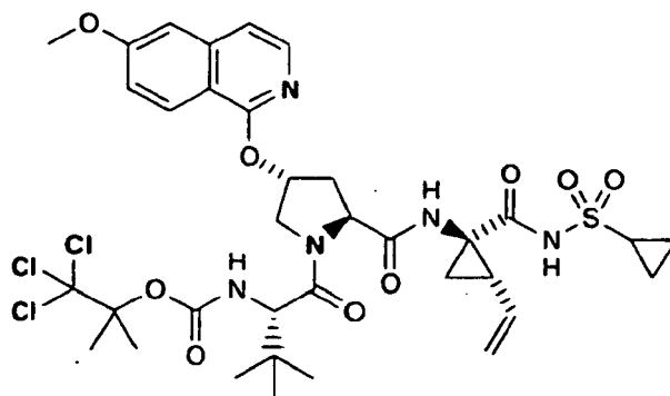
Compound 68
