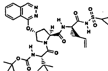
Compound 184
