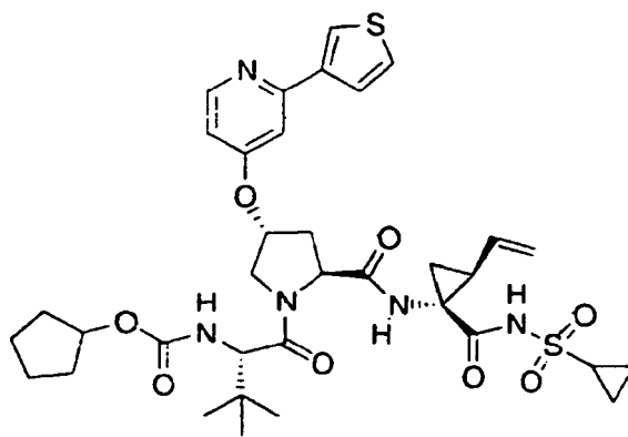
Compound 430
