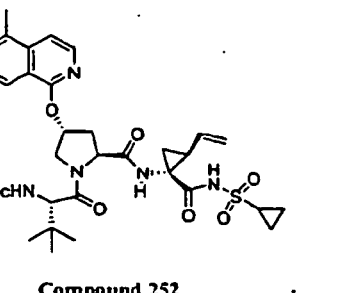
Compound 252
