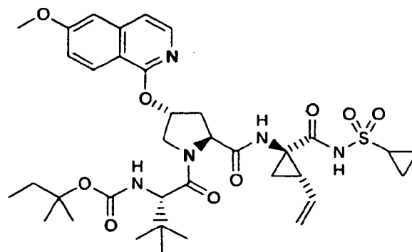
Compound 67
