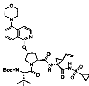
Compound 271
