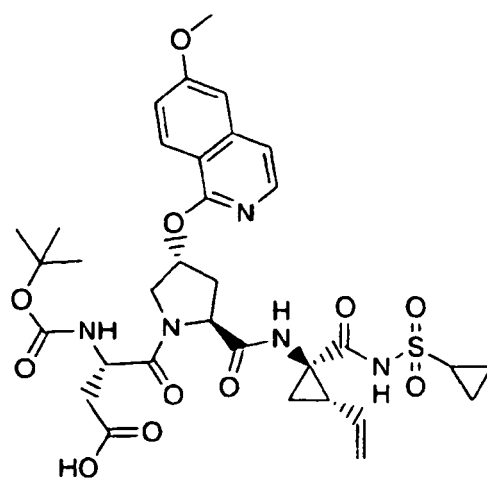
Compound 140
