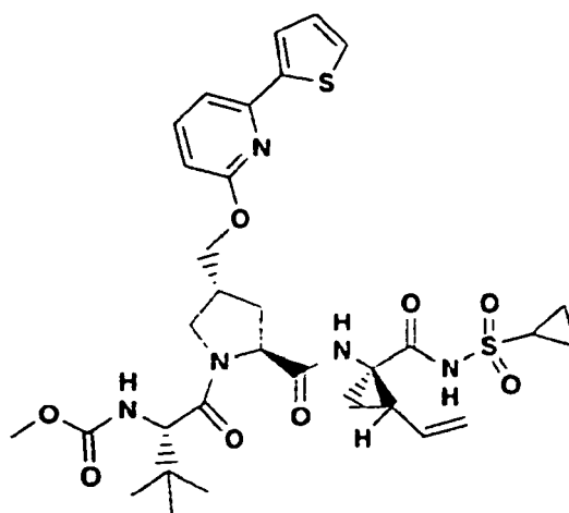
Compound 356
