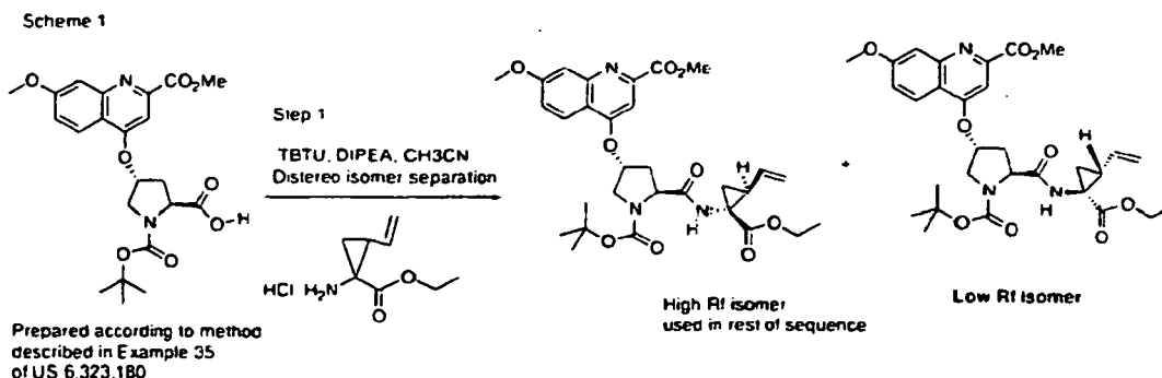
Compound 370
