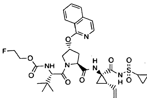
Compound 126
