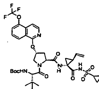
Compound 269
