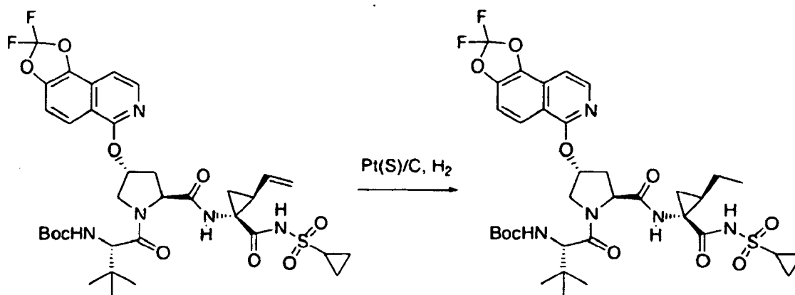
Compound 287
