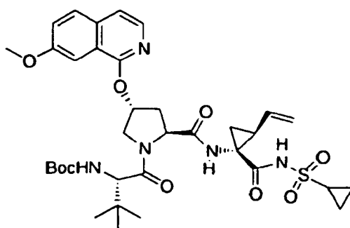
Compound 260
