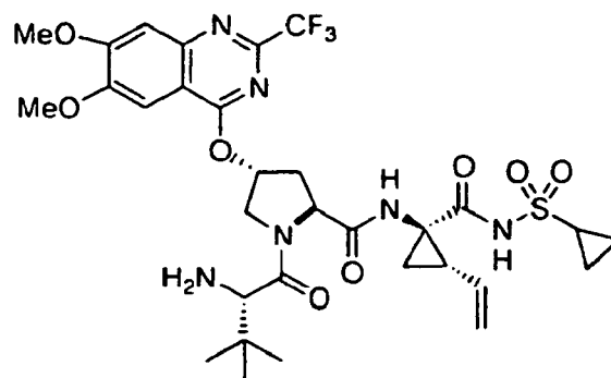
Compound 52
