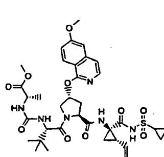
Compound 145
