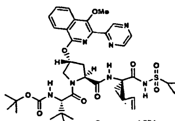
Compound 231
