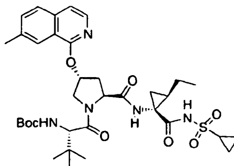
Compound 296
