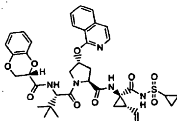
Compound 133
