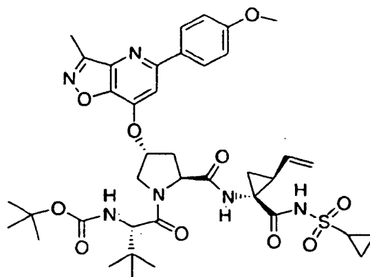
Compound 3
