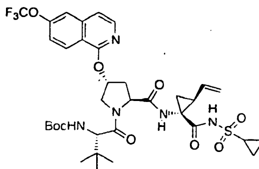
Compound 282
