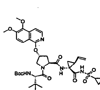
Compound 272
