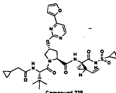
Compound 339
