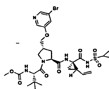
Compound 346
