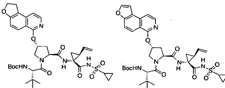
Compound 267
