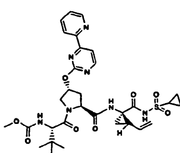
Compound 336
