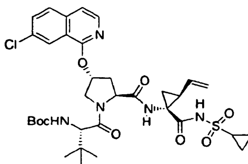
Compound 258
