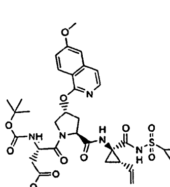
Compound 138
