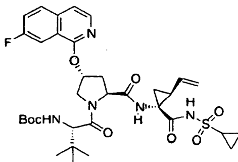
Compound 257
