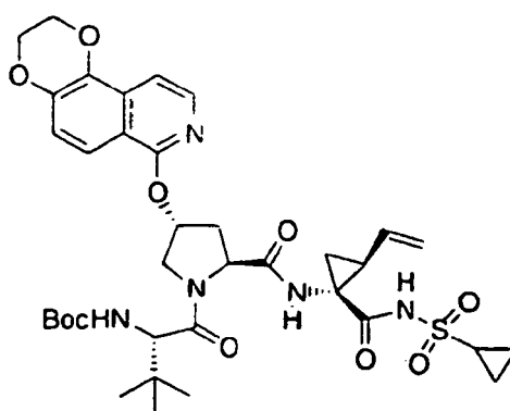
Compound 286
