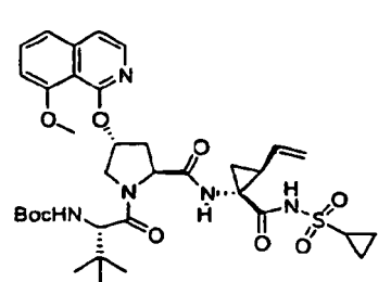
Compound 264
