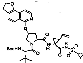
Compound 265
