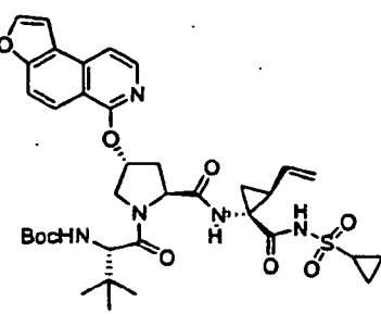
Compound 268
