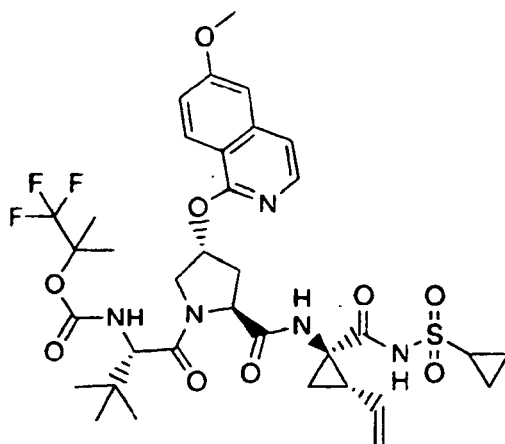
Compound 155
