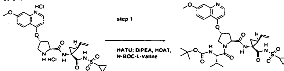
compound 378
