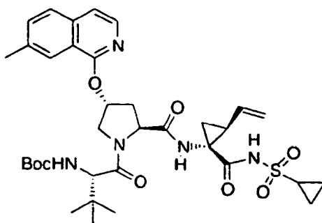
Compound 259
