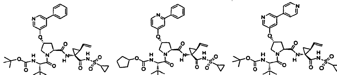
Compound 420
