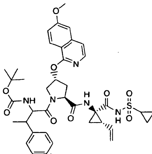
Compound 135
