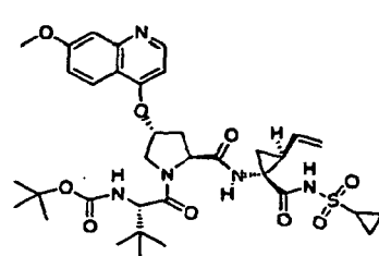
Compound 376
