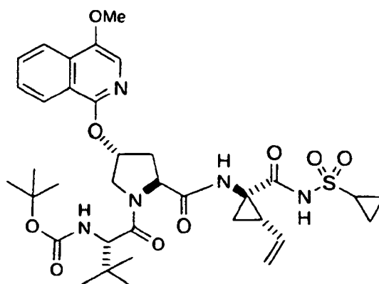
Compound 251
