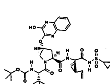
Compound 243
