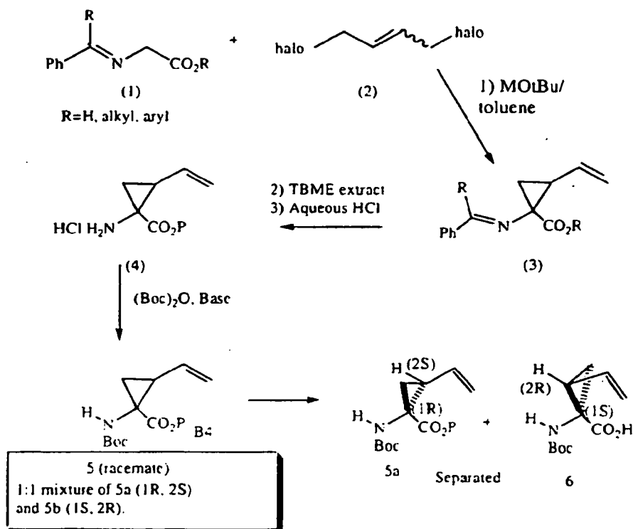
Scheme VIII
