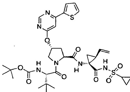
Compound 412
