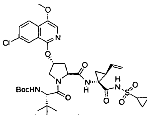
Compound 277
