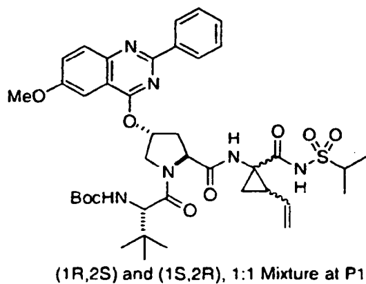
Compound 45
