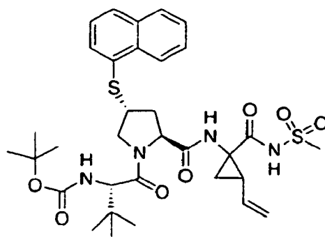
Compound 451
