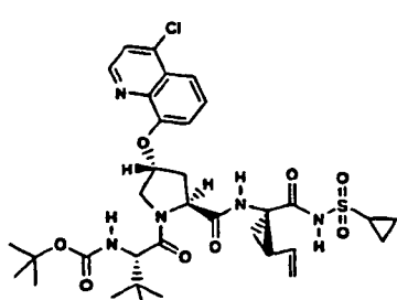
Compound 242
