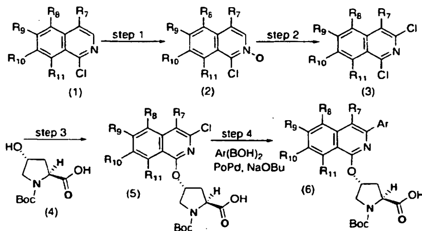
Scheme XVIII
