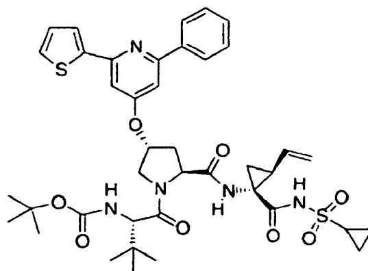
Compound 413
