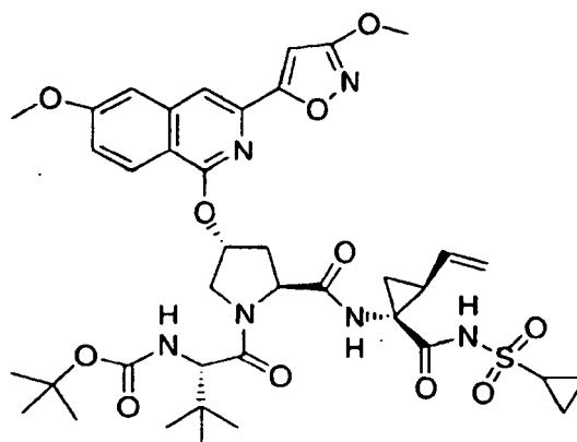
Compound 38
