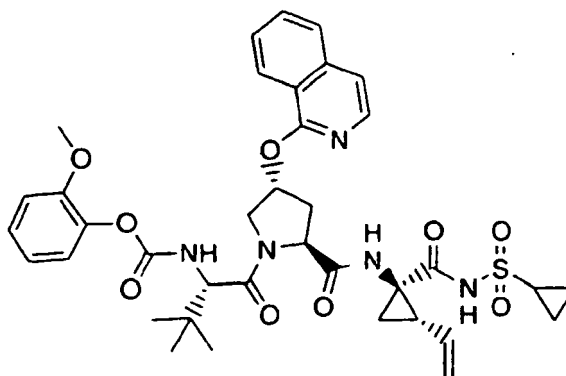
Compound 127
