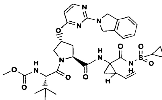
Compound 342
