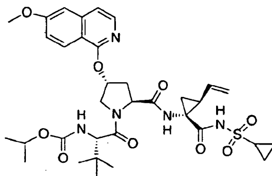
Compound 17
