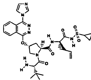
Compound 197
