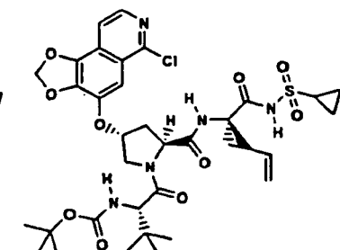
Compound 212
