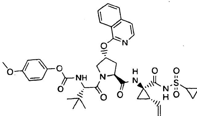
Compound 123
