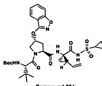
Compound 334
