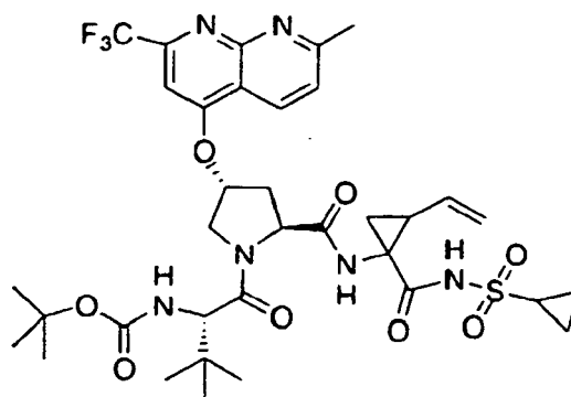
Compound 8
