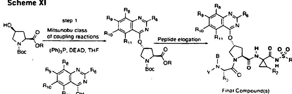
Scheme XI
