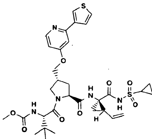
Compound 349
