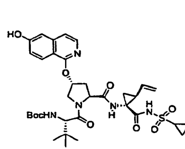
Compound 280
