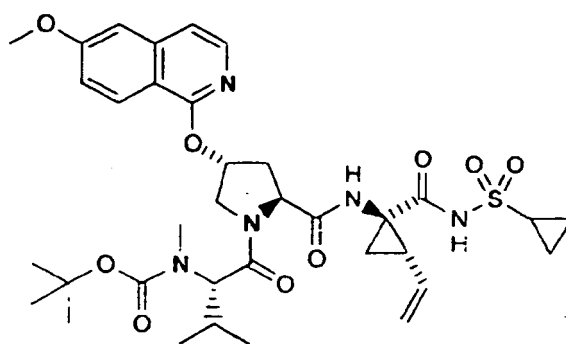
Compound 85
