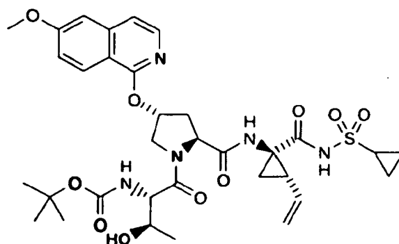
Compound 91
