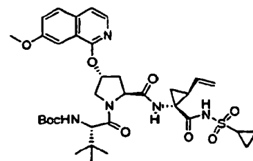
Compound 260
