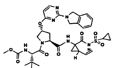
Compound 342
