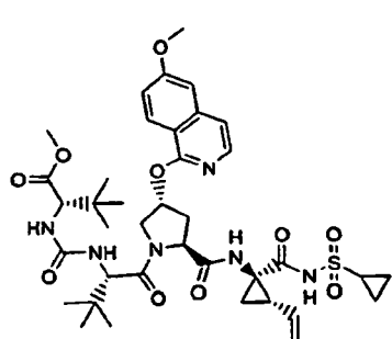
Compound 146
