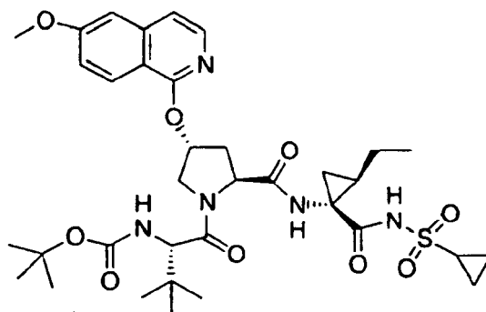
Compound 14
