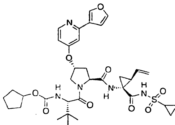
Compound 426
