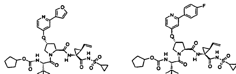
Compound 426
