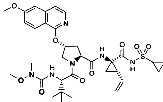
Compound 78
