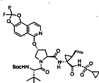
Compound 287
