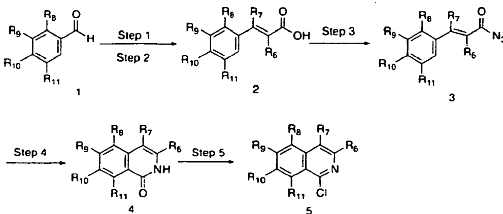
Scheme XII
