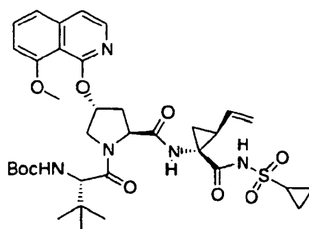
Compound 264
