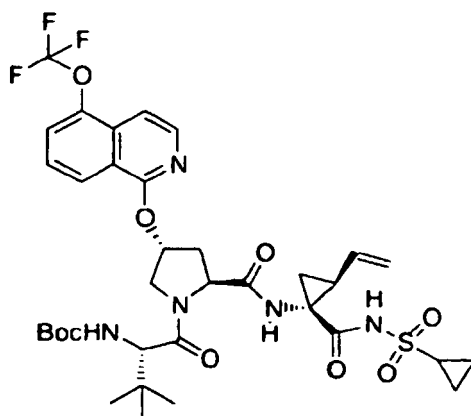
Compound 269
