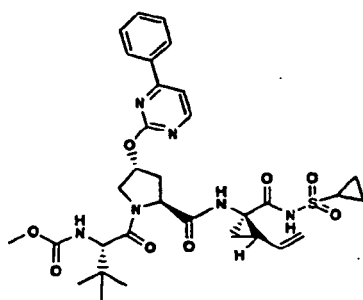
Compound 335
