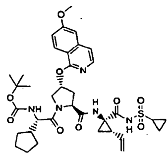
Compound 149
