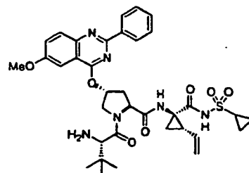
Compound 50
