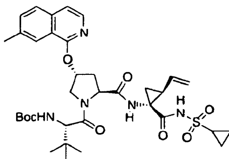
Compound 259
