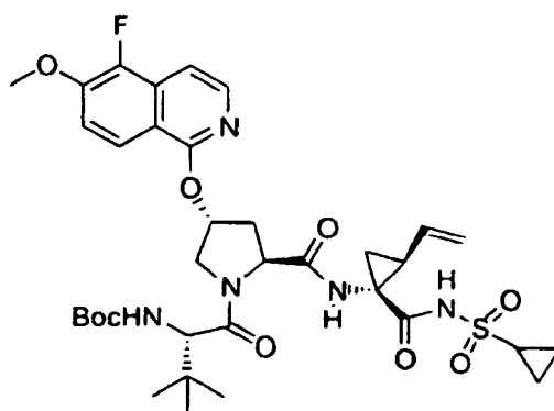
Compound 274
