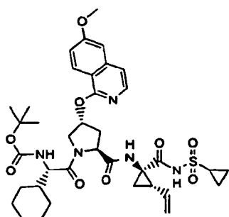
Compound 143
