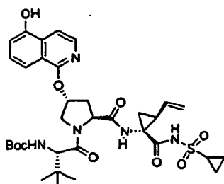
Compound 256
