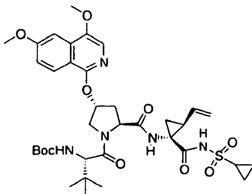
Compound 279
