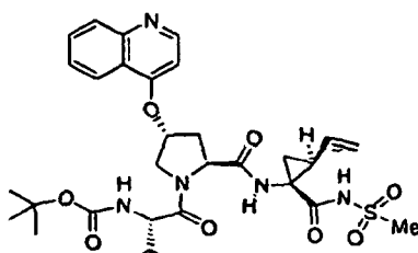
Compound 386
