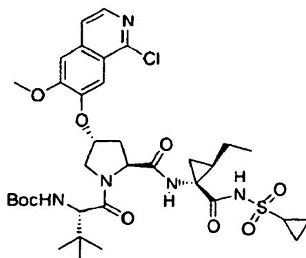
Compound 300
