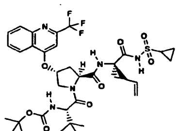
Compound 180
