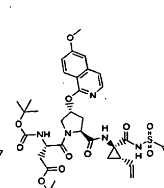
Compound 139
