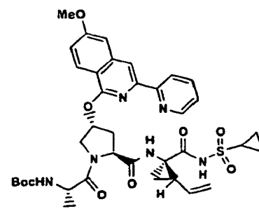
Compound 320
