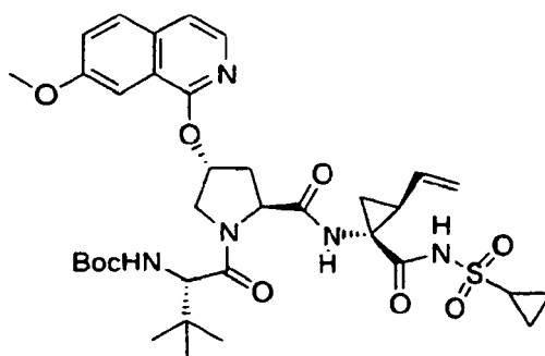
Compound 260
