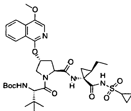
Compound 291
