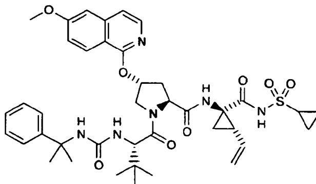
Compound 83
