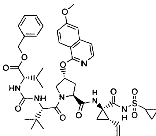
Compound 150
