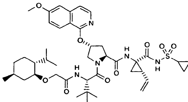
Compound 60
