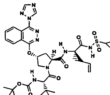
Compound 198
