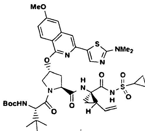
Compound 331
