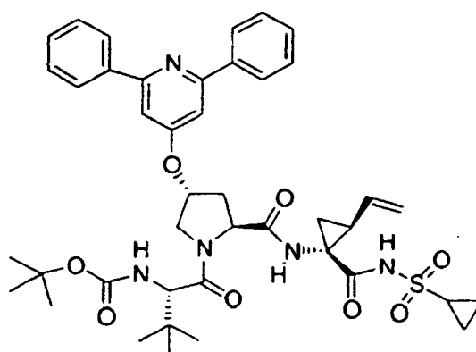
Compound 415
