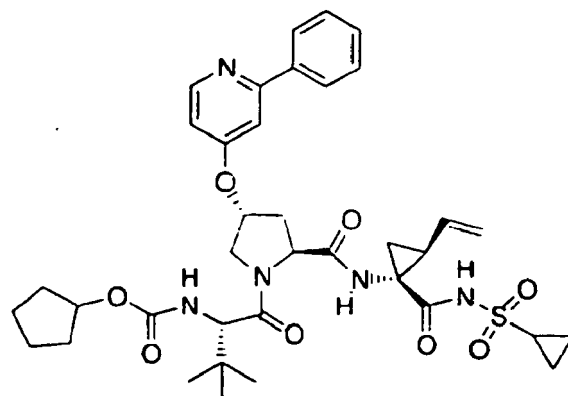
Compound 421
