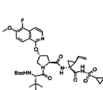
Compound 274
