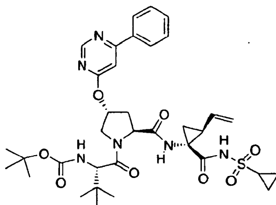
Compound 411
