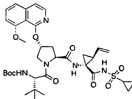
Compound 264
