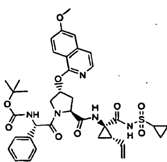
Compound 134
