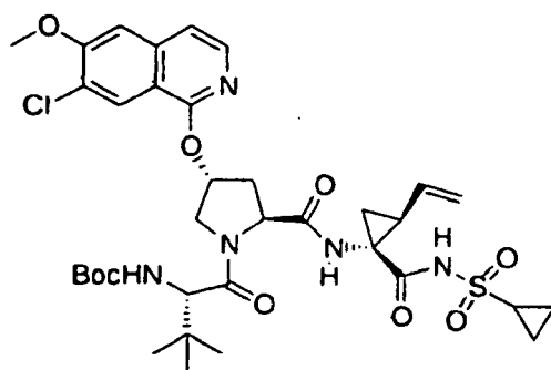
Compound 273
