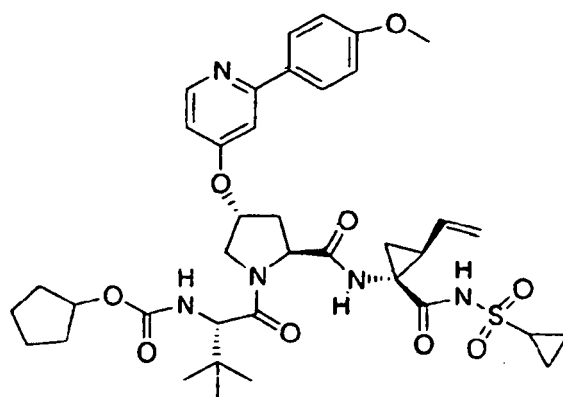
Compound 428
