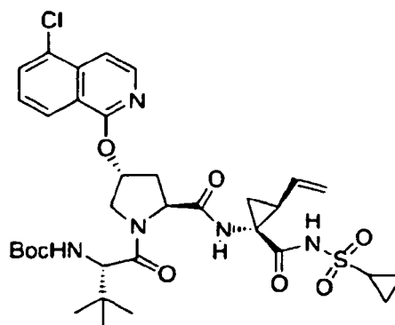
Compound 254
