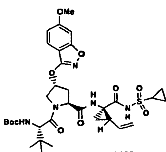
Compound 323
