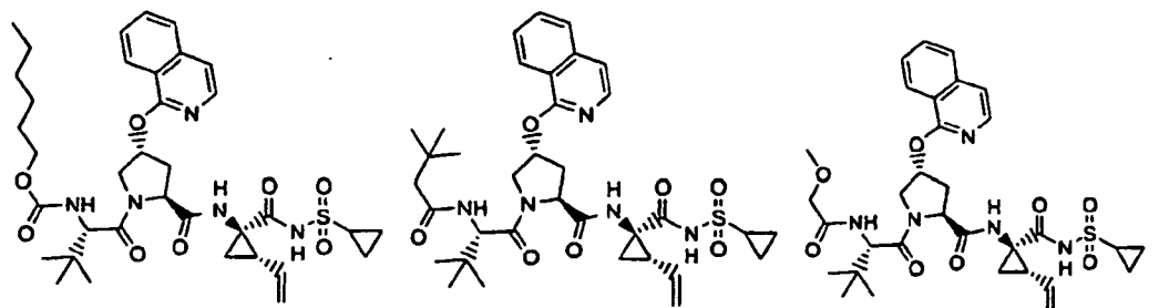
Compound 129
