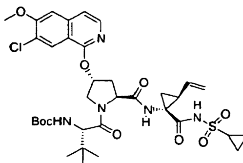
Compound 273
