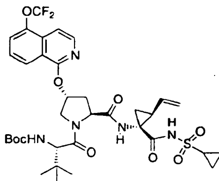
Compound 285
