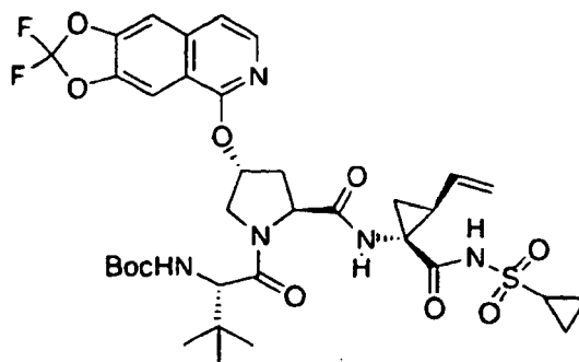
Compound 288
