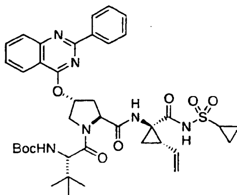
Compound 47
