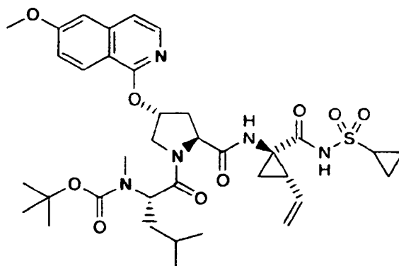
Compound 86
