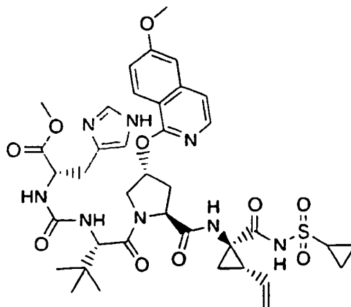
Compound 147
