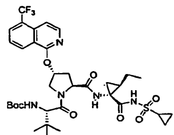
Compound 295
