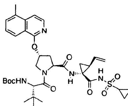
Compound 252
