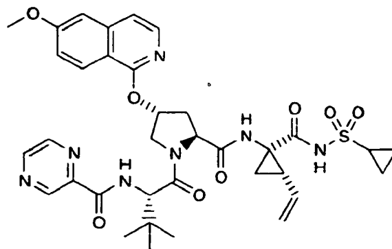
Compound 63
