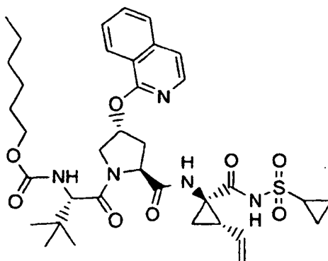
Compound 129
