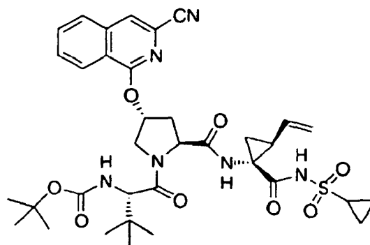
Compound 32
