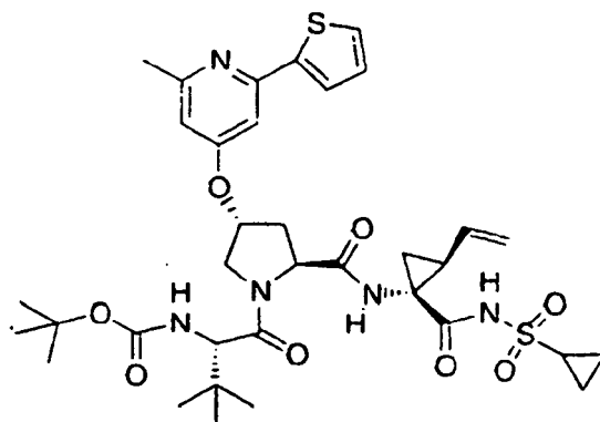
Compound 438
