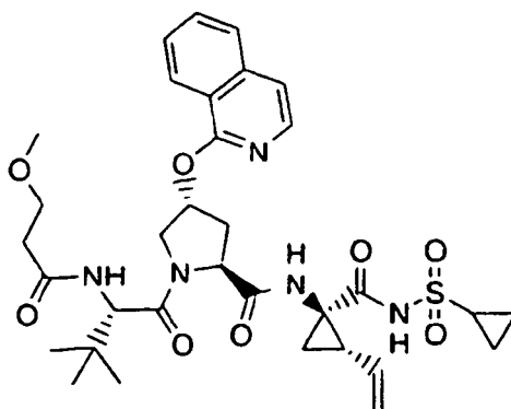
Compound 132
