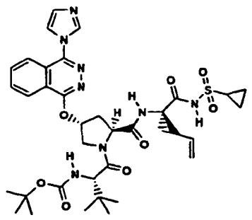
Compound 196
