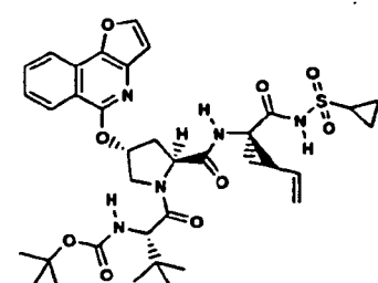
Compound 220
