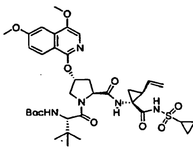
Compound 279
