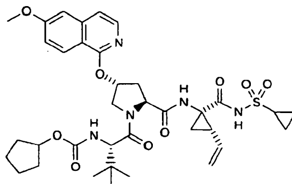
Compound 70
