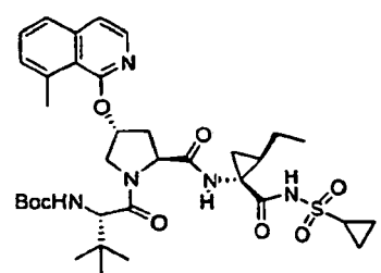
Compound 297
