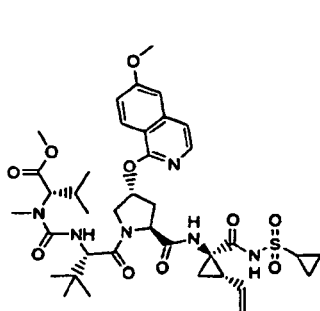
Compound 154
