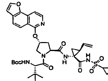
Compound 266
