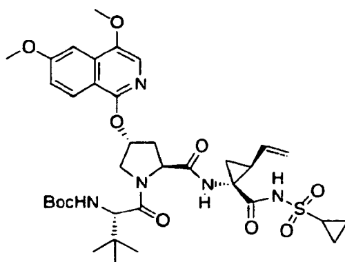
Compound 279
