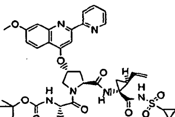
Compound 379
