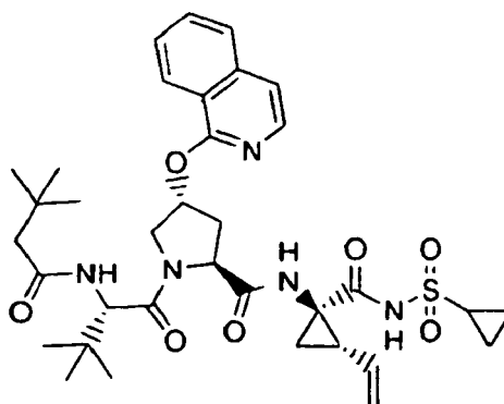
Compound 130
