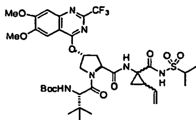
Compound 51
