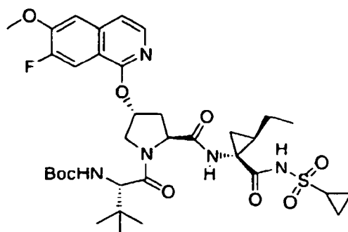
Compound 298
