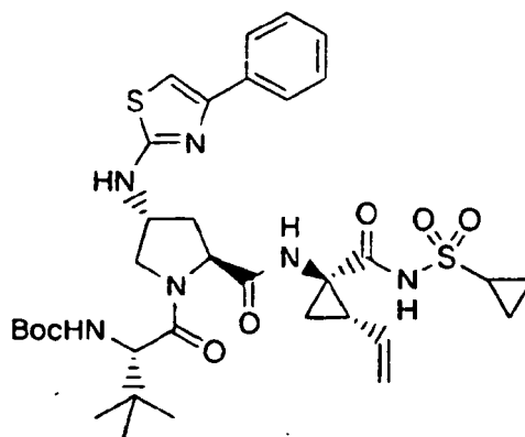
Compound 53
