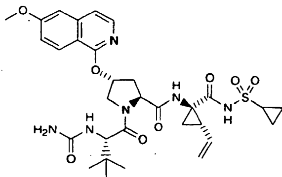
Compound 80
