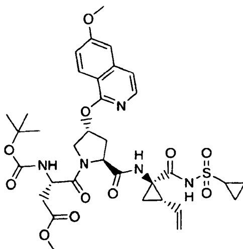
Compound 138
