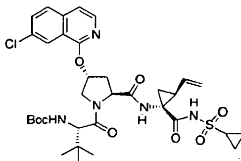
Compound 258
