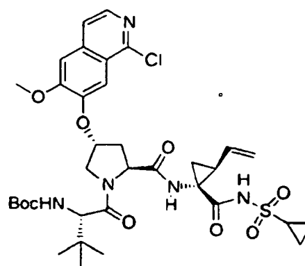
Compound 262
