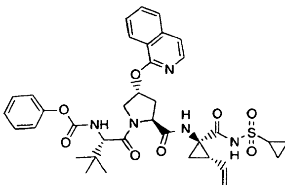
Compound 121
