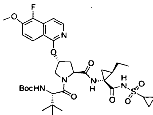
Compound 299
