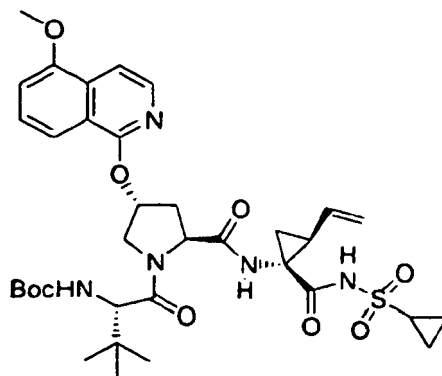
Compound 253
