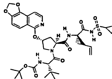
Compound 211
