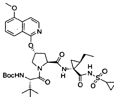
Compound 292
