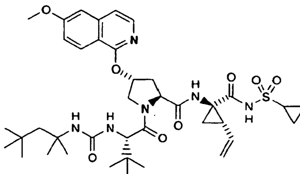
Compound 81
