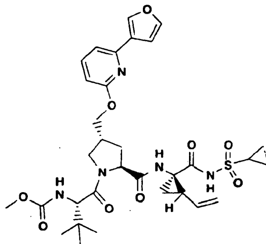
Compound 355
