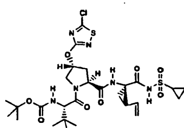
Compound 236
