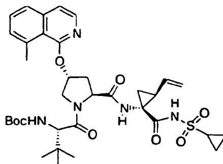
Compound 263
