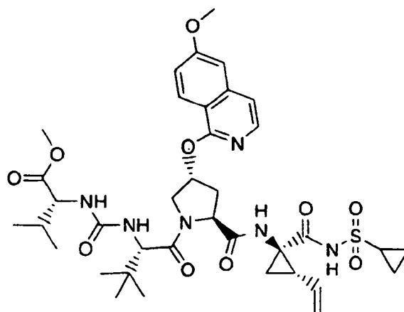
Compound 142
