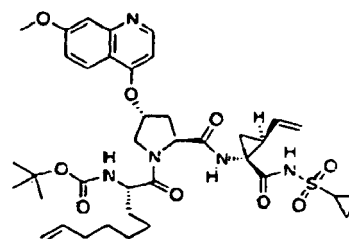
compound 377
