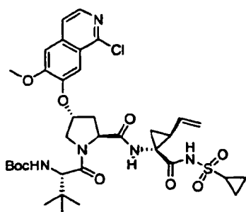
Compound 262
