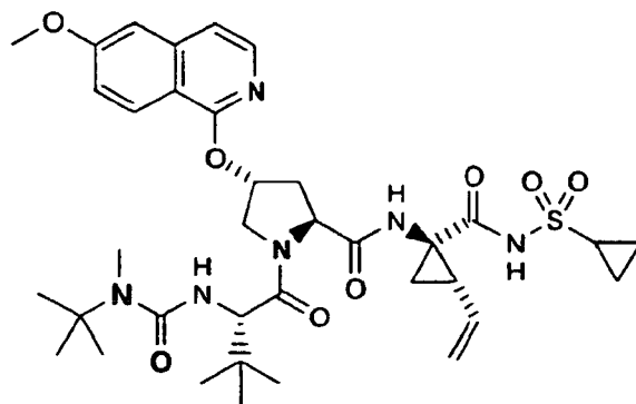
Compound 77
