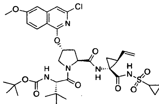
Compound 40
