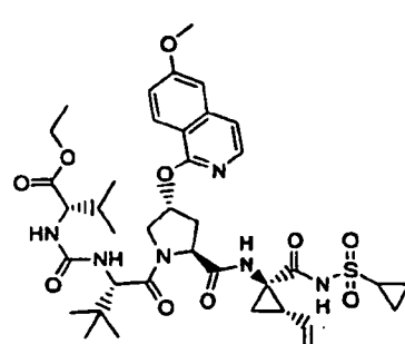
Compound 148
