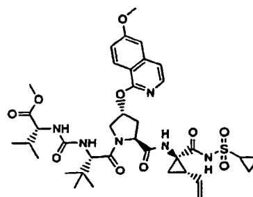
Compound 142
