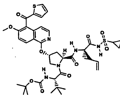
Compound 209
