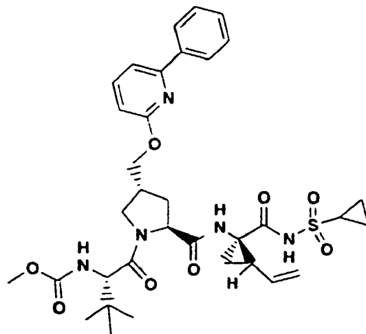
Compound 354
