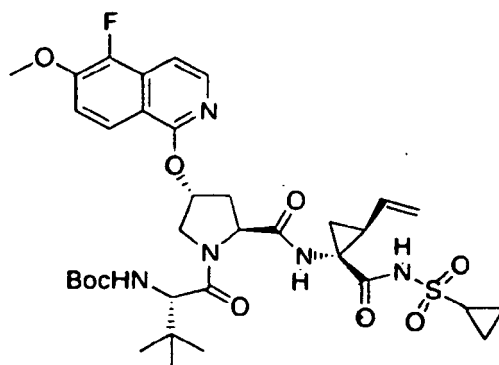
Compound 274
