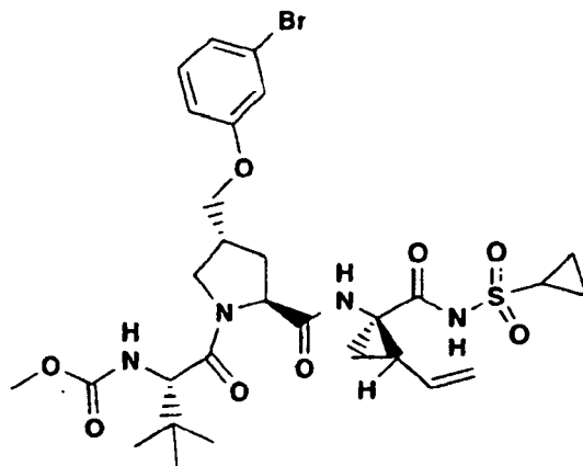
Compound 345
