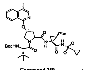
Compound 250
