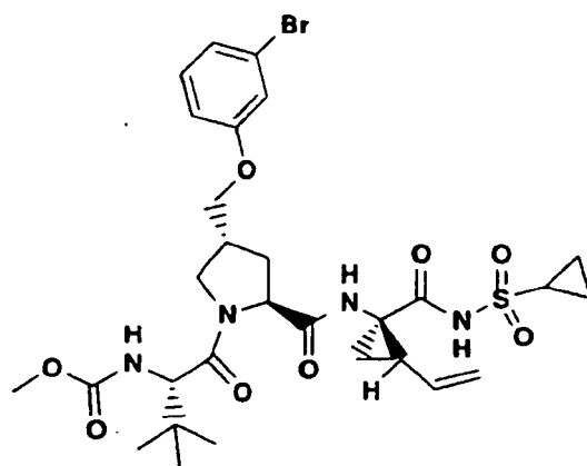
Compound 345
