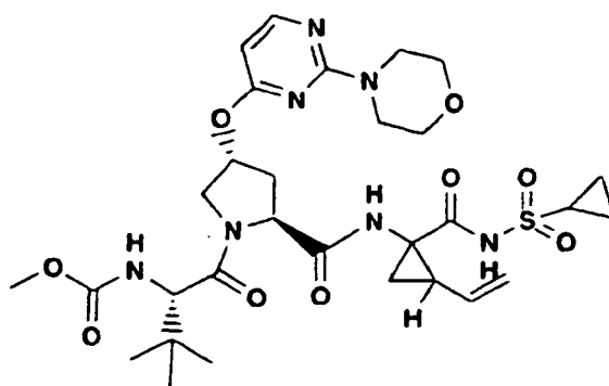
Compound 343
