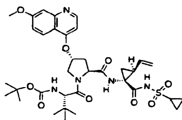
Compound 376
