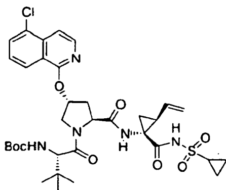
Compound 254
