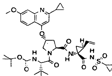
Compound 373
