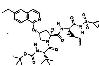
Compound 189
