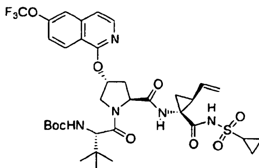
Compound 282
