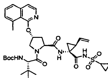
Compound 263
