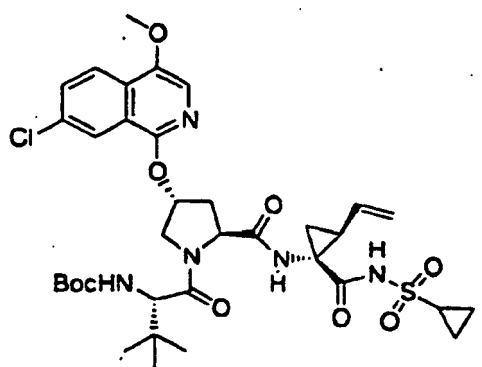
Compound 277
