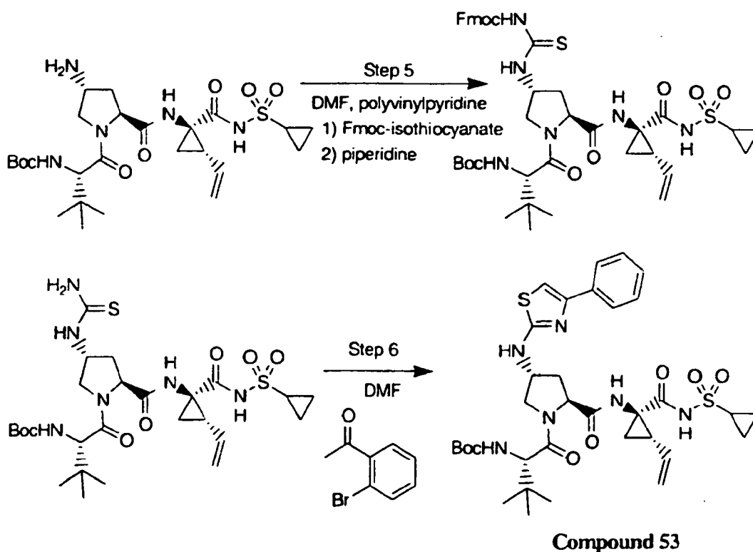
Scheme 3
