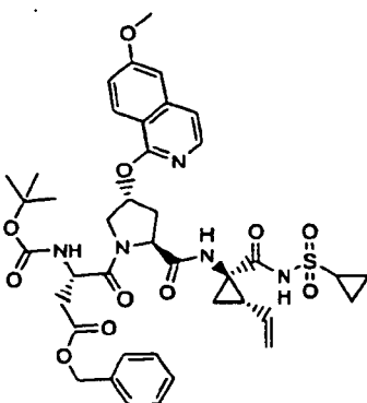
Compound 137
