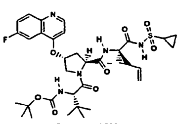
Compound 239
