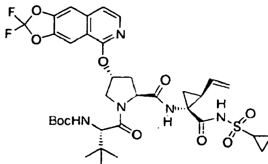
Compound 288
