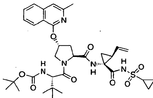
Compound 33
