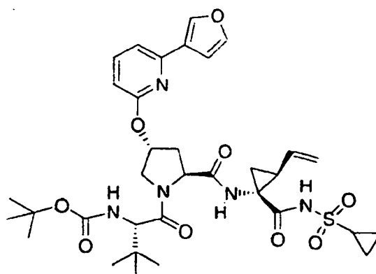
Compound 435
