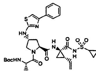
Compound 53
