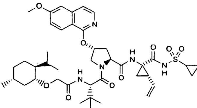
Compound 61
