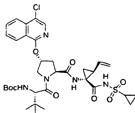
Compound 281
