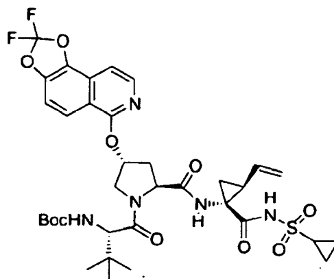
Compound 287
