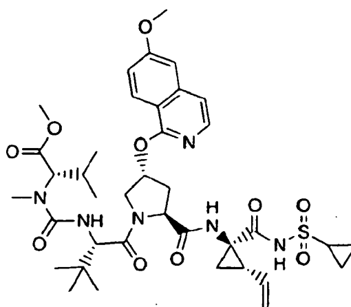
Compound 154
