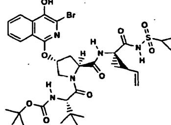
Compound 224
