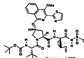
Compound 232
