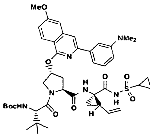
Compound 330
