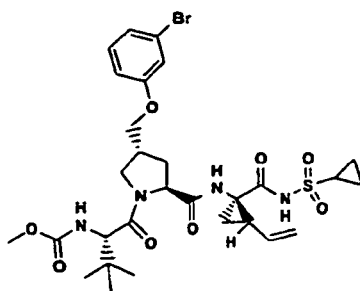
Compound 345
