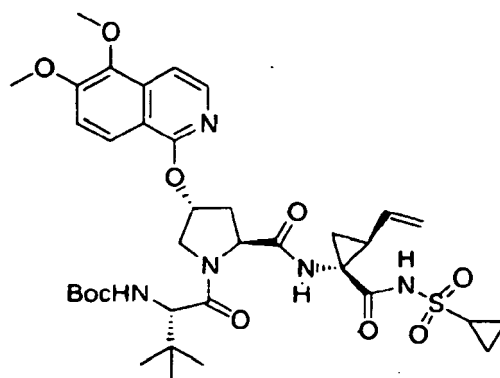
Compound 272
