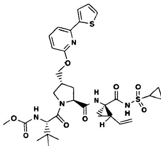
Compound 356
