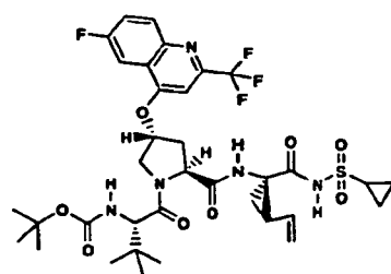
Compound 238
