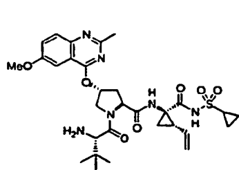
Compound 48
