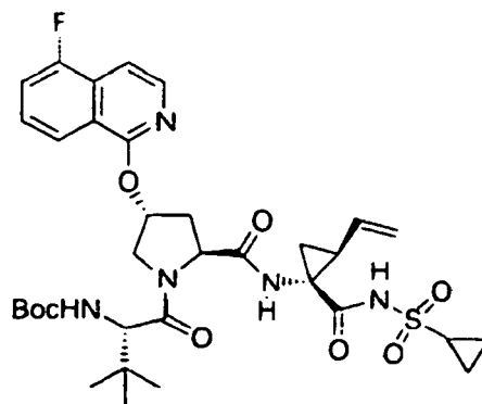
Compound 255
