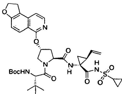
Compound 267
