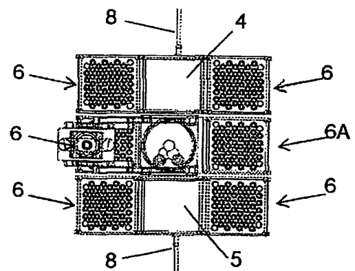
Fig. 4 Plan view
