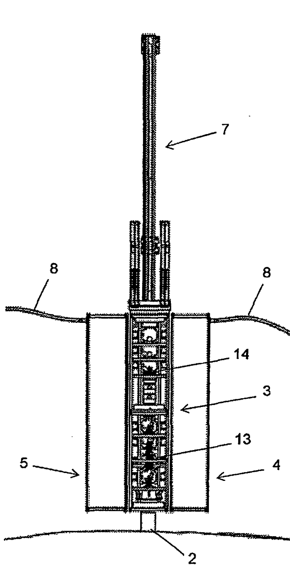
Fig. 2 Front elevation with pipe unit 6A removed
