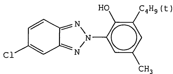
Ultraviolet Absorbent (UV-1):
