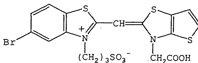
Sensitizing Dye S-1:
