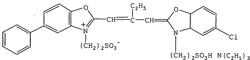
Sensitizing Dye S-5:
