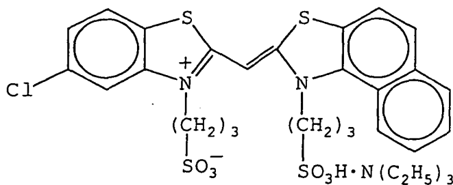
Sensitizing Dye S-3:
