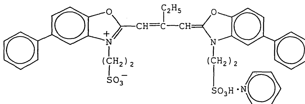
Sensitizing Dye S-4:
