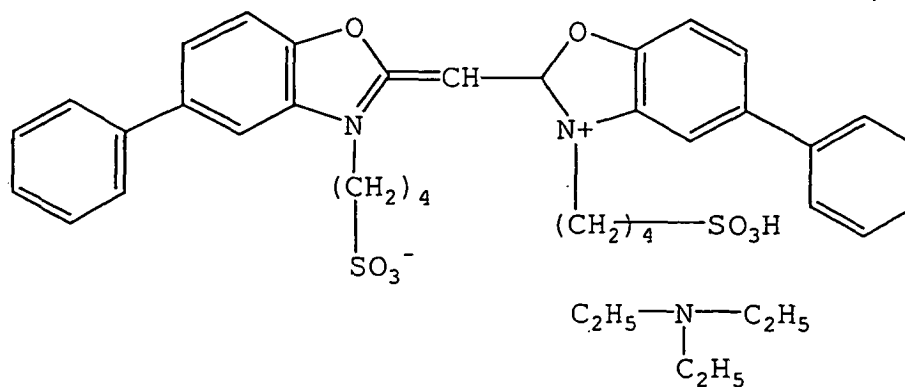
Sensitizing Dye S-6:
