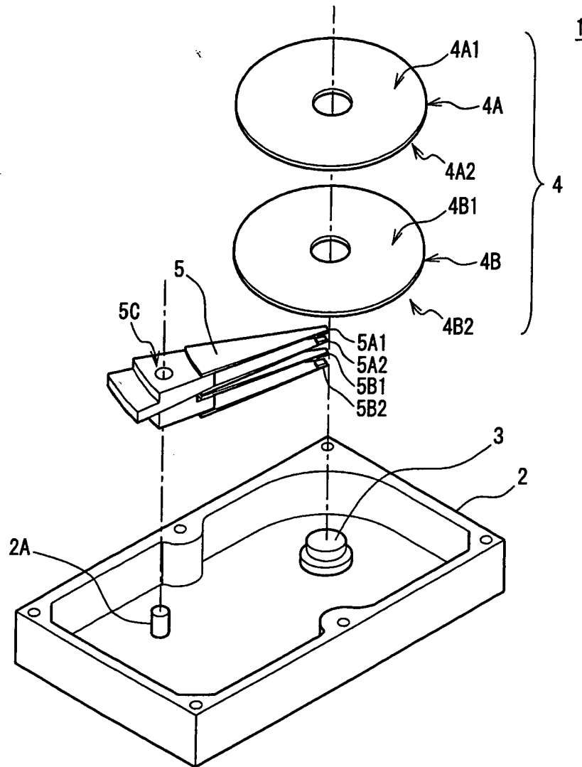
FIG. 1 (RELATED ART)
