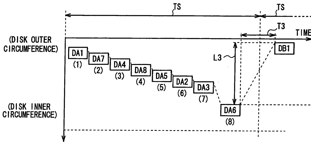
FIG. 6C (RELATED ART)
