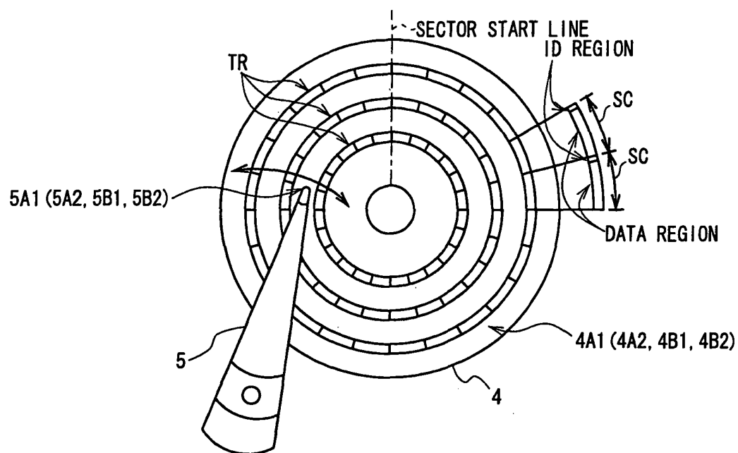
FIG. 2 (RELATED ART)
