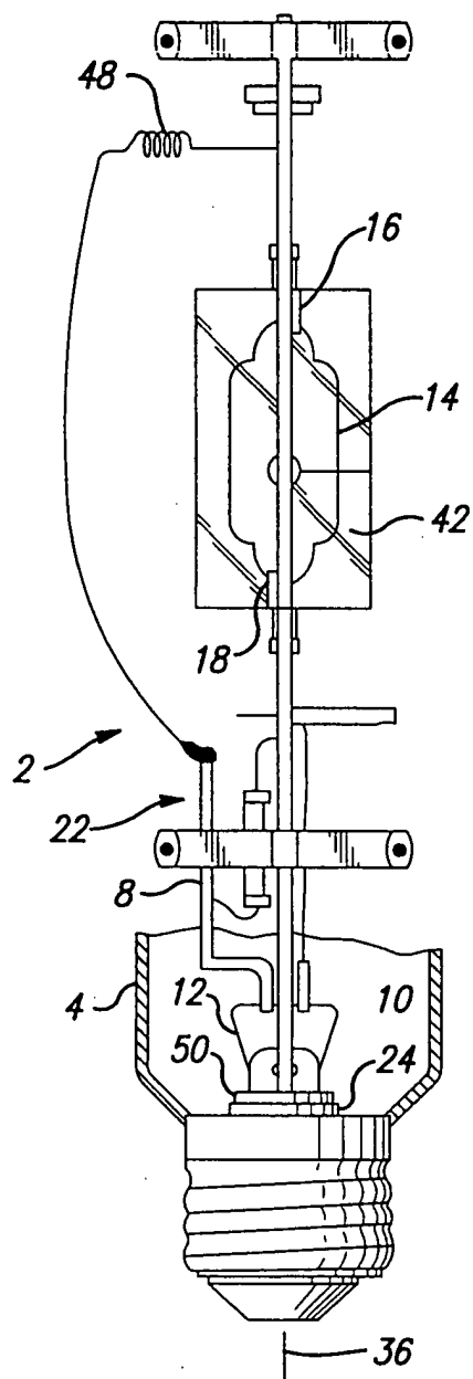
FIG. 1 PRIOR ART
