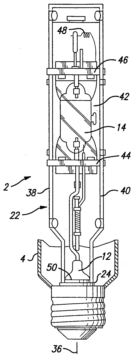
FIG. 2 PRIOR ART
